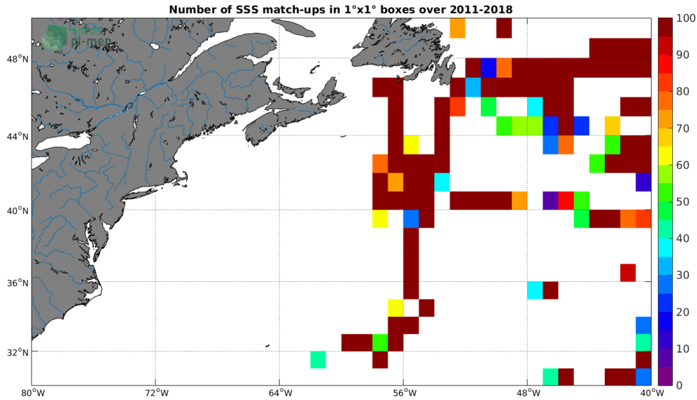
Figure 4: Number of SSS match-ups between TSG-GOSUD-Research-vessel SSS and the SMOS L2 v662 (ESA) SSS product for the Gulf Stream Pi-MEP region over 1^\circ \times 1^\circ boxes and for the full satellite product period.
