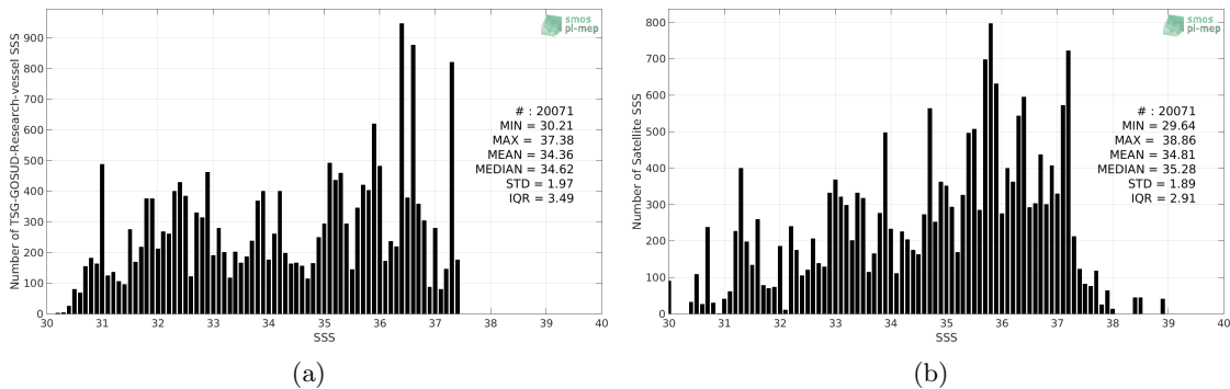
Figure 2: Histograms of SSS from TSG-GOSUD-Research-vessel (a) and SMOS L2 v662 (ESA) (b) considering all match-up pairs per bins of 0.1 over the Gulf Stream Pi-MEP region and for the full satellite product period.
