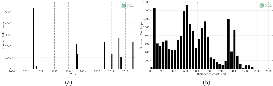
Figure 1: Number of match-ups between TSG-GOSUD-Research-vessel and SMOS L2 v662 (ESA) SSS as a function of time (a) and as function of the distance to coast (b) over the Gulf Stream Pi-MEP region and for the full satellite product period.
