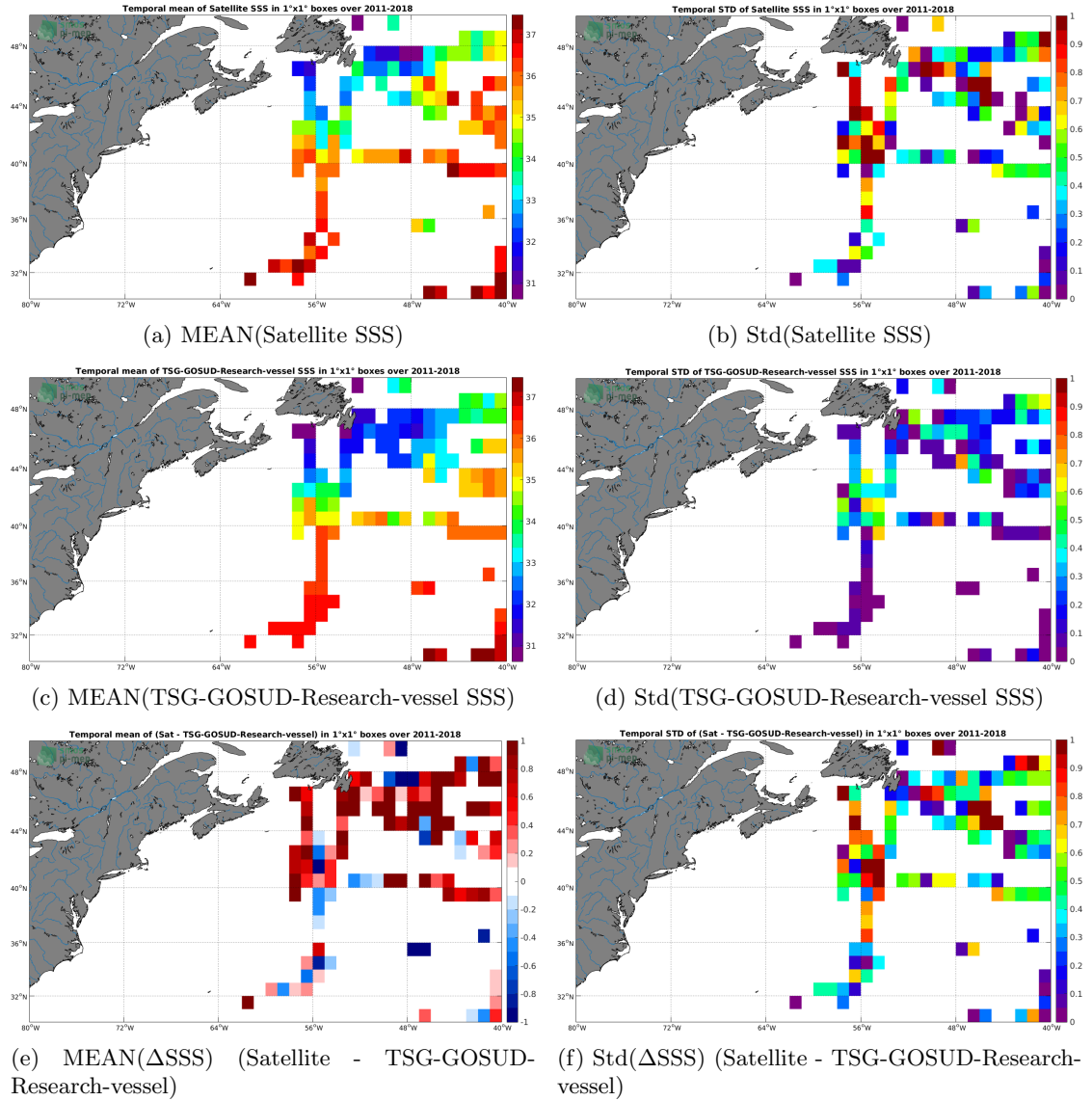
Figure 6: Temporal mean (left) and Std (right) of SSS from SMOS L2 v662 (ESA) (top), TSG-GOSUD-Research-vessel (middle), and of \Delta SSS (Satellite - TSG-GOSUD-Research-vessel). Only match-up pairs are used to generate these maps.
