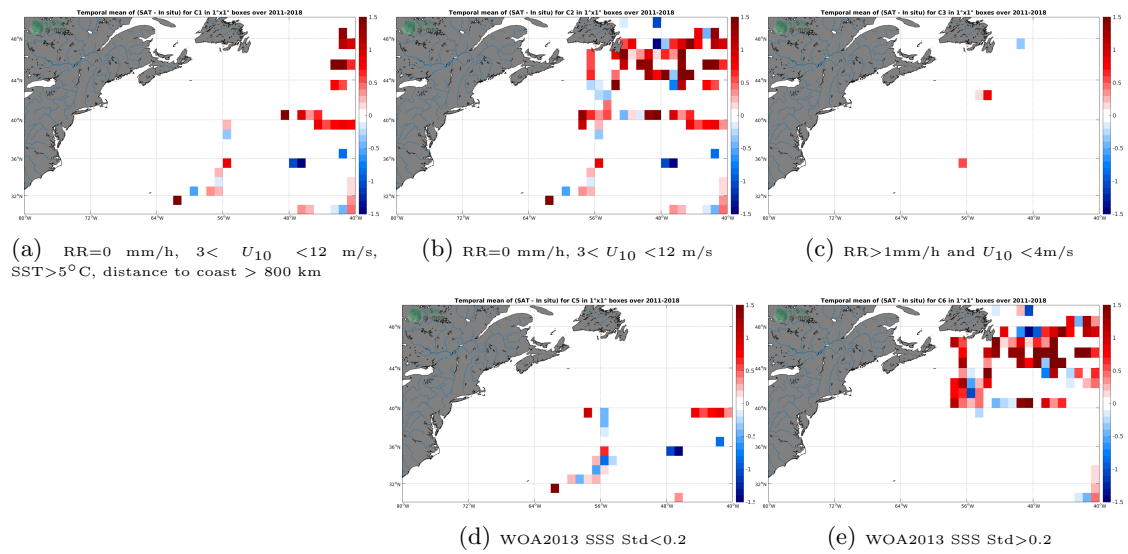
Figure 12: Temporal mean gridded over spatial boxes of size 1^\circ \times 1^\circ of \Delta SSS (SMOS L2 v662 (ESA) - TSG-GOSUD-Research-vessel) for 5 different subdatasets corresponding to:RR=0 mm/h, 3 < U_{10} < 12 m/s, SST > 5°C, distance to coast > 800 km (a), RR=0 mm/h, 3 < U_{10} < 12 m/s (b), RR > 1mm/h and U_{10} < 4 m/s (c), WOA2013 SSS Std < 0.2 (d), WOA2013 SSS Std > 0.2 (e).
