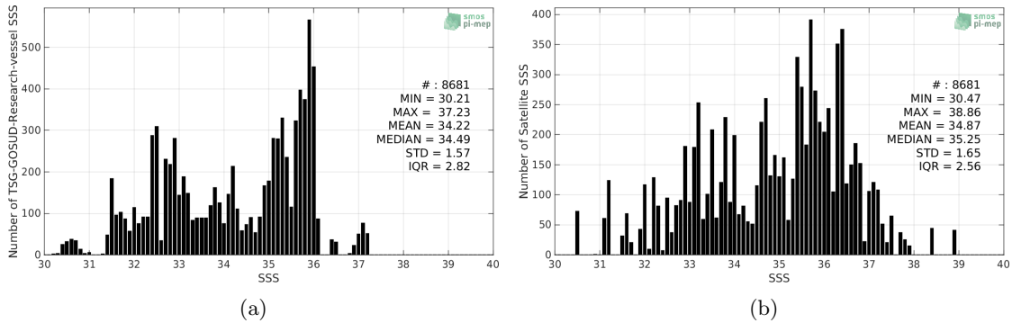
Figure 2: Histograms of SSS from TSG-GOSUD-Research-vessel (a) and SMOS-L2-DPGS-v662 (b) considering all match-up pairs per bins of 0.1 over the Gulf Stream Pi-MEP region and for the full satellite product period.
