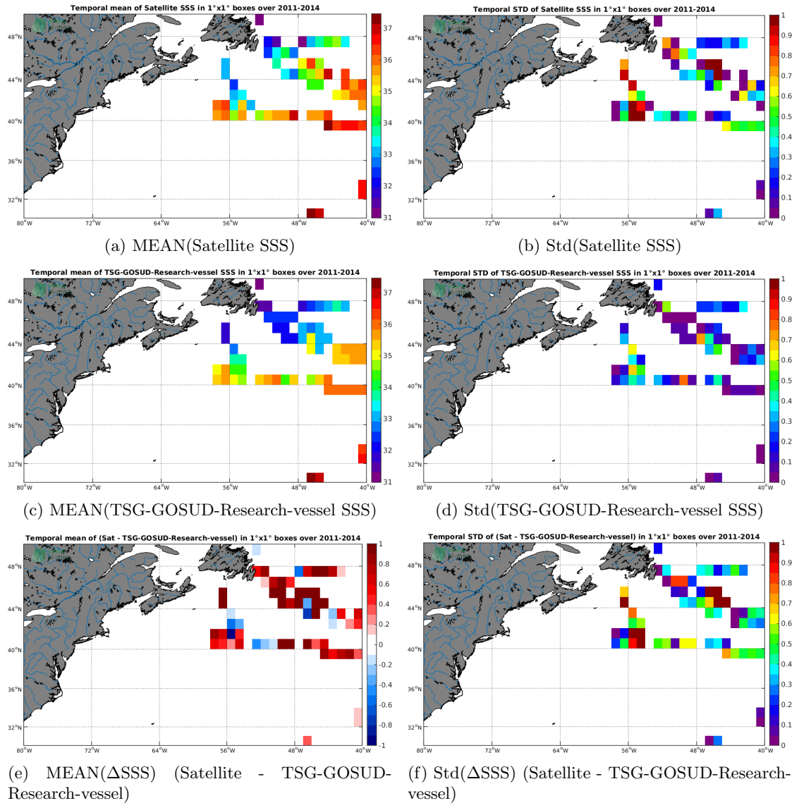
Figure 6: Temporal mean (left) and Std (right) of SSS from SMOS-L2-DPGS-v662 (top), TSG-GOSUD-Research-vessel (middle), and of \Delta SSS (Satellite - TSG-GOSUD-Research-vessel). Only match-up pairs are used to generate these maps.
