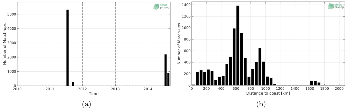
Figure 1: Number of match-ups between TSG-GOSUD-Research-vessel and SMOS-L2-DPGS-v662 SSS as a function of time (a) and as function of the distance to coast (b) over the Gulf Stream Pi-MEP region and for the full satellite product period.
