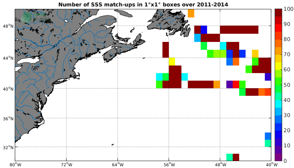
Figure 4: Number of SSS match-ups between TSG-GOSUD-Research-vessel SSS and the SMOS-L2-DPGS-v662 SSS product for the Gulf Stream Pi-MEP region over 1^\circ \times 1^\circ boxes and for the full satellite product period.
