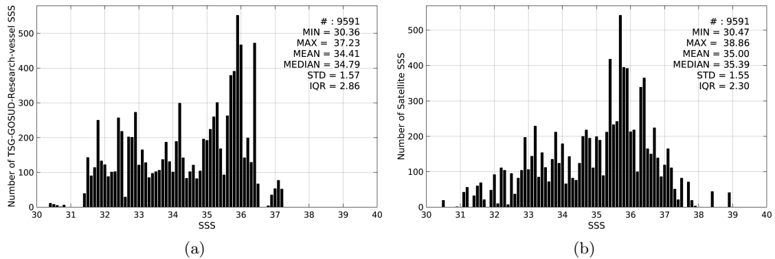
Figure 2: Histograms of SSS from TSG-GOSUD-Research-vessel (a) and SMOS-L2-DPGS-v662 (b) considering all match-up pairs per bins of 0.1 over the Gulf Stream Pi-MEP region and for the full satellite product period.
