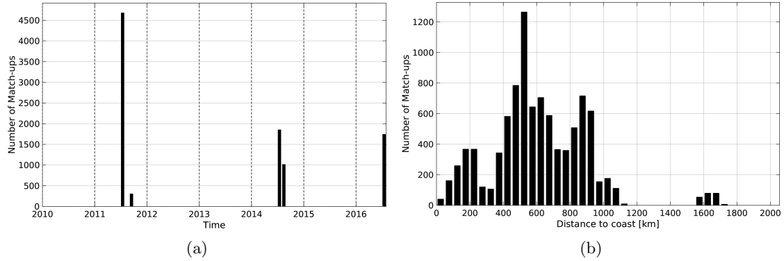
Figure 1: Number of match-ups between TSG-GOSUD-Research-vessel and SMOS-L2-DPGS-v662 SSS as a function of time (a) and as function of the distance to coast (b) over the Gulf Stream Pi-MEP region and for the full satellite product period.
