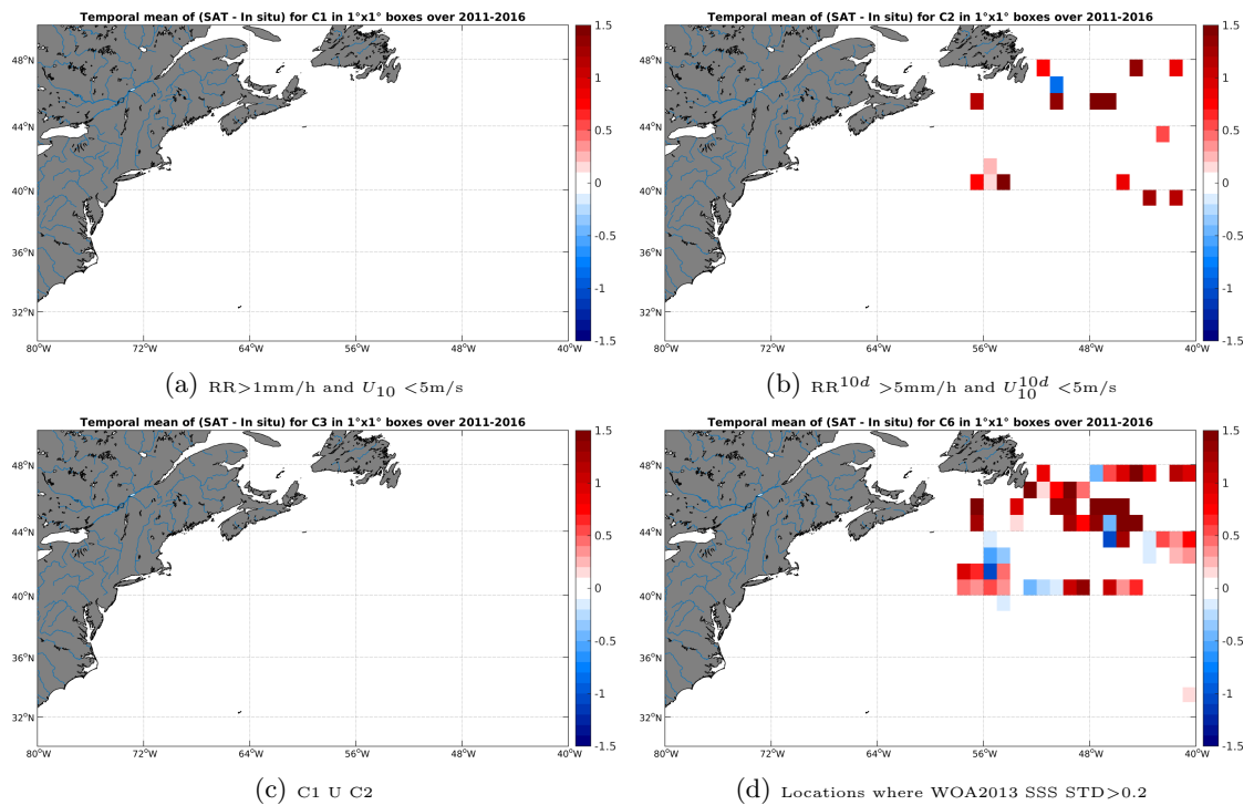
Figure 12: Temporal mean gridded over spatial boxes of size 1^\circ \times 1^\circ of \Delta SSS (SMOS-L2-DPGS-v662 - TSG-GOSUD-Research-vessel) for 4 different subdatasets corresponding to:RR >1 mm/h and U_{10} < 5 m/s (a), RR^{10d} > 5 mm/h and U_{10}^{10d} < 5 m/s (b), C1 U C2 (c),Locations where WOA2013 SSS STD >0.2 (d).
