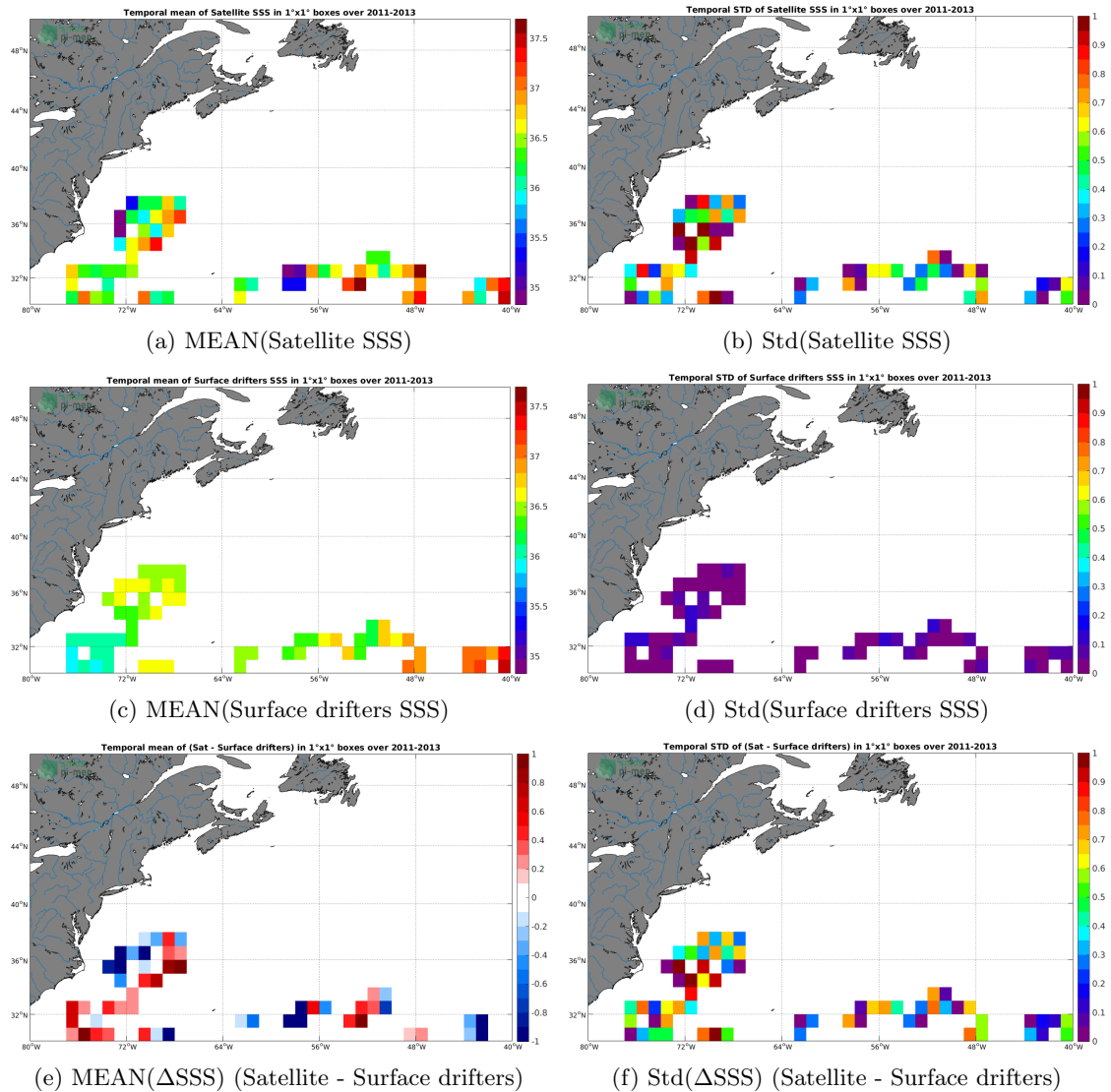
Figure 5: Temporal mean (left) and Std (right) of SSS from SMOS SSS L2 v662 (ESA) (top), Surface drifters (middle), and of \Delta\text{SSS} (Satellite - Surface drifters). Only match-up pairs are used to generate these maps.
