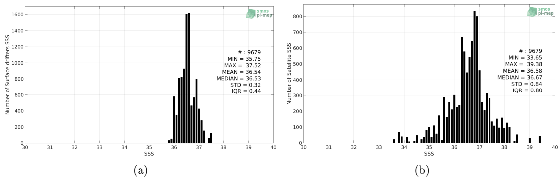
Figure 2: Histograms of SSS from Surface drifters (a) and SMOS SSS L2 v662 (ESA) (b) considering all match-up pairs per bins of 0.1 over the Gulf Stream Pi-MEP region and for the full satellite product period.
