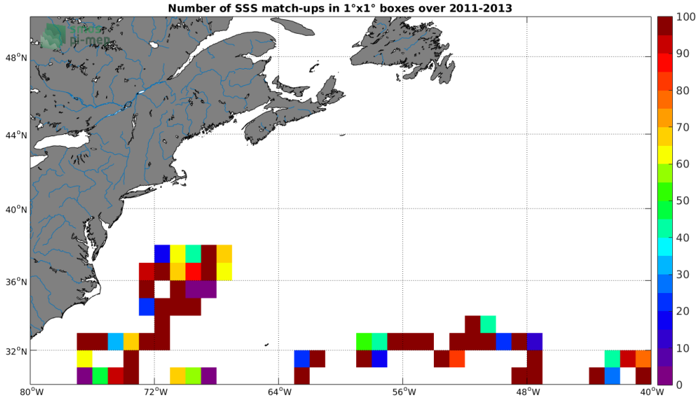
Figure 3: Number of SSS match-ups between Surface drifters SSS and the SMOS SSS L2 v662 (ESA) SSS product for the Gulf Stream Pi-MEP region over 1°x1° boxes and for the full satellite product period.
