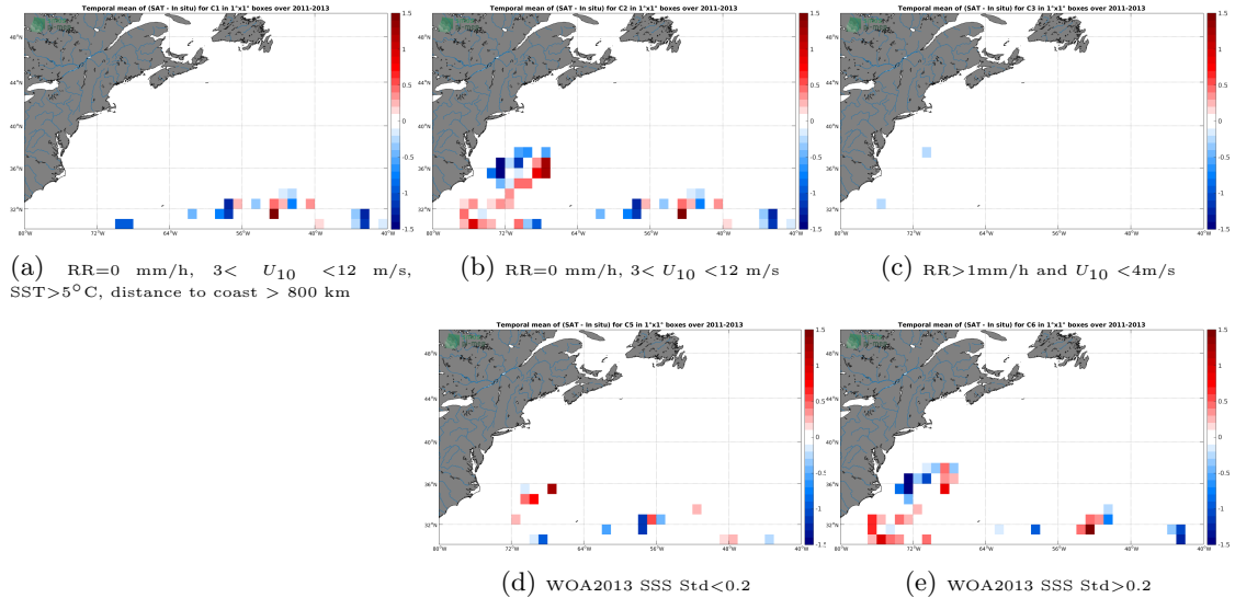
Figure 11: Temporal mean gridded over spatial boxes of size 1^{\circ}\times 1^{\circ} of \Delta\text{SSS} (SMOS SSS L2 v662 (ESA) - Surface drifters) for 5 different subdatasets corresponding to:RR=0 mm/h, 3 < U_{10} < 12 m/s, SST >5^{\circ}\text{C} , distance to coast > 800 km (a), RR=0 mm/h, 3 < U_{10} < 12 m/s (b), RR >1 mm/h and U_{10} < 4 m/s (c), WOA2013 SSS Std <0.2 (d), WOA2013 SSS Std >0.2 (e).
