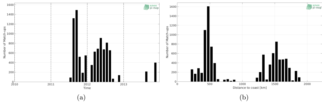
Figure 1: Number of match-ups between Surface drifters and SMOS SSS L2 v662 (ESA) SSS as a function of time (a) and as function of the distance to coast (b) over the Gulf Stream Pi-MEP region and for the full satellite product period.
