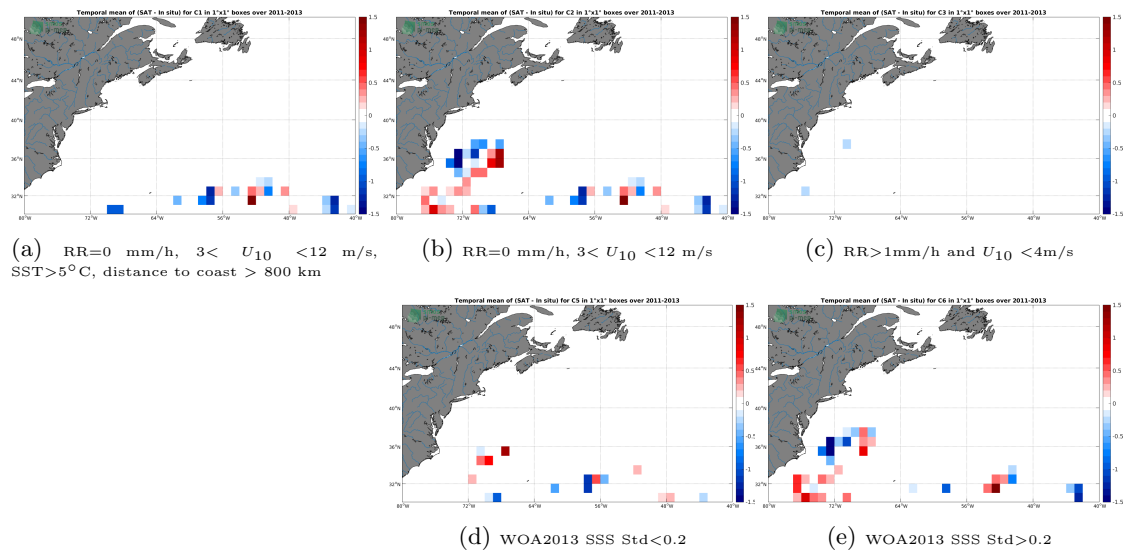
Figure 11: Temporal mean gridded over spatial boxes of size 1^{\circ}\times 1^{\circ} of \Delta\text{SSS} (SMOS L2 v662 (ESA) - Surface drifters) for 5 different subdatasets corresponding to:RR=0 mm/h, 3 < U_{10} < 12 m/s, SST >5^{\circ}\text{C} , distance to coast > 800 km (a), RR=0 mm/h, 3 < U_{10} < 12 m/s (b), RR >1 mm/h and U_{10} < 4 m/s (c), WOA2013 SSS Std <0.2 (d), WOA2013 SSS Std >0.2 (e).
