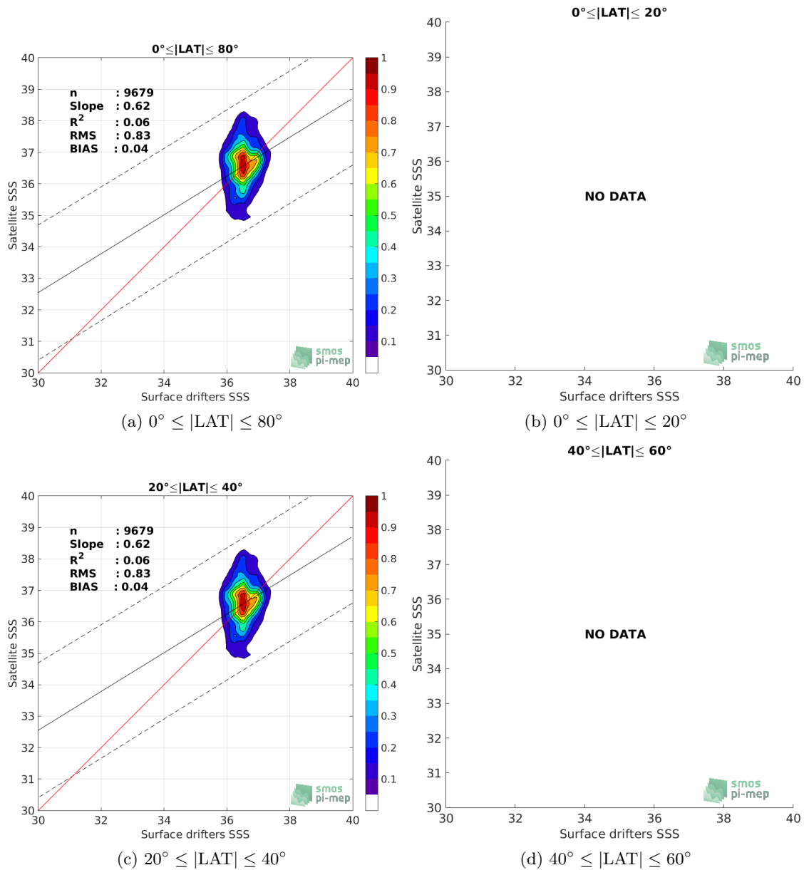
Figure 8: Contour maps of the concentration of SMOS L2 v662 (ESA) SSS (y-axis) versus Surface drifters SSS (x-axis) at match-up pairs for different latitude bands. For each plot, the red line shows x=y . The black thin and dashed lines indicate a linear fit through the data cloud and the \pm 95\% confidence levels, respectively. The number match-up pairs n , the slope and R^2 coefficient of the linear fit, the root mean square (RMS) and the mean bias between satellite and in situ data are indicated for each latitude band in each plots.
