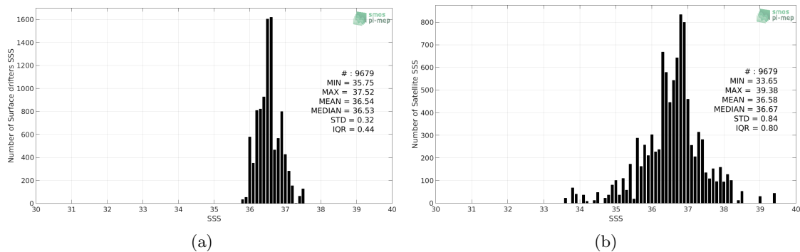
Figure 2: Histograms of SSS from Surface drifters (a) and SMOS L2 v662 (ESA) (b) considering all match-up pairs per bins of 0.1 over the Gulf Stream Pi-MEP region and for the full satellite product period.
