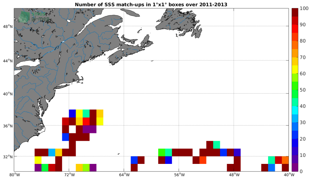
Figure 3: Number of SSS match-ups between Surface drifters SSS and the SMOS L2 v662 (ESA) SSS product for the Gulf Stream Pi-MEP region over 1^\circ \times 1^\circ boxes and for the full satellite product period.
