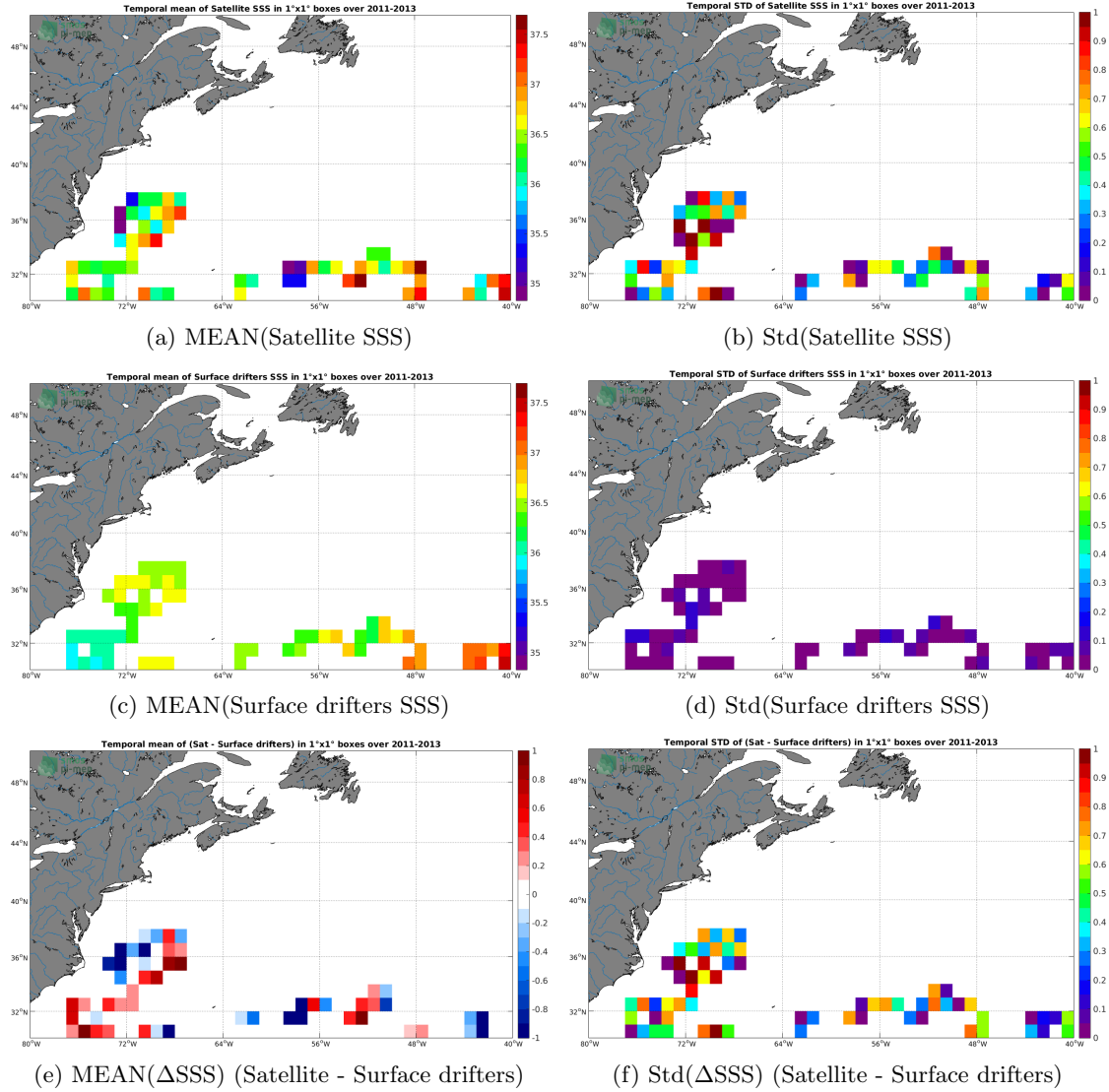
Figure 5: Temporal mean (left) and Std (right) of SSS from SMOS L2 v662 (ESA) (top), Surface drifters (middle), and of \Delta\text{SSS} (Satellite - Surface drifters). Only match-up pairs are used to generate these maps.
