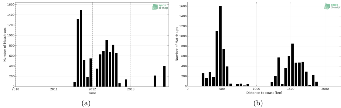
Figure 1: Number of match-ups between Surface drifters and SMOS L2 v662 (ESA) SSS as a function of time (a) and as function of the distance to coast (b) over the Gulf Stream Pi-MEP region and for the full satellite product period.
