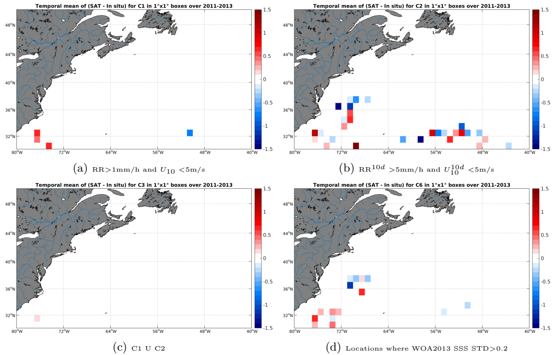
Figure 11: Temporal mean gridded over spatial boxes of size 1^\circ \times 1^\circ of \Delta SSS (SMOS-L2-DPGS-v662 - Surface drifters) for 4 different subdatasets corresponding to: RR > 1mm/h and U_{10} < 5 m/s (a), RR^{10d} > 5 mm/h and U_{10}^{10d} < 5 m/s (b), C1 U C2 (c), Locations where WOA2013 SSS STD > 0.2 (d).
