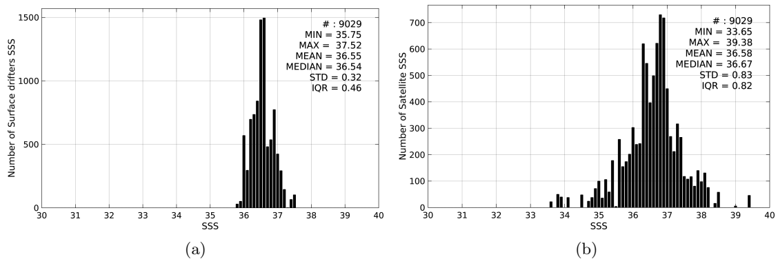
Figure 2: Histograms of SSS from Surface drifters (a) and SMOS-L2-DPGS-v662 (b) considering all match-up pairs per bins of 0.1 over the Gulf Stream Pi-MEP region and for the full satellite product period.
