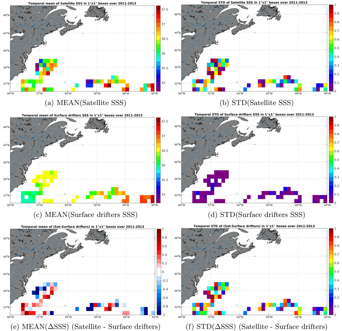
Figure 5: Temporal mean (left) and STD (right) of SSS from SMOS-L2-DPGS-v662 (top), Surface drifters (middle), and of \Delta\text{SSS} (Satellite - Surface drifters). Only match-up pairs are used to generate these maps.
