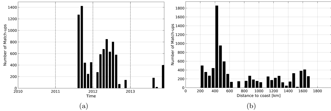
Figure 1: Number of match-ups between Surface drifters and SMOS-L2-DPGS-v662 SSS as a function of time (a) and as function of the distance to coast (b) over the Gulf Stream Pi-MEP region and for the full satellite product period.
