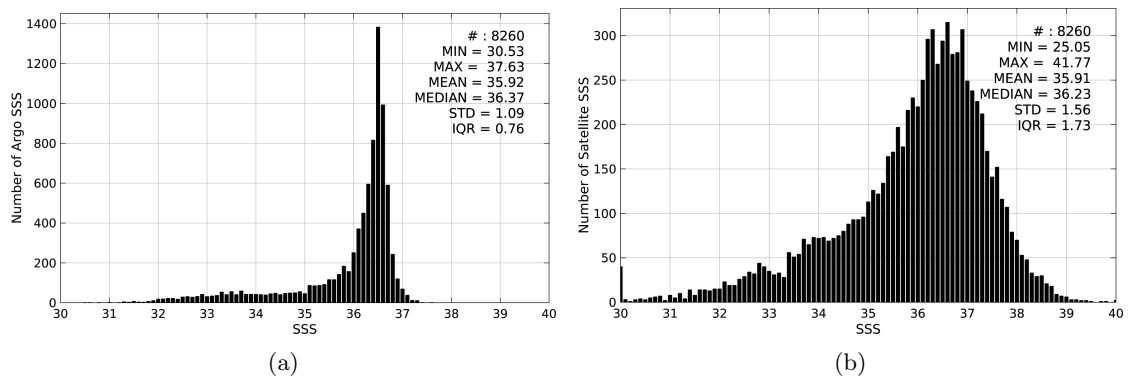
Figure 2: Histograms of SSS from Argo (a) and SMOS-L2-DPGS-v662 (b) considering all match-up pairs per bins of 0.1 over the Gulf Stream Pi-MEP region and for the full satellite product period.
