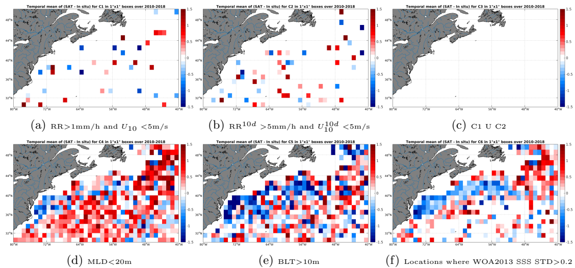
Figure 12: Temporal mean gridded over spatial boxes of size 1^\circ \times 1^\circ of \Delta\text{SSS} (SMOS-L2-DPGS-v662 - Argo) for 6 different subdatasets corresponding to: RR > 1\text{mm/h} and U_{10} < 5\text{m/s} (a), RR^{10d} > 5\text{mm/h} and U_{10}^{10d} < 5\text{m/s} (b), C1 U C2 (c), MLD < 20\text{m} (d), BLT > 10\text{m} (e), Locations where WOA2013 SSS STD > 0.2 (f).
