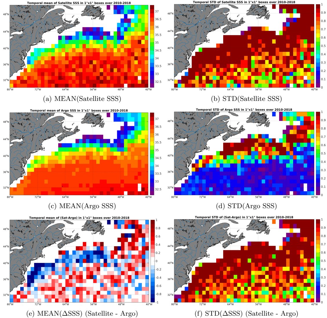
Figure 6: Temporal mean (left) and STD (right) of SSS from SMOS-L2-DPGS-v662 (top), Argo (middle), and of \Delta SSS (Satellite - Argo). Only match-up pairs are used to generate these maps.
