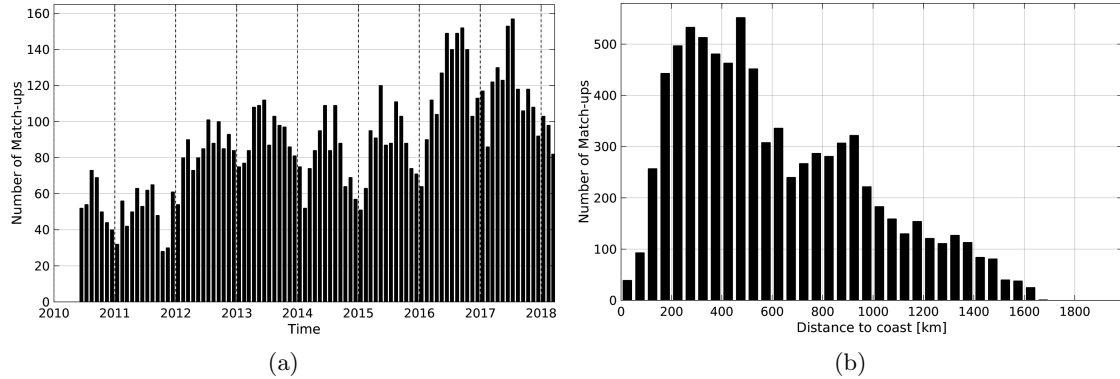
Figure 1: Number of match-ups between Argo and SMOS-L2-DPGS-v662 SSS as a function of time (a) and as function of the distance to coast (b) over the Gulf Stream Pi-MEP region and for the full satellite product period.
