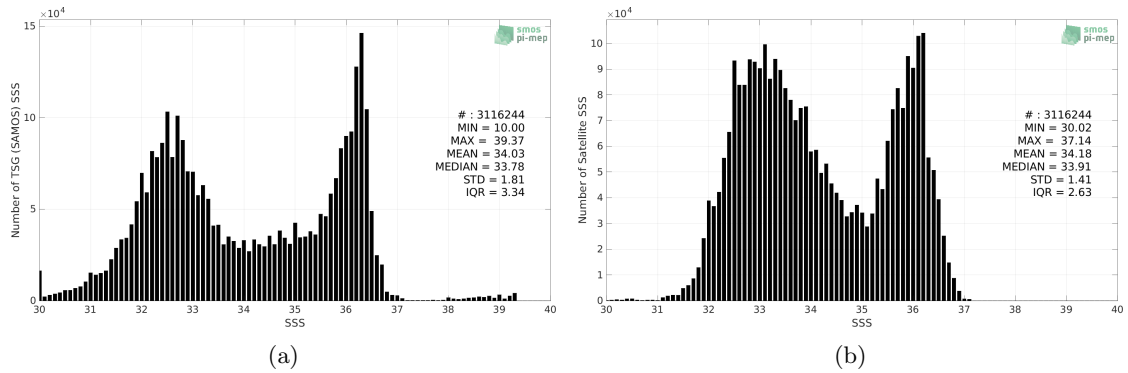
Figure 2: Histograms of SSS from TSG (SAMOS) (a) and SMAP SSS L4 OI v1 - 7 Days (IPRC) (b) considering all match-up pairs per bins of 0.1 over the Gulf Stream Pi-MEP region and for the full satellite product period.
