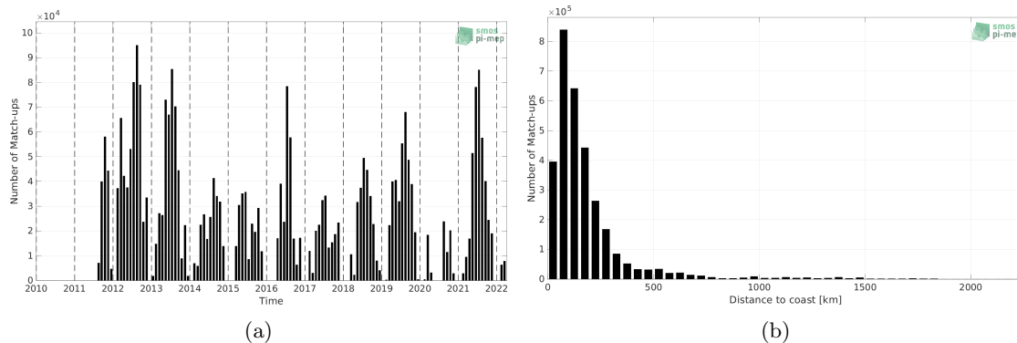
Figure 1: Number of match-ups between TSG (SAMOS) and SMAP SSS L4 OI v1 - 7 Days (IPRC) SSS as a function of time (a) and as function of the distance to coast (b) over the Gulf Stream Pi-MEP region and for the full satellite product period.
