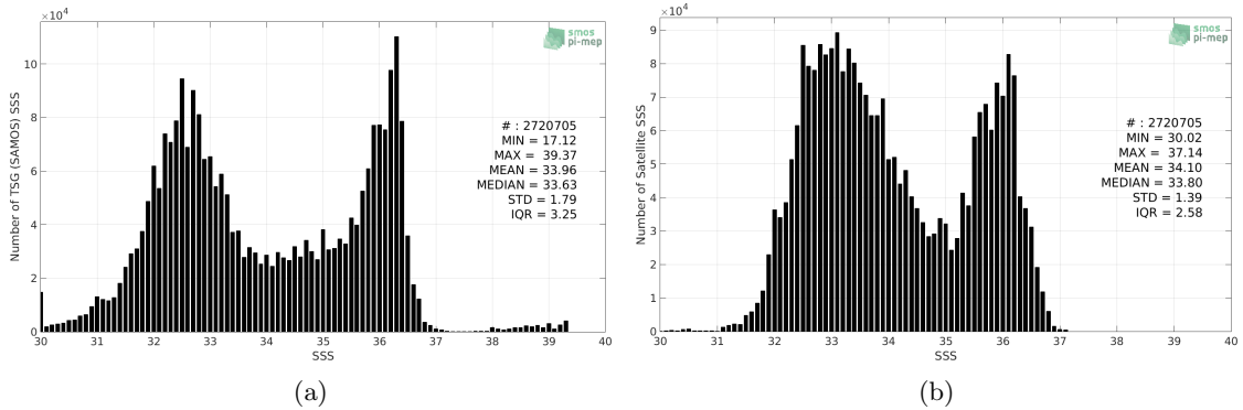
Figure 2: Histograms of SSS from TSG (SAMOS) (a) and SMAP SSS L4 OI v1 - 7day (IPRC) (b) considering all match-up pairs per bins of 0.1 over the Gulf Stream Pi-MEP region and for the full satellite product period.
