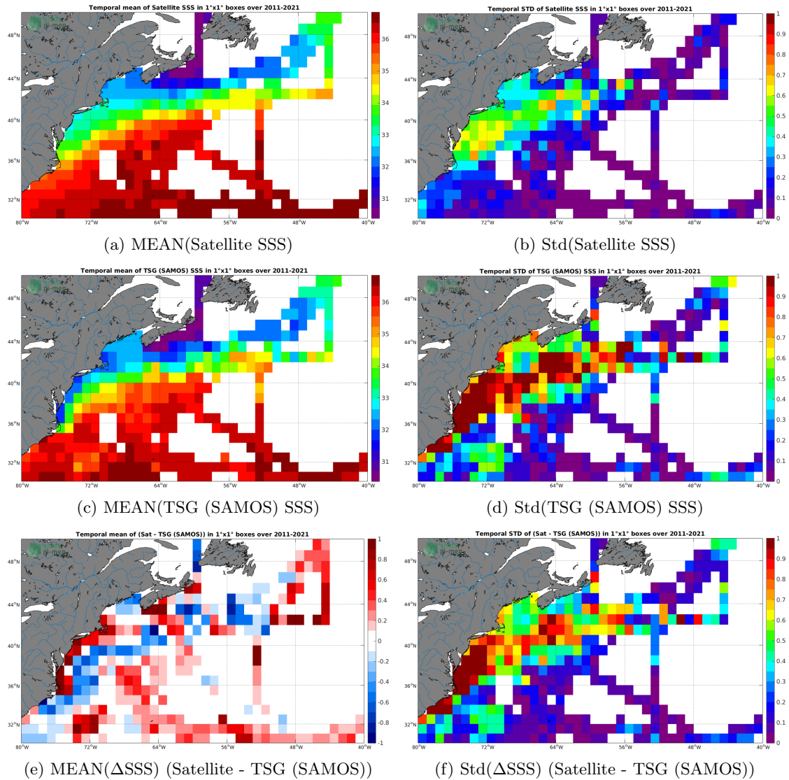
Figure 6: Temporal mean (left) and Std (right) of SSS from SMAP SSS L4 OI v1 - 7day (IPRC) (top), TSG (SAMOS) (middle), and of \Delta SSS (Satellite - TSG (SAMOS)). Only match-up pairs are used to generate these maps.
