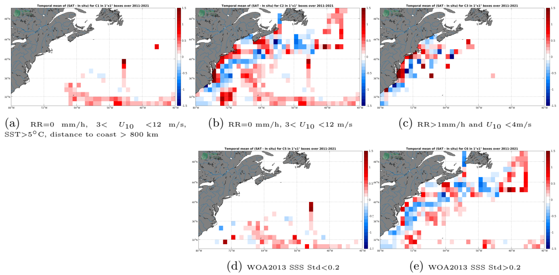
Figure 12: Temporal mean gridded over spatial boxes of size 1°x1° of \Delta SSS (SMAP SSS L4 OI v1 - 7day (IPRC) - TSG (SAMOS)) for 5 different subdatasets corresponding to:RR=0 mm/h, 3 < U_{10} < 12 m/s, SST>5°C, distance to coast > 800 km (a), RR=0 mm/h, 3 < U_{10} < 12 m/s (b), RR>1mm/h and U_{10} < 4 m/s (c), WOA2013 SSS Std<0.2 (d), WOA2013 SSS Std>0.2 (e).
