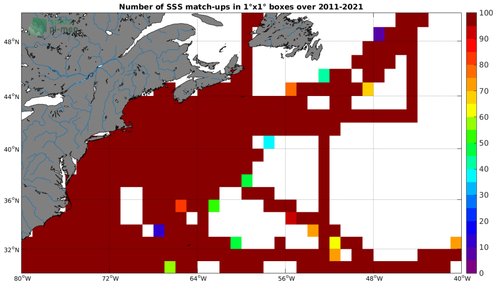
Figure 4: Number of SSS match-ups between TSG (SAMOS) SSS and the SMAP SSS L4 OI v1 - 7day (IPRC) SSS product for the Gulf Stream Pi-MEP region over 1^\circ \times 1^\circ boxes and for the full satellite product period.
