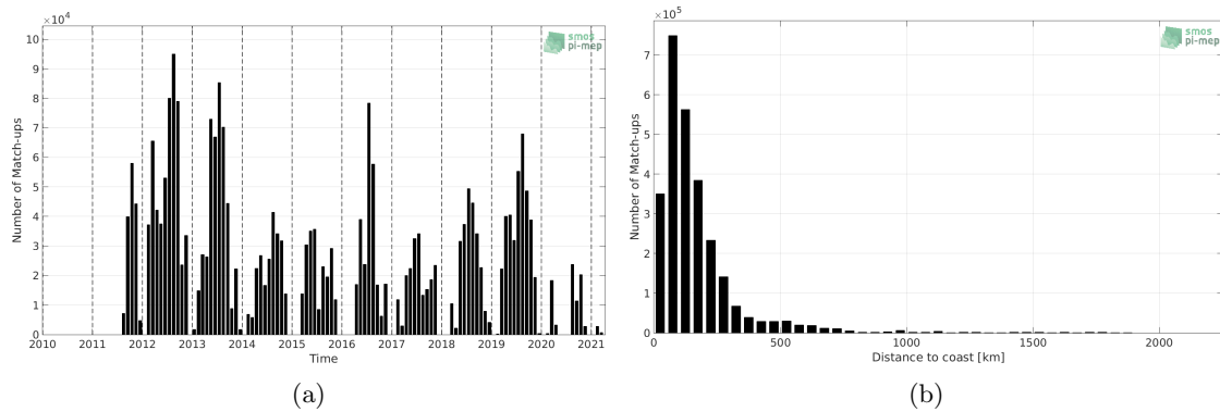
Figure 1: Number of match-ups between TSG (SAMOS) and SMAP SSS L4 OI v1 - 7day (IPRC) SSS as a function of time (a) and as function of the distance to coast (b) over the Gulf Stream Pi-MEP region and for the full satellite product period.
