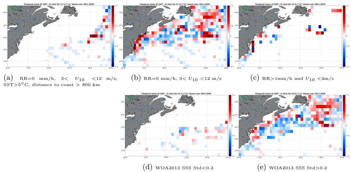
Figure 12: Temporal mean gridded over spatial boxes of size 1^\circ \times 1^\circ of \Delta SSS (SMAP SSS L4 OI v1 - 7day (IPRC) - TSG (LEGOS-DM)) for 5 different subdatasets corresponding to:RR=0 mm/h, 3 < U_{10} < 12 m/s, SST > 5^\circ\text{C} , distance to coast > 800 km (a), RR=0 mm/h, 3 < U_{10} < 12 m/s (b), RR > 1 mm/h and U_{10} < 4 m/s (c), WOA2013 SSS Std < 0.2 (d), WOA2013 SSS Std > 0.2 (e).
