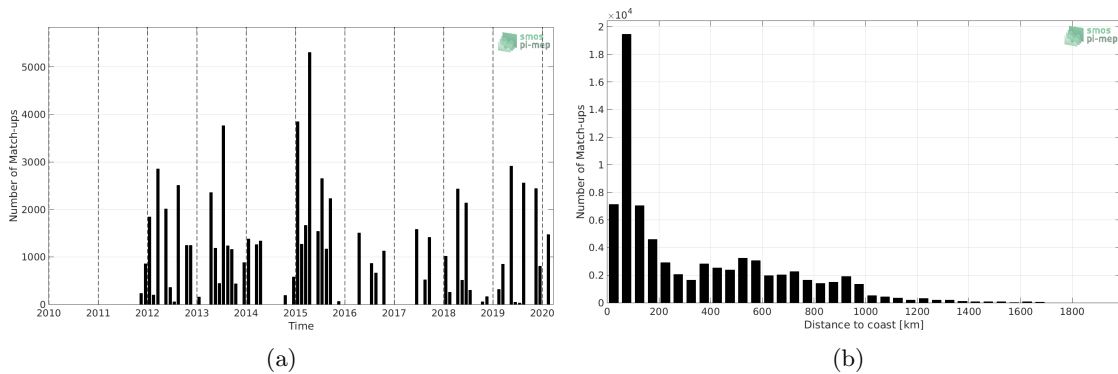
Figure 1: Number of match-ups between TSG (LEGOS-DM) and SMAP SSS L4 OI v1 - 7day (IPRC) SSS as a function of time (a) and as function of the distance to coast (b) over the Gulf Stream Pi-MEP region and for the full satellite product period.
