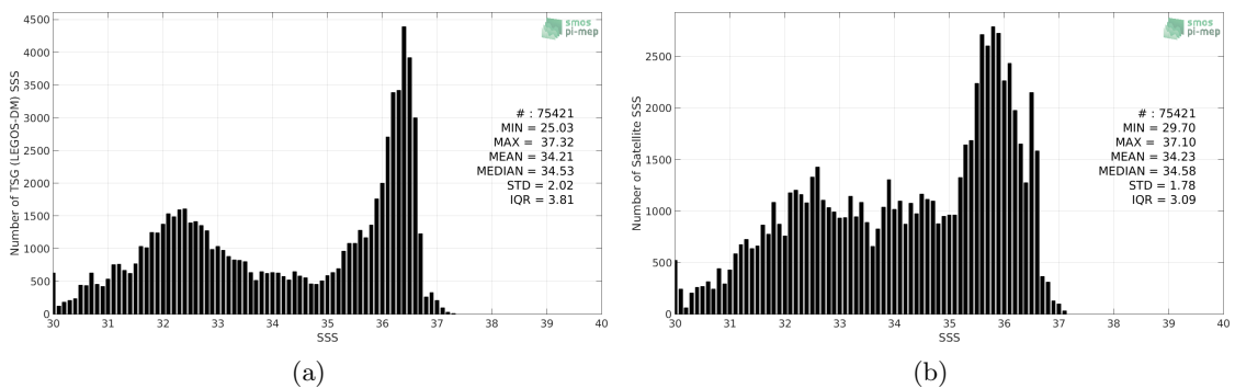
Figure 2: Histograms of SSS from TSG (LEGOS-DM) (a) and SMAP SSS L4 OI v1 - 7day (IPRC) (b) considering all match-up pairs per bins of 0.1 over the Gulf Stream Pi-MEP region and for the full satellite product period.
