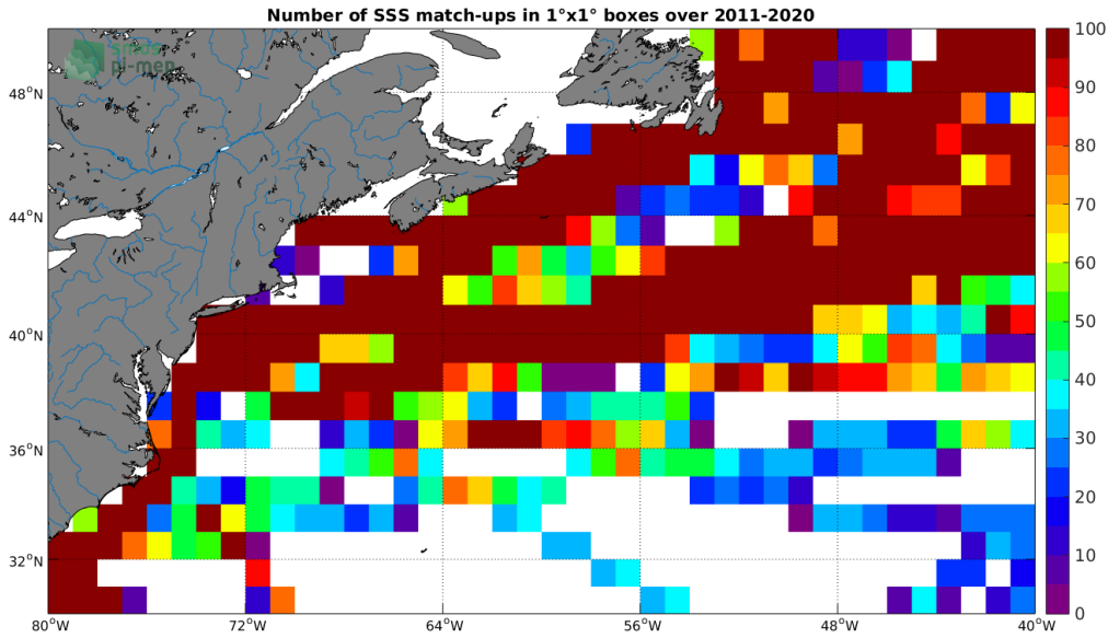
Figure 4: Number of SSS match-ups between TSG (LEGOS-DM) SSS and the SMAP SSS L4 OI v1 - 7day (IPRC) SSS product for the Gulf Stream Pi-MEP region over 1^{\circ} \times 1^{\circ} boxes and for the full satellite product period.
