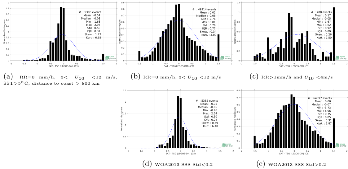
Figure 13: Normalized histogram of \Delta SSS (SMAP SSS L4 OI v1 - 7day (IPRC) - TSG (LEGOS-DM)) for 5 different subdatasets corresponding to: RR=0 mm/h, 3 < U_{10} < 12 m/s, SST > 5°C, distance to coast > 800 km (a), RR=0 mm/h, 3 < U_{10} < 12 m/s (b), RR > 1mm/h and U_{10} < 4 m/s (c), WOA2013 SSS Std < 0.2 (d), WOA2013 SSS Std > 0.2 (e).
