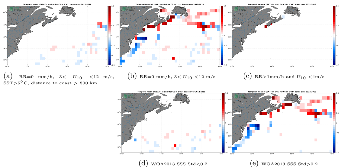
Figure 12: Temporal mean gridded over spatial boxes of size 1^\circ \times 1^\circ of \Delta SSS (SMAP SSS L4 OI v1 - 7 Days (IPRC) - TSG (GOSUD-Sailing-ship)) for 5 different subdatasets corresponding to: RR=0 mm/h, 3 < U_{10} < 12 m/s, SST>5°C, distance to coast > 800 km (a), RR=0 mm/h, 3 < U_{10} < 12 m/s (b), RR>1mm/h and U_{10} < 4 m/s (c), WOA2013 SSS Std<0.2 (d), WOA2013 SSS Std>0.2 (e).
