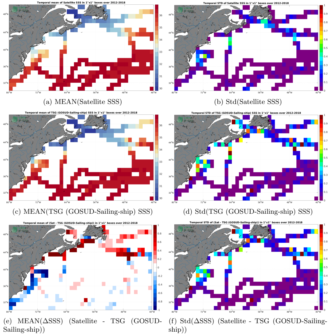
Figure 6: Temporal mean (left) and Std (right) of SSS from SMAP SSS L4 OI v1 - 7 Days (IPRC) (top), TSG (GOSUD-Sailing-ship) (middle), and of \Delta SSS (Satellite - TSG (GOSUD-Sailing-ship)). Only match-up pairs are used to generate these maps.
