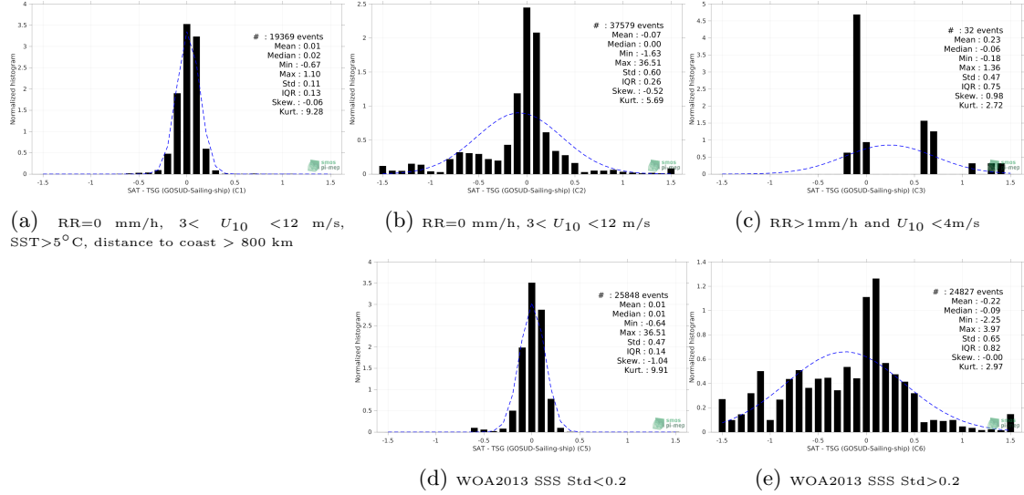
Figure 13: Normalized histogram of \Delta\text{SSS} (SMAP SSS L4 OI v1 - 7 Days (IPRC) - TSG (GOSUD-Sailing-ship)) for 5 different subdatasets corresponding to: RR=0 mm/h, 3 < U_{10} < 12 m/s, SST>5°C, distance to coast > 800 km (a), RR=0 mm/h, 3 < U_{10} < 12 m/s (b), RR>1mm/h and U_{10} < 4 m/s (c), WOA2013 SSS Std<0.2 (d), WOA2013 SSS Std>0.2 (e).
