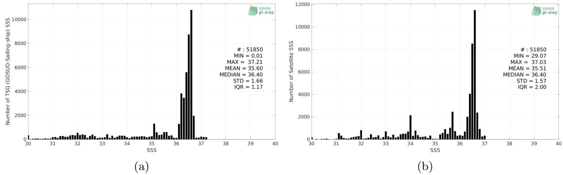
Figure 2: Histograms of SSS from TSG (GOSUD-Sailing-ship) (a) and SMAP SSS L4 OI v1 - 7 Days (IPRC) (b) considering all match-up pairs per bins of 0.1 over the Gulf Stream Pi-MEP region and for the full satellite product period.
