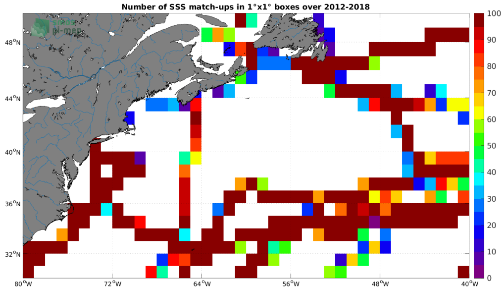
Figure 4: Number of SSS match-ups between TSG (GOSUD-Sailing-ship) SSS and the SMAP SSS L4 OI v1 - 7 Days (IPRC) SSS product for the Gulf Stream Pi-MEP region over 1^\circ \times 1^\circ boxes and for the full satellite product period.
