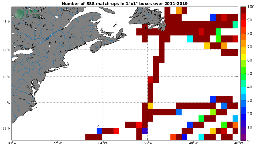
Figure 4: Number of SSS match-ups between TSG (GOSUD-Research-vessel) SSS and the SMAP SSS L4 OI v1 - 7 Days (IPRC) SSS product for the Gulf Stream Pi-MEP region over 1^\circ \times 1^\circ boxes and for the full satellite product period.
