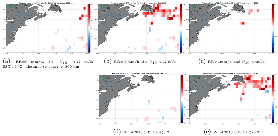
Figure 12: Temporal mean gridded over spatial boxes of size 1^\circ \times 1^\circ of \Delta SSS (SMAP SSS L4 OI v1 - 7 Days (IPRC) - TSG (GOSUD-Research-vessel)) for 5 different subdatasets corresponding to: RR=0 mm/h, 3 < U_{10} < 12 m/s, SST > 5°C, distance to coast > 800 km (a), RR=0 mm/h, 3 < U_{10} < 12 m/s (b), RR > 1mm/h and U_{10} < 4 m/s (c), WOA2013 SSS Std < 0.2 (d), WOA2013 SSS Std > 0.2 (e).
