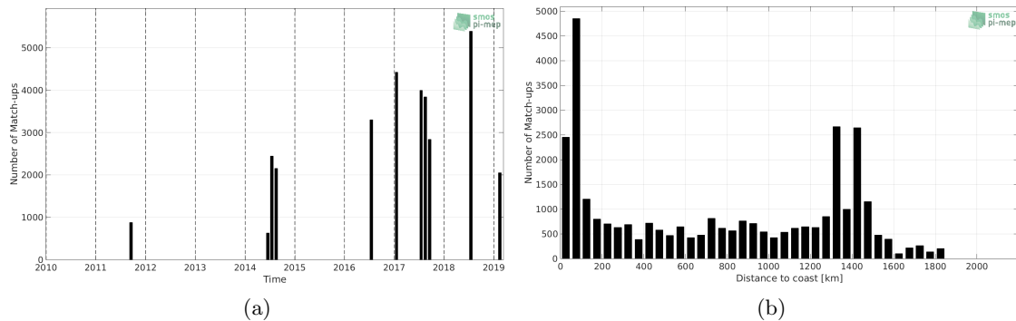
Figure 1: Number of match-ups between TSG (GOSUD-Research-vessel) and SMAP SSS L4 OI v1 - 7 Days (IPRC) SSS as a function of time (a) and as function of the distance to coast (b) over the Gulf Stream Pi-MEP region and for the full satellite product period.
