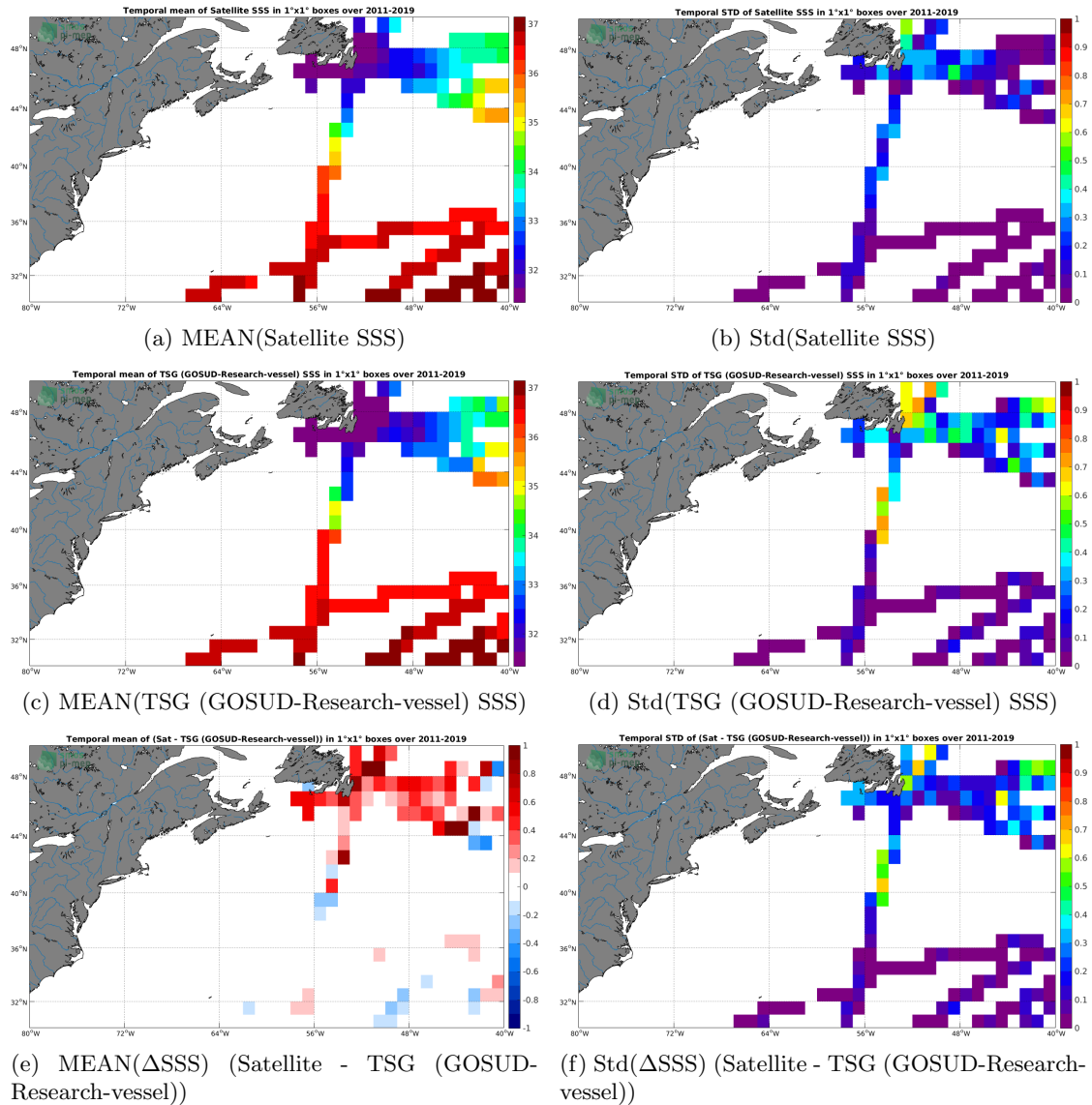
Figure 6: Temporal mean (left) and Std (right) of SSS from SMAP SSS L4 OI v1 - 7 Days (IPRC) (top), TSG (GOSUD-Research-vessel) (middle), and of \Delta SSS (Satellite - TSG (GOSUD-Research-vessel)). Only match-up pairs are used to generate these maps.
