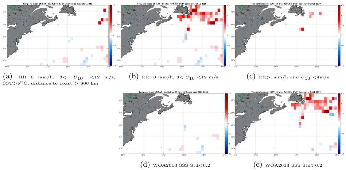
Figure 12: Temporal mean gridded over spatial boxes of size 1^\circ \times 1^\circ of \Delta SSS (SMAP SSS L4 OI v1 - 7day (IPRC) - TSG (GOSUD-Research-vessel)) for 5 different subdatasets corresponding to:RR=0 mm/h, 3 < U_{10} < 12 m/s, SST>5°C, distance to coast > 800 km (a), RR=0 mm/h, 3 < U_{10} < 12 m/s (b), RR>1mm/h and U_{10} < 4 m/s (c), WOA2013 SSS Std<0.2 (d), WOA2013 SSS Std>0.2 (e).
