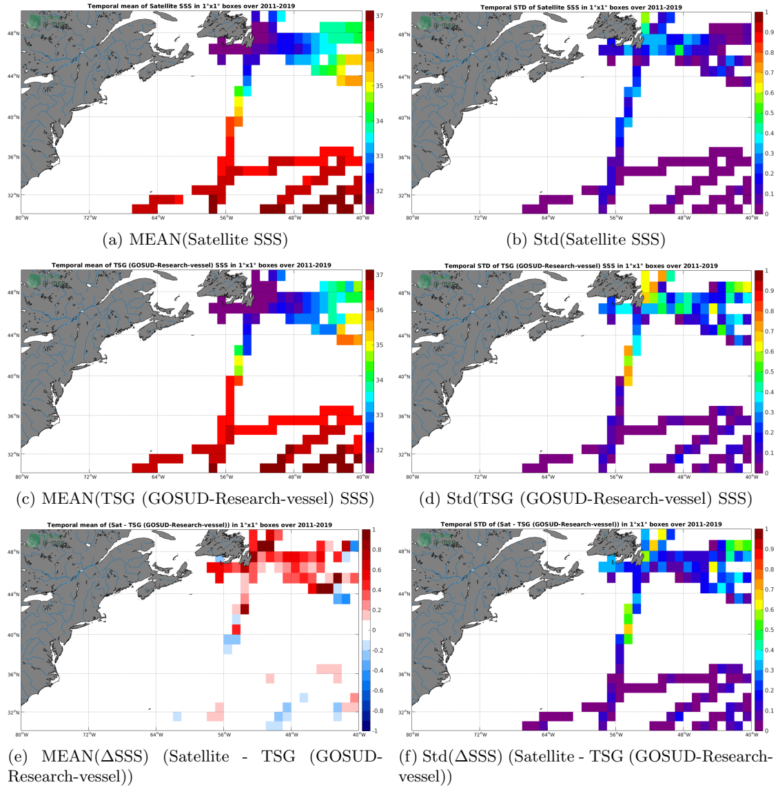
Figure 6: Temporal mean (left) and Std (right) of SSS from SMAP SSS L4 OI v1 - 7day (IPRC) (top), TSG (GOSUD-Research-vessel) (middle), and of \Delta SSS (Satellite - TSG (GOSUD-Research-vessel)). Only match-up pairs are used to generate these maps.
