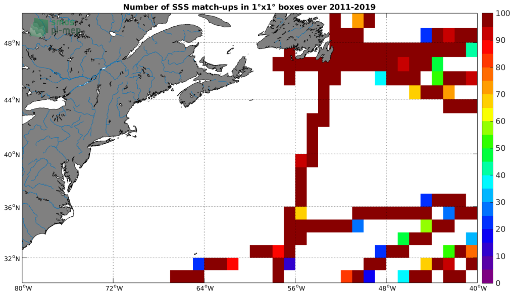
Figure 4: Number of SSS match-ups between TSG (GOSUD-Research-vessel) SSS and the SMAP SSS L4 OI v1 - 7day (IPRC) SSS product for the Gulf Stream Pi-MEP region over 1^\circ \times 1^\circ boxes and for the full satellite product period.
