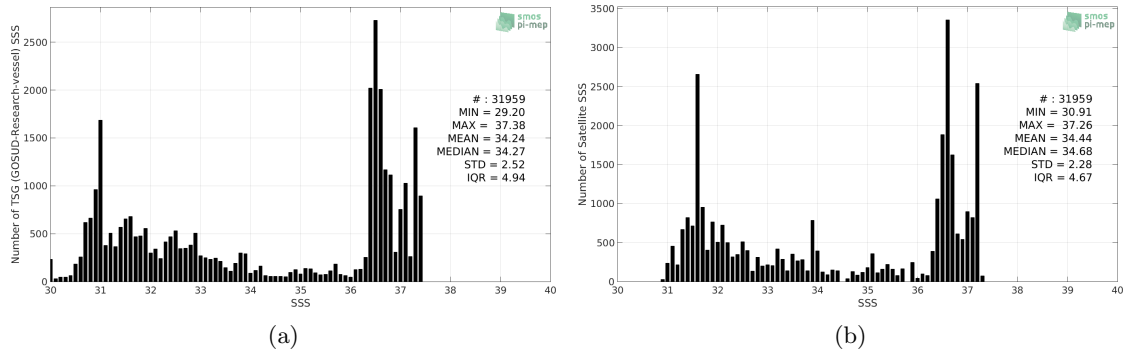
Figure 2: Histograms of SSS from TSG (GOSUD-Research-vessel) (a) and SMAP SSS L4 OI v1 - 7day (IPRC) (b) considering all match-up pairs per bins of 0.1 over the Gulf Stream Pi-MEP region and for the full satellite product period.
