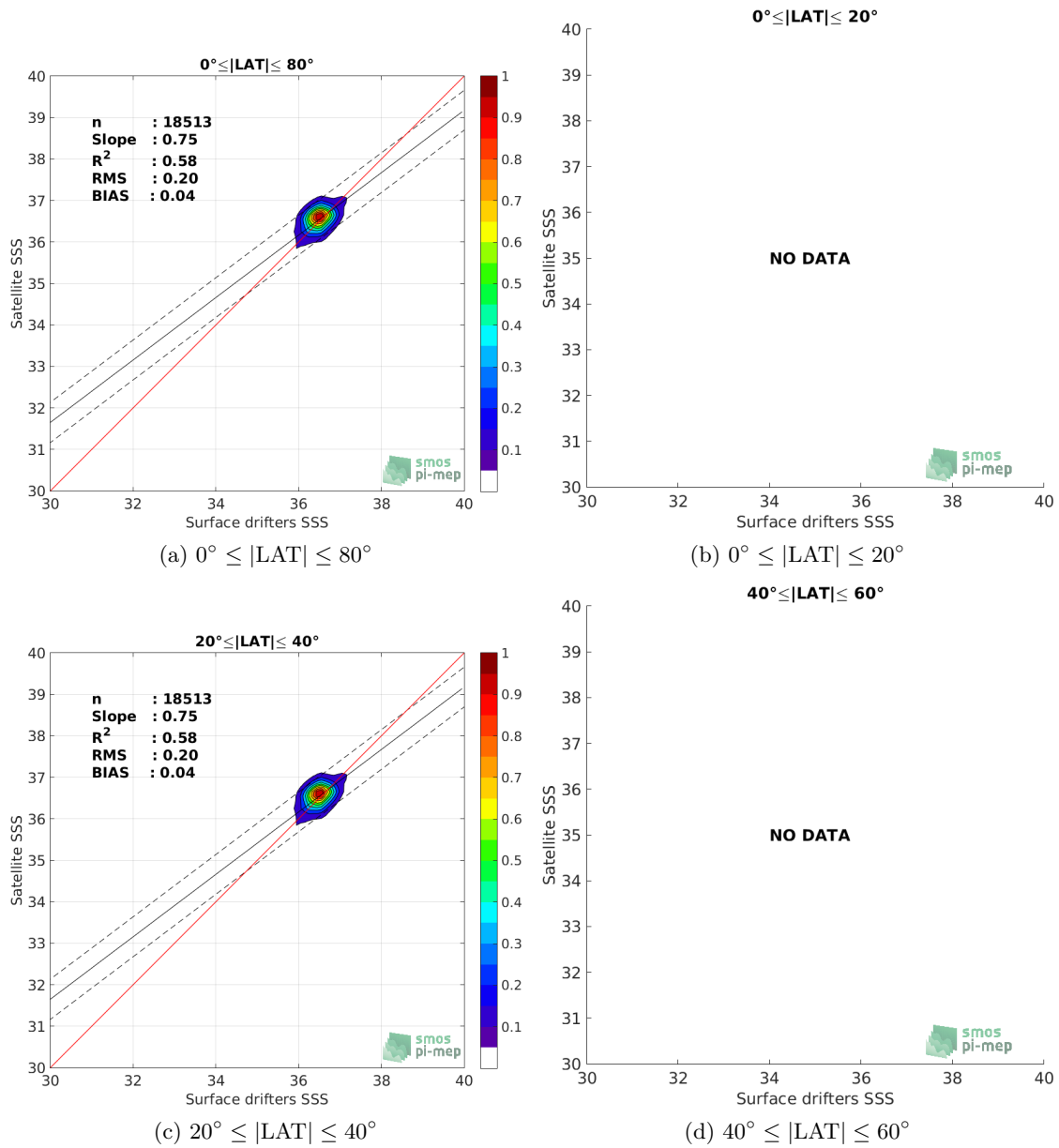
Figure 8: Contour maps of the concentration of SMAP SSS L4 OI v1 - 7day (IPRC) SSS (y-axis) versus Surface drifters SSS (x-axis) at match-up pairs for different latitude bands. For each plot, the red line shows x=y . The black thin and dashed lines indicate a linear fit through the data cloud and the \pm 95\% confidence levels, respectively. The number match-up pairs n , the slope and R^2 coefficient of the linear fit, the root mean square (RMS) and the mean bias between satellite and in situ data are indicated for each latitude band in each plots.
