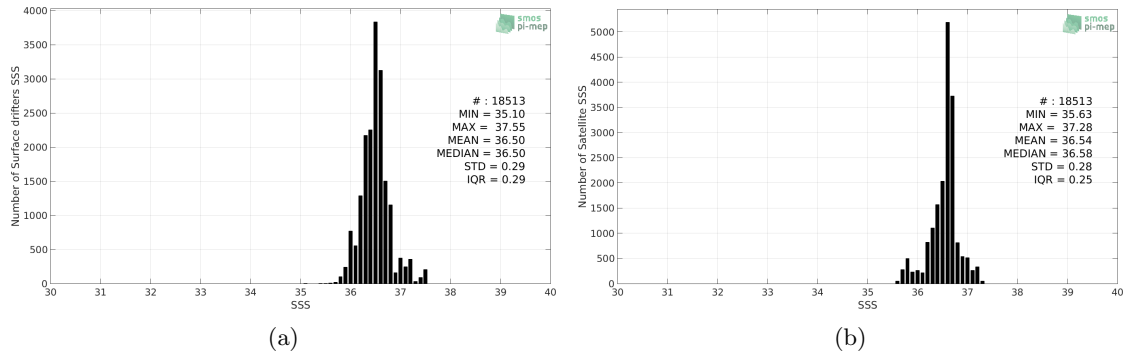
Figure 2: Histograms of SSS from Surface drifters (a) and SMAP SSS L4 OI v1 - 7day (IPRC) (b) considering all match-up pairs per bins of 0.1 over the Gulf Stream Pi-MEP region and for the full satellite product period.
