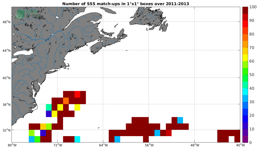
Figure 3: Number of SSS match-ups between Surface drifters SSS and the SMAP SSS L4 OI v1 - 7day (IPRC) SSS product for the Gulf Stream Pi-MEP region over 1^\circ \times 1^\circ boxes and for the full satellite product period.
