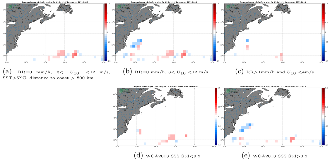
Figure 11: Temporal mean gridded over spatial boxes of size 1^{\circ}\times 1^{\circ} of \Delta\text{SSS} (SMAP SSS L4 OI v1 - 7day (IPRC) - Surface drifters) for 5 different subdatasets corresponding to:RR=0 mm/h, 3 < U_{10} < 12 m/s, SST >5^{\circ}\text{C} , distance to coast > 800 km (a), RR=0 mm/h, 3 < U_{10} < 12 m/s (b), RR >1 mm/h and U_{10} < 4 m/s (c), WOA2013 SSS Std <0.2 (d), WOA2013 SSS Std >0.2 (e).
