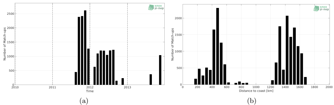
Figure 1: Number of match-ups between Surface drifters and SMAP SSS L4 OI v1 - 7day (IPRC) SSS as a function of time (a) and as function of the distance to coast (b) over the Gulf Stream Pi-MEP region and for the full satellite product period.
