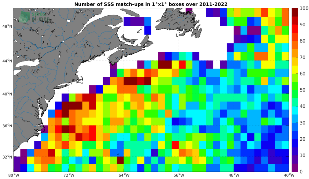
Figure 4: Number of SSS match-ups between Argo SSS and the SMAP SSS L4 OI v1 - 7 Days (IPRC) SSS product for the Gulf Stream Pi-MEP region over 1^{\circ} \times 1^{\circ} boxes and for the full satellite product period.
