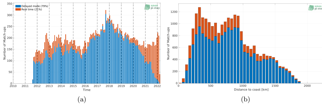
Figure 1: Number of match-ups between Argo and SMAP SSS L4 OI v1 - 7 Days (IPRC) SSS as a function of time (a) and as function of the distance to coast (b) over the Gulf Stream Pi-MEP region and for the full satellite product period.
