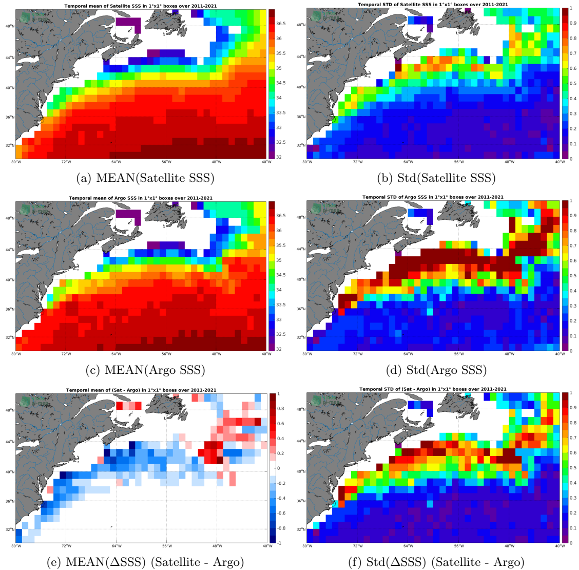
Figure 6: Temporal mean (left) and Std (right) of SSS from SMAP SSS L4 OI v1 - 7day (IPRC) (top), Argo (middle), and of \Delta SSS (Satellite - Argo). Only match-up pairs are used to generate these maps.
