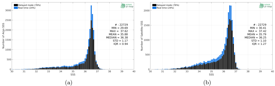
Figure 2: Histograms of SSS from Argo (a) and SMAP SSS L4 OI v1 - 7day (IPRC) (b) considering all match-up pairs per bins of 0.1 over the Gulf Stream Pi-MEP region and for the full satellite product period.
