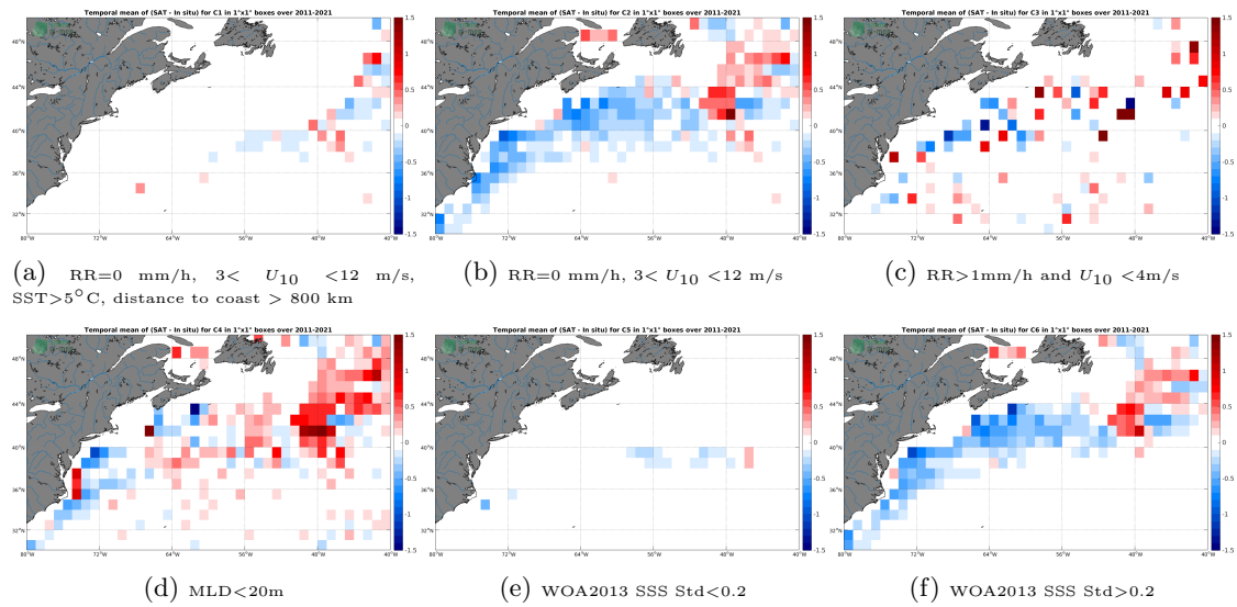
Figure 12: Temporal mean gridded over spatial boxes of size 1^\circ \times 1^\circ of \Delta SSS (SMAP SSS L4 OI v1 - 7day (IPRC) - Argo) for 6 different subdatasets corresponding to: RR=0 mm/h, 3 < U_{10} < 12 m/s, SST > 5°C, distance to coast > 800 km (a), RR=0 mm/h, 3 < U_{10} < 12 m/s (b), RR > 1mm/h and U_{10} < 4 m/s (c), MLD < 20m (d), WOA2013 SSS Std < 0.2 (e), WOA2013 SSS Std > 0.2 (f).
