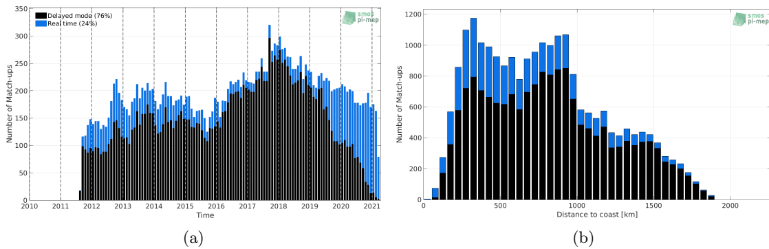
Figure 1: Number of match-ups between Argo and SMAP SSS L4 OI v1 - 7day (IPRC) SSS as a function of time (a) and as function of the distance to coast (b) over the Gulf Stream Pi-MEP region and for the full satellite product period.
