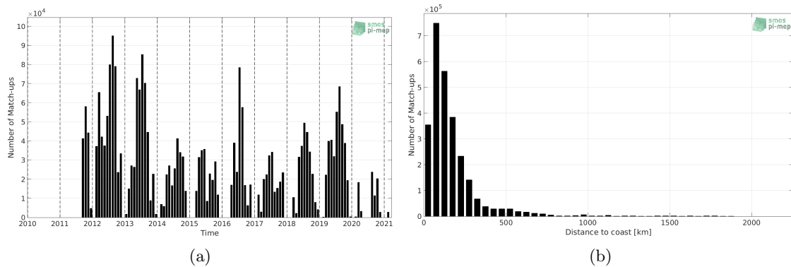
Figure 1: Number of match-ups between TSG (SAMOS) and SMAP SSS L4 OI v1 - Monthly (IPRC) SSS as a function of time (a) and as function of the distance to coast (b) over the Gulf Stream Pi-MEP region and for the full satellite product period.
