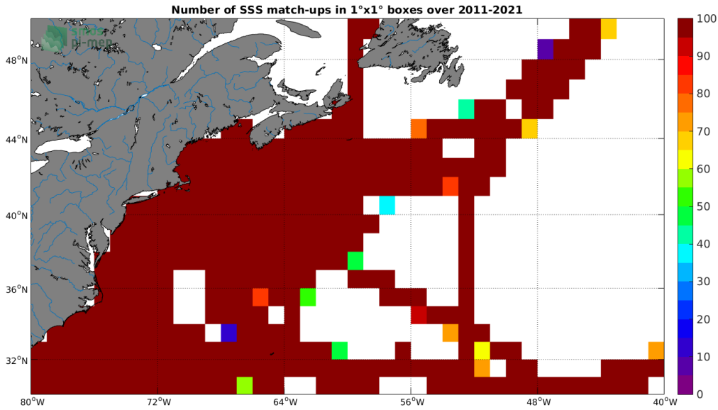
Figure 4: Number of SSS match-ups between TSG (SAMOS) SSS and the SMAP SSS L4 OI v1 - Monthly (IPRC) SSS product for the Gulf Stream Pi-MEP region over 1°x1° boxes and for the full satellite product period.
