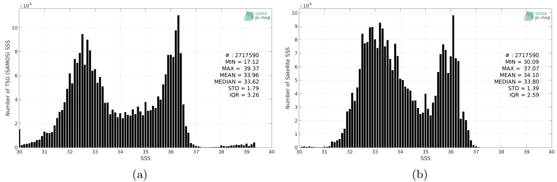
Figure 2: Histograms of SSS from TSG (SAMOS) (a) and SMAP SSS L4 OI v1 - Monthly (IPRC) (b) considering all match-up pairs per bins of 0.1 over the Gulf Stream Pi-MEP region and for the full satellite product period.
