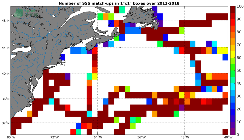
Figure 4: Number of SSS match-ups between TSG (GOSUD-Sailing-ship) SSS and the SMAP SSS L4 OI v1 - Monthly (IPRC) SSS product for the Gulf Stream Pi-MEP region over 1^\circ \times 1^\circ boxes and for the full satellite product period.
