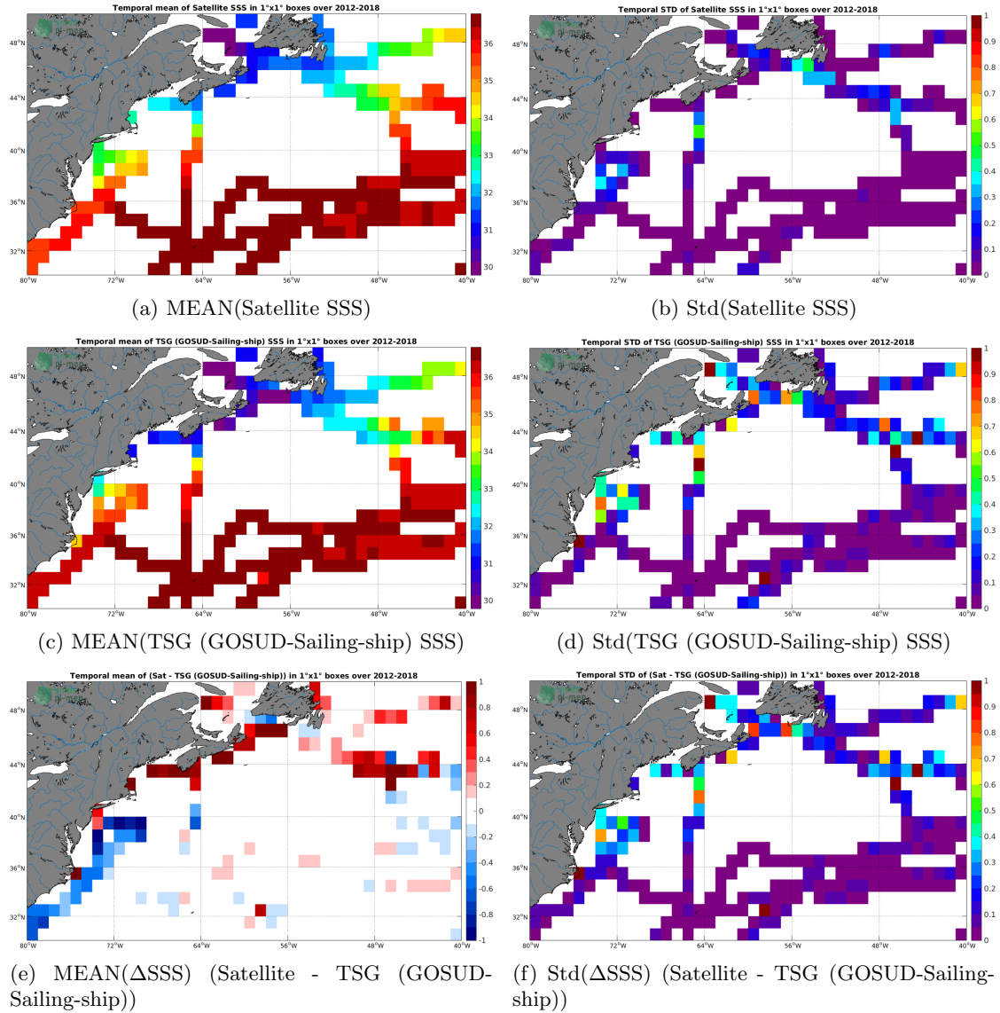
Figure 6: Temporal mean (left) and Std (right) of SSS from SMAP SSS L4 OI v1 - Monthly (IPRC) (top), TSG (GOSUD-Sailing-ship) (middle), and of \Delta SSS (Satellite - TSG (GOSUD-Sailing-ship)). Only match-up pairs are used to generate these maps.
