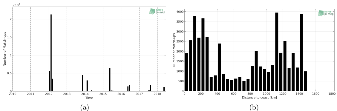
Figure 1: Number of match-ups between TSG (GOSUD-Sailing-ship) and SMAP SSS L4 OI v1 - Monthly (IPRC) SSS as a function of time (a) and as function of the distance to coast (b) over the Gulf Stream Pi-MEP region and for the full satellite product period.
