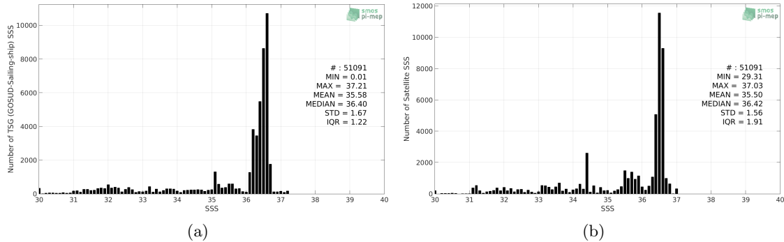
Figure 2: Histograms of SSS from TSG (GOSUD-Sailing-ship) (a) and SMAP SSS L4 OI v1 - Monthly (IPRC) (b) considering all match-up pairs per bins of 0.1 over the Gulf Stream Pi-MEP region and for the full satellite product period.
