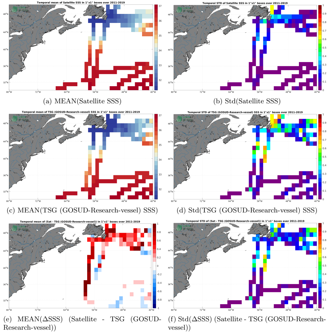
Figure 6: Temporal mean (left) and Std (right) of SSS from SMAP SSS L4 OI v1 - Monthly (IPRC) (top), TSG (GOSUD-Research-vessel) (middle), and of \Delta SSS (Satellite - TSG (GOSUD-Research-vessel)). Only match-up pairs are used to generate these maps.
