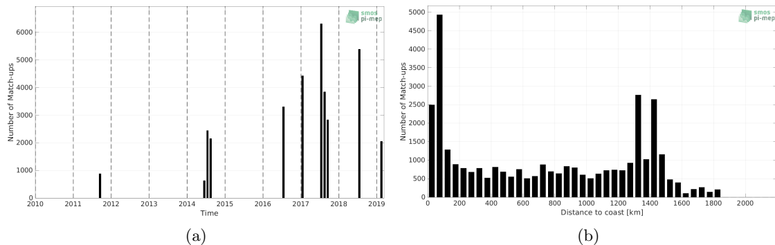
Figure 1: Number of match-ups between TSG (GOSUD-Research-vessel) and SMAP SSS L4 OI v1 - Monthly (IPRC) SSS as a function of time (a) and as function of the distance to coast (b) over the Gulf Stream Pi-MEP region and for the full satellite product period.
