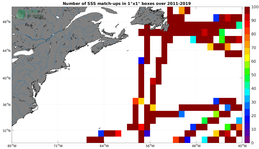
Figure 4: Number of SSS match-ups between TSG (GOSUD-Research-vessel) SSS and the SMAP SSS L4 OI v1 - Monthly (IPRC) SSS product for the Gulf Stream Pi-MEP region over 1^\circ \times 1^\circ boxes and for the full satellite product period.
