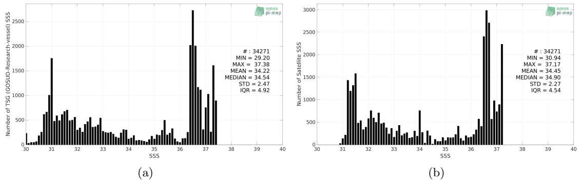
Figure 2: Histograms of SSS from TSG (GOSUD-Research-vessel) (a) and SMAP SSS L4 OI v1 - Monthly (IPRC) (b) considering all match-up pairs per bins of 0.1 over the Gulf Stream Pi-MEP region and for the full satellite product period.
