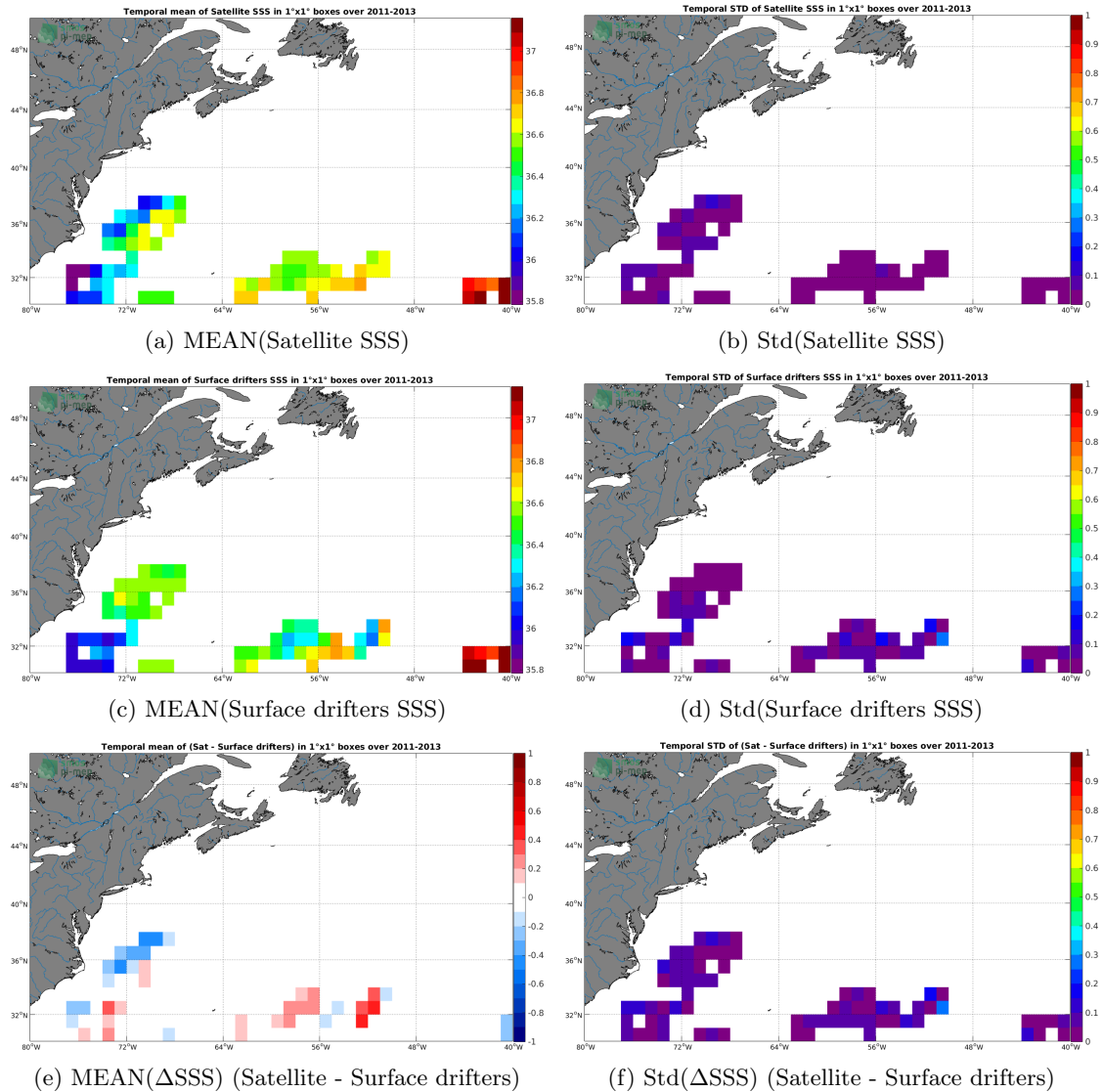
Figure 5: Temporal mean (left) and Std (right) of SSS from SMAP SSS L4 OI v1 - Monthly (IPRC) (top), Surface drifters (middle), and of \Delta SSS (Satellite - Surface drifters). Only match-up pairs are used to generate these maps.
