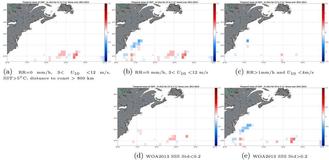
Figure 11: Temporal mean gridded over spatial boxes of size 1^{\circ}\times 1^{\circ} of \Delta\text{SSS} (SMAP SSS L4 OI v1 - Monthly (IPRC) - Surface drifters) for 5 different subdatasets corresponding to:RR=0 mm/h, 3 < U_{10} < 12 m/s, SST > 5^{\circ}\text{C} , distance to coast > 800 km (a), RR=0 mm/h, 3 < U_{10} < 12 m/s (b), RR > 1 mm/h and U_{10} < 4 m/s (c), WOA2013 SSS Std < 0.2 (d), WOA2013 SSS Std > 0.2 (e).
