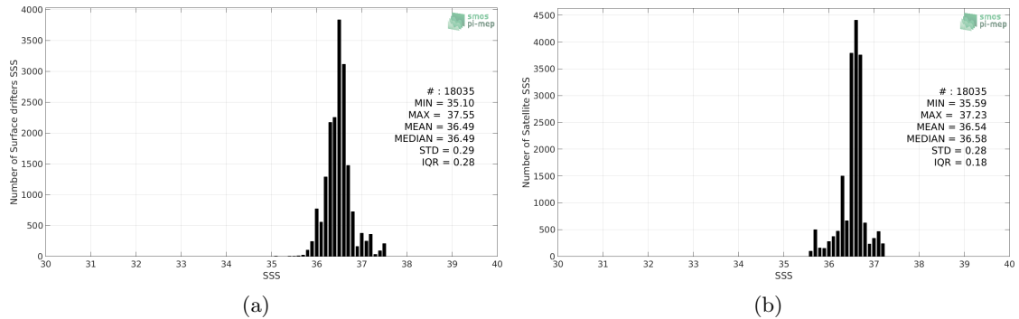
Figure 2: Histograms of SSS from Surface drifters (a) and SMAP SSS L4 OI v1 - Monthly (IPRC) (b) considering all match-up pairs per bins of 0.1 over the Gulf Stream Pi-MEP region and for the full satellite product period.
