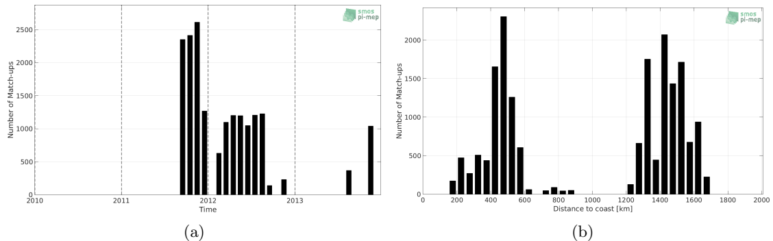
Figure 1: Number of match-ups between Surface drifters and SMAP SSS L4 OI v1 - Monthly (IPRC) SSS as a function of time (a) and as function of the distance to coast (b) over the Gulf Stream Pi-MEP region and for the full satellite product period.
