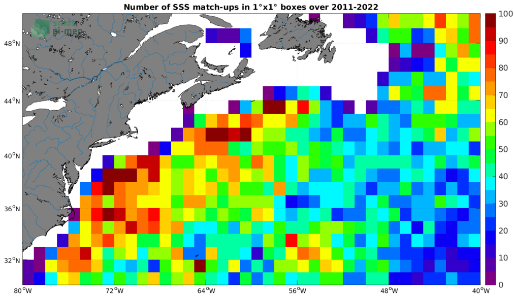
Figure 4: Number of SSS match-ups between Argo SSS and the SMAP SSS L4 OI v1 - Monthly (IPRC) SSS product for the Gulf Stream Pi-MEP region over 1^{\circ} \times 1^{\circ} boxes and for the full satellite product period.
