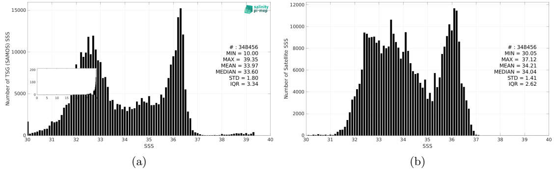
Figure 3: Histograms of SSS from TSG (SAMOS) (a) and SMAP SSS L4 OI v3 - Monthly (ESR) (b) considering all match-up pairs per bins of 0.1 over the Gulf Stream Pi-MEP region and for the full satellite product period.
