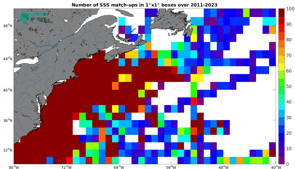
Figure 5: Number of SSS match-ups between TSG (SAMOS) SSS and the SMAP SSS L4 OI v3 - Monthly (ESR) SSS product for the Gulf Stream Pi-MEP region over 1^\circ \times 1^\circ boxes and for the full satellite product period.
