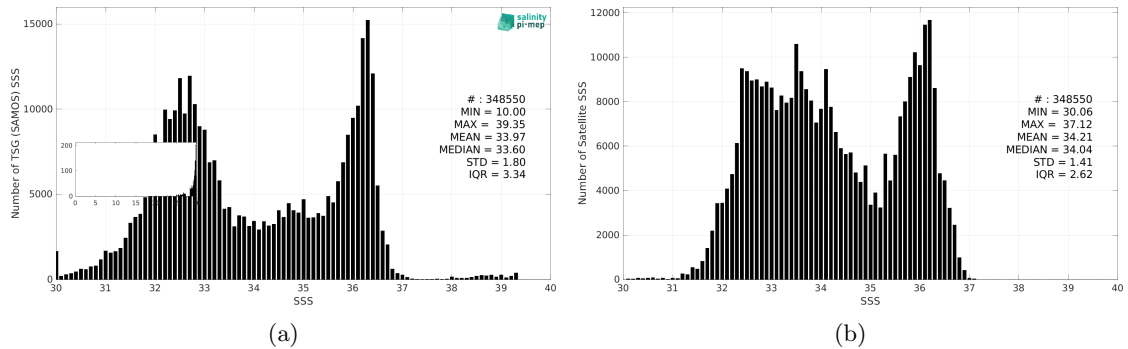
Figure 3: Histograms of SSS from TSG (SAMOS) (a) and SMAP SSS L4 OI v3 - Monthly (ESR) (b) considering all match-up pairs per bins of 0.1 over the Gulf Stream Pi-MEP region and for the full satellite product period.
