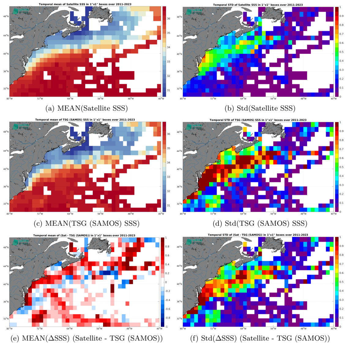
Figure 7: Temporal mean (left) and Std (right) of SSS from SMAP SSS L4 OI v3 - Monthly (ESR) (top), TSG (SAMOS) (middle), and of \Delta SSS (Satellite - TSG (SAMOS)). Only match-up pairs are used to generate these maps.
