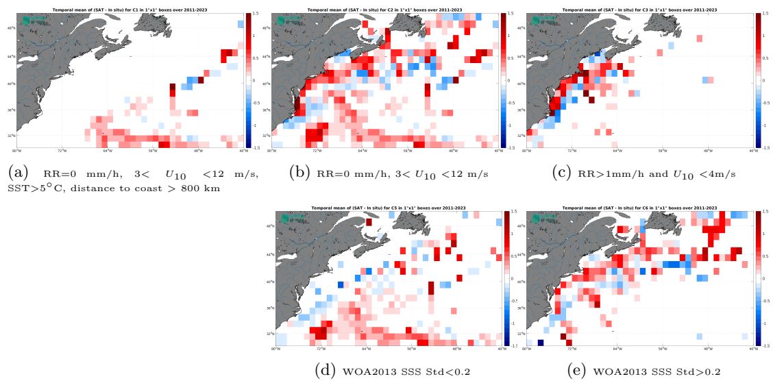
Figure 14: Temporal mean gridded over spatial boxes of size 1^\circ \times 1^\circ of \Delta SSS (SMAP SSS L4 OI v3 - Monthly (ESR) - TSG (SAMOS)) for 5 different subdatasets corresponding to:RR=0 mm/h, 3 < U_{10} < 12 m/s, SST >5^\circ C, distance to coast > 800 km (a), RR=0 mm/h, 3 < U_{10} < 12 m/s (b), RR >1 mm/h and U_{10} < 4 m/s (c), WOA2013 SSS Std <0.2 (d), WOA2013 SSS Std >0.2 (e).
