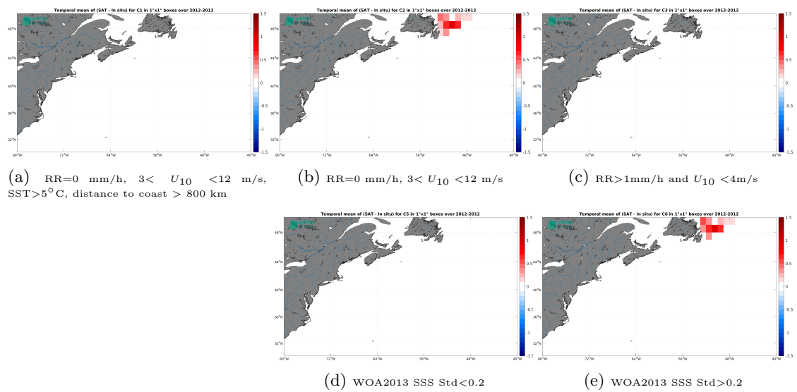
Figure 14: Temporal mean gridded over spatial boxes of size 1^\circ \times 1^\circ of \Delta SSS (SMAP SSS L4 OI v3 - Monthly (ESR) - TSG (CSIC-UTM)) for 5 different subdatasets corresponding to:RR=0 mm/h, 3 < U_{10} < 12 m/s, SST > 5°C, distance to coast > 800 km (a), RR=0 mm/h, 3 < U_{10} < 12 m/s (b), RR > 1mm/h and U_{10} < 4 m/s (c), WOA2013 SSS Std < 0.2 (d), WOA2013 SSS Std > 0.2 (e).
