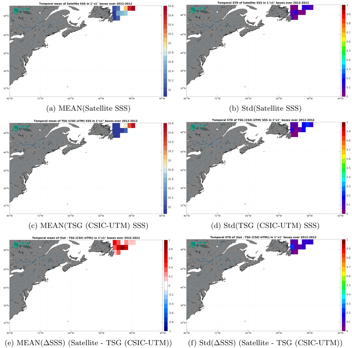
Figure 7: Temporal mean (left) and Std (right) of SSS from SMAP SSS L4 OI v3 - Monthly (ESR) (top), TSG (CSIC-UTM) (middle), and of \Delta SSS (Satellite - TSG (CSIC-UTM)). Only match-up pairs are used to generate these maps.
