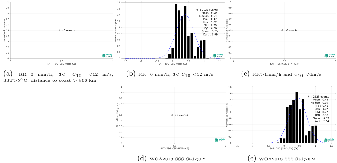
Figure 15: Normalized histogram of \Delta SSS (SMAP SSS L4 OI v3 - Monthly (ESR) - TSG (CSIC-UTM)) for 5 different subdatasets corresponding to: RR=0 mm/h, 3 < U_{10} < 12 m/s, SST > 5°C, distance to coast > 800 km (a), RR=0 mm/h, 3 < U_{10} < 12 m/s (b), RR > 1mm/h and U_{10} < 4 m/s (c), WOA2013 SSS Std < 0.2 (d), WOA2013 SSS Std > 0.2 (e).
