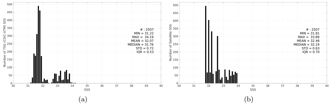
Figure 3: Histograms of SSS from TSG (CSIC-UTM) (a) and SMAP SSS L4 OI v3 - Monthly (ESR) (b) considering all match-up pairs per bins of 0.1 over the Gulf Stream Pi-MEP region and for the full satellite product period.
