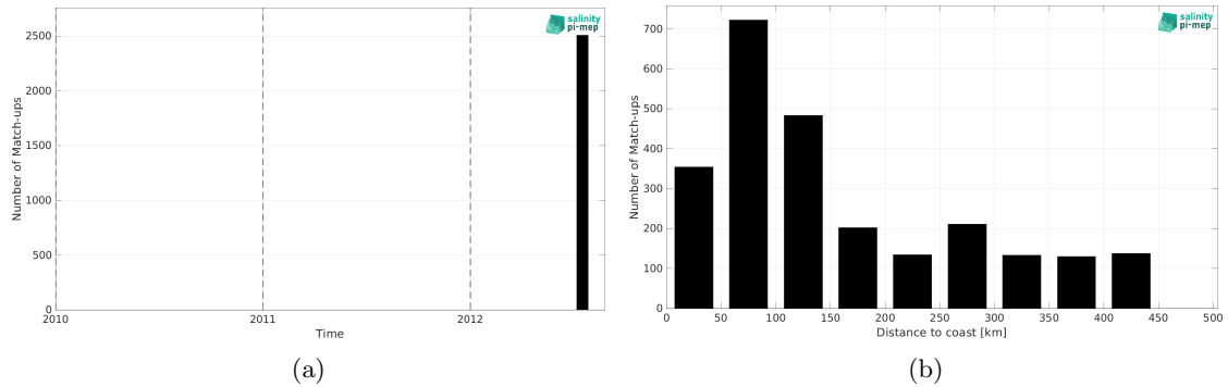
Figure 2: Number of match-ups between TSG (CSIC-UTM) and SMAP SSS L4 OI v3 - Monthly (ESR) SSS as a function of time (a) and as function of the distance to coast (b) over the Gulf Stream Pi-MEP region and for the full satellite product period.
