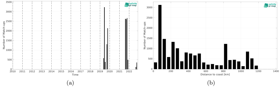
Figure 2: Number of match-ups between Saildrone and SMAP SSS L4 OI v3 - Monthly (ESR) SSS as a function of time (a) and as function of the distance to coast (b) over the Gulf Stream Pi-MEP region and for the full satellite product period.
