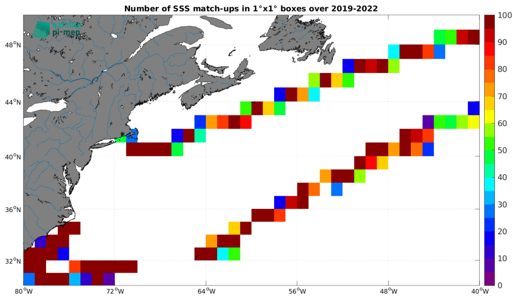
Figure 5: Number of SSS match-ups between Saildrone SSS and the SMAP SSS L4 OI v3 - Monthly (ESR) SSS product for the Gulf Stream Pi-MEP region over 1^\circ \times 1^\circ boxes and for the full satellite product period.
