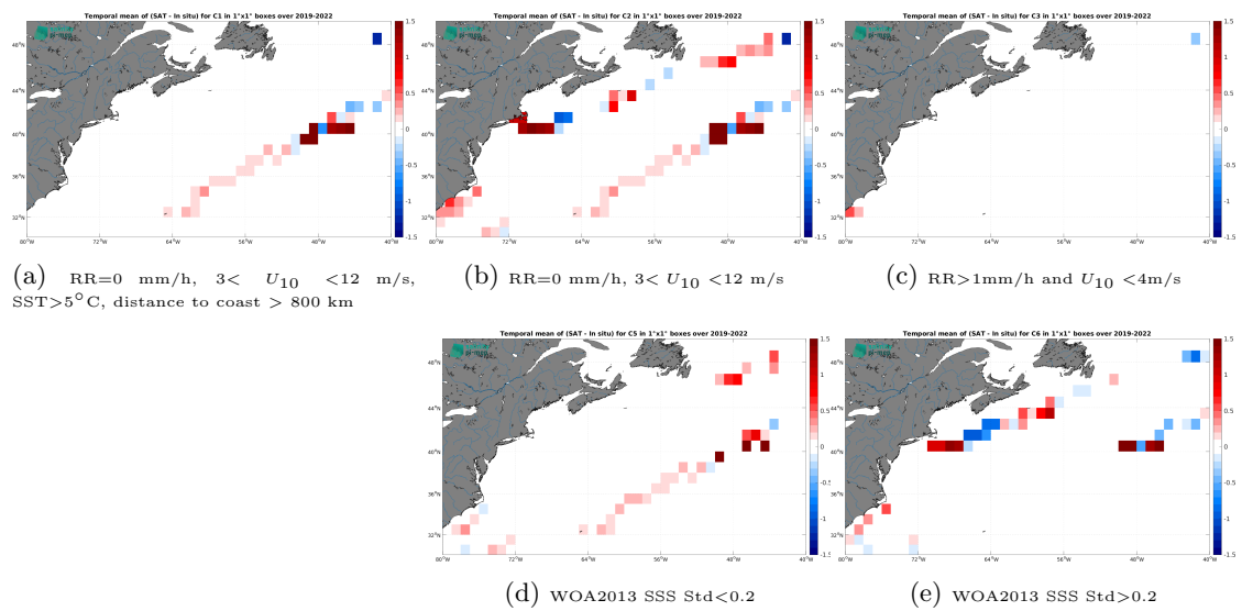
Figure 14: Temporal mean gridded over spatial boxes of size 1^\circ \times 1^\circ of \Delta SSS (SMAP SSS L4 OI v3 - Monthly (ESR) - Saildrone) for 5 different subdatasets corresponding to:RR=0 mm/h, 3 < U_{10} < 12 m/s, SST>5°C, distance to coast > 800 km (a), RR=0 mm/h, 3 < U_{10} < 12 m/s (b), RR>1mm/h and U_{10} < 4 m/s (c), WOA2013 SSS Std<0.2 (d), WOA2013 SSS Std>0.2 (e).
