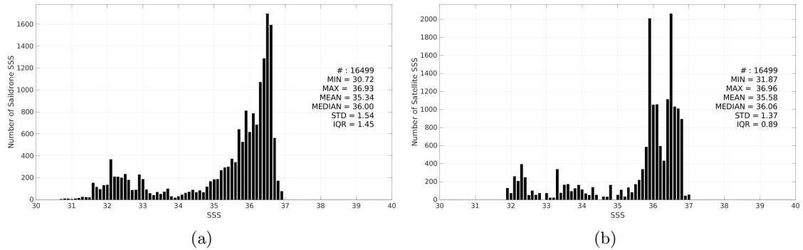
Figure 3: Histograms of SSS from Saildrone (a) and SMAP SSS L4 OI v3 - Monthly (ESR) (b) considering all match-up pairs per bins of 0.1 over the Gulf Stream Pi-MEP region and for the full satellite product period.
