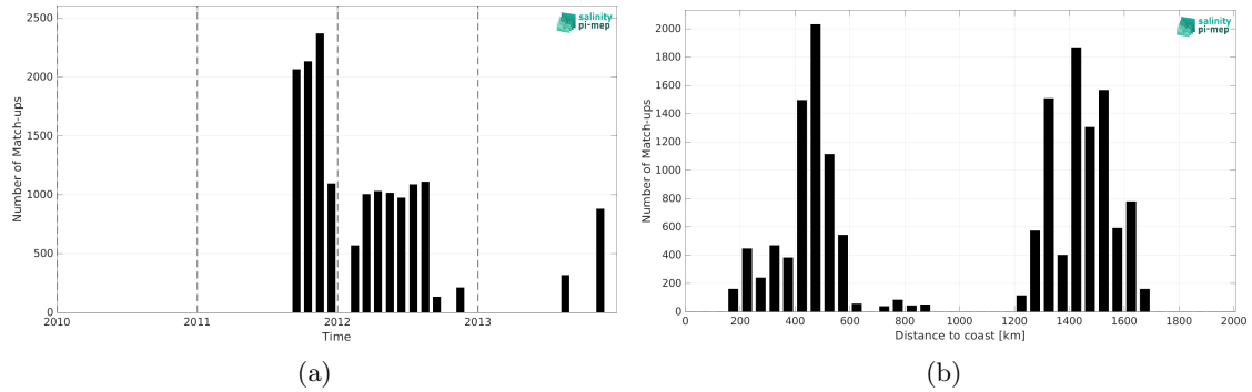
Figure 2: Number of match-ups between Surface drifters and SMAP SSS L4 OI v3 - Monthly (ESR) SSS as a function of time (a) and as function of the distance to coast (b) over the Gulf Stream Pi-MEP region and for the full satellite product period.
