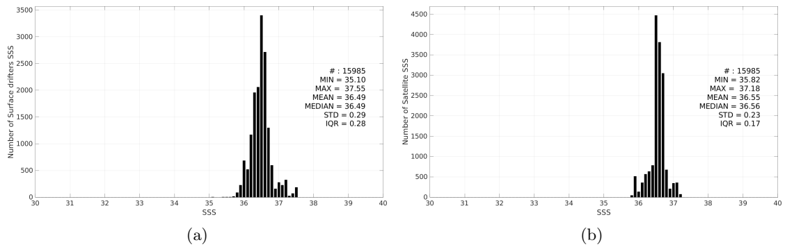
Figure 3: Histograms of SSS from Surface drifters (a) and SMAP SSS L4 OI v3 - Monthly (ESR) (b) considering all match-up pairs per bins of 0.1 over the Gulf Stream Pi-MEP region and for the full satellite product period.
