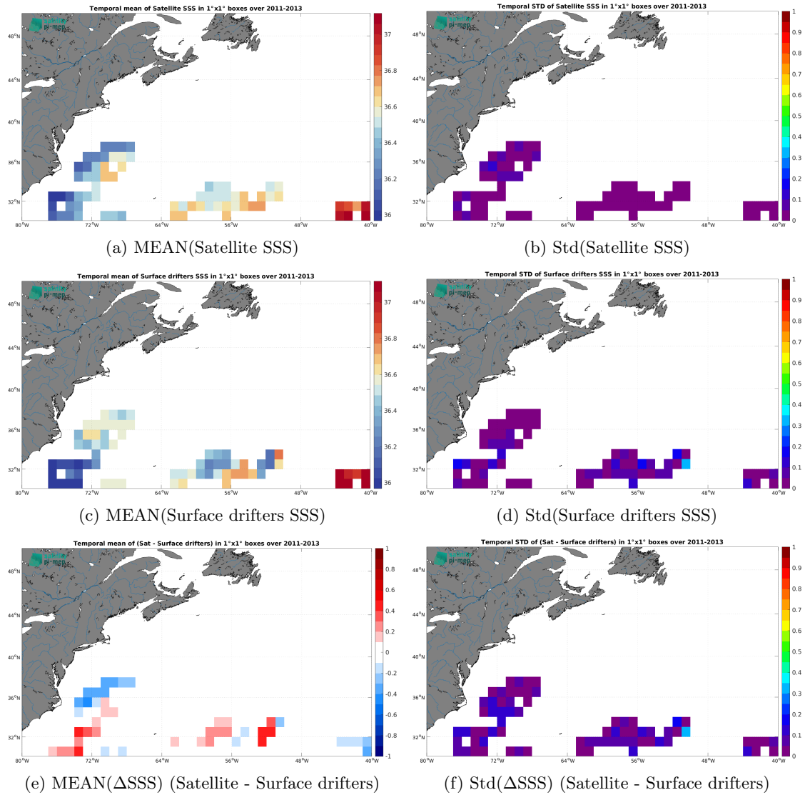
Figure 6: Temporal mean (left) and Std (right) of SSS from SMAP SSS L4 OI v3 - Monthly (ESR) (top), Surface drifters (middle), and of \Delta SSS (Satellite - Surface drifters). Only match-up pairs are used to generate these maps.
