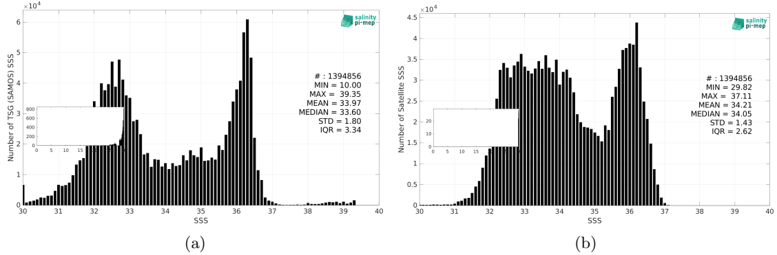
Figure 3: Histograms of SSS from TSG (SAMOS) (a) and SMAP SSS L4 OI v3 - Daily (ESR) (b) considering all match-up pairs per bins of 0.1 over the Gulf Stream Pi-MEP region and for the full satellite product period.
