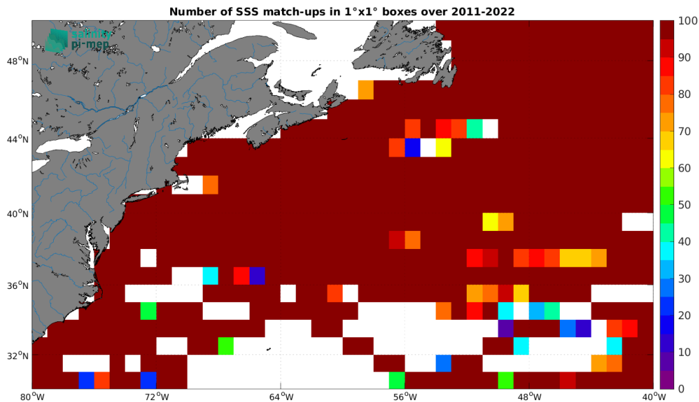
Figure 5: Number of SSS match-ups between TSG (LEGOS-DM) SSS and the SMAP SSS L4 OI v3 - Daily (ESR) SSS product for the Gulf Stream Pi-MEP region over 1^\circ \times 1^\circ boxes and for the full satellite product period.
