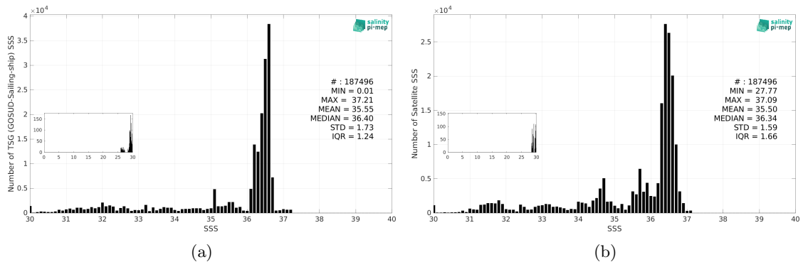
Figure 3: Histograms of SSS from TSG (GOSUD-Sailing-ship) (a) and SMAP SSS L4 OI v3 - Daily (ESR) (b) considering all match-up pairs per bins of 0.1 over the Gulf Stream Pi-MEP region and for the full satellite product period.
