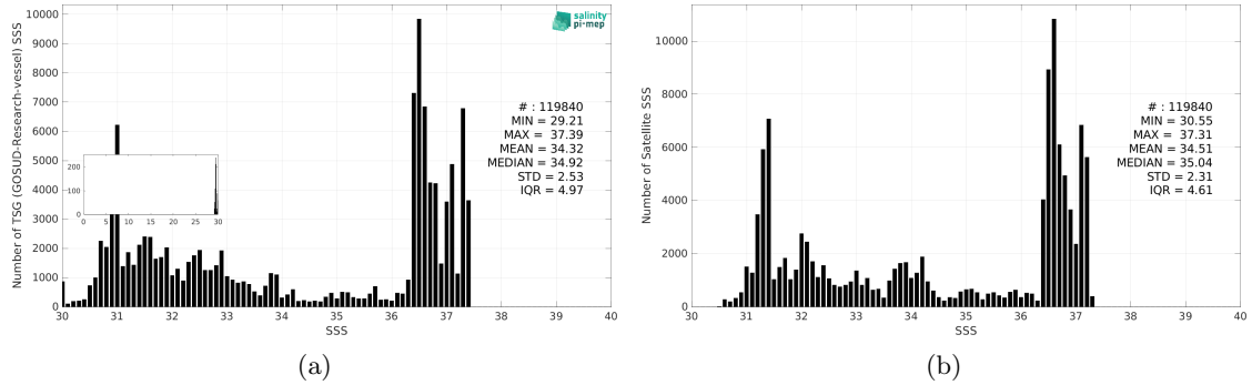
Figure 3: Histograms of SSS from TSG (GOSUD-Research-vessel) (a) and SMAP SSS L4 OI v3 - Daily (ESR) (b) considering all match-up pairs per bins of 0.1 over the Gulf Stream Pi-MEP region and for the full satellite product period.
