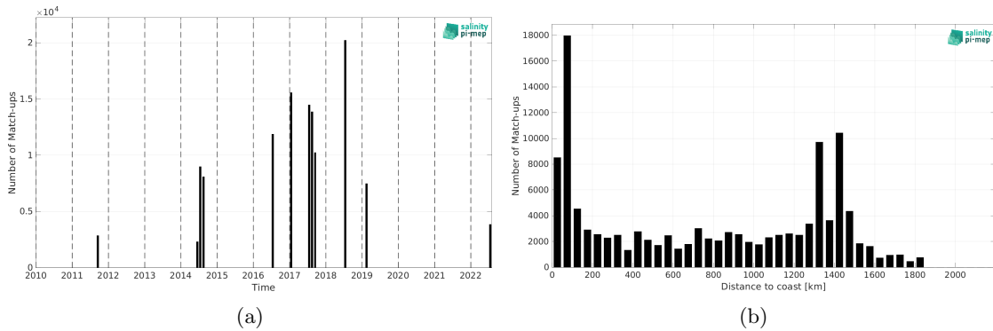
Figure 2: Number of match-ups between TSG (GOSUD-Research-vessel) and SMAP SSS L4 OI v3 - Daily (ESR) SSS as a function of time (a) and as function of the distance to coast (b) over the Gulf Stream Pi-MEP region and for the full satellite product period.
