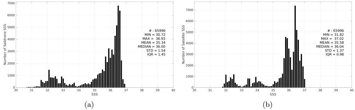
Figure 3: Histograms of SSS from Saildrone (a) and SMAP SSS L4 OI v3 - Daily (ESR) (b) considering all match-up pairs per bins of 0.1 over the Gulf Stream Pi-MEP region and for the full satellite product period.
