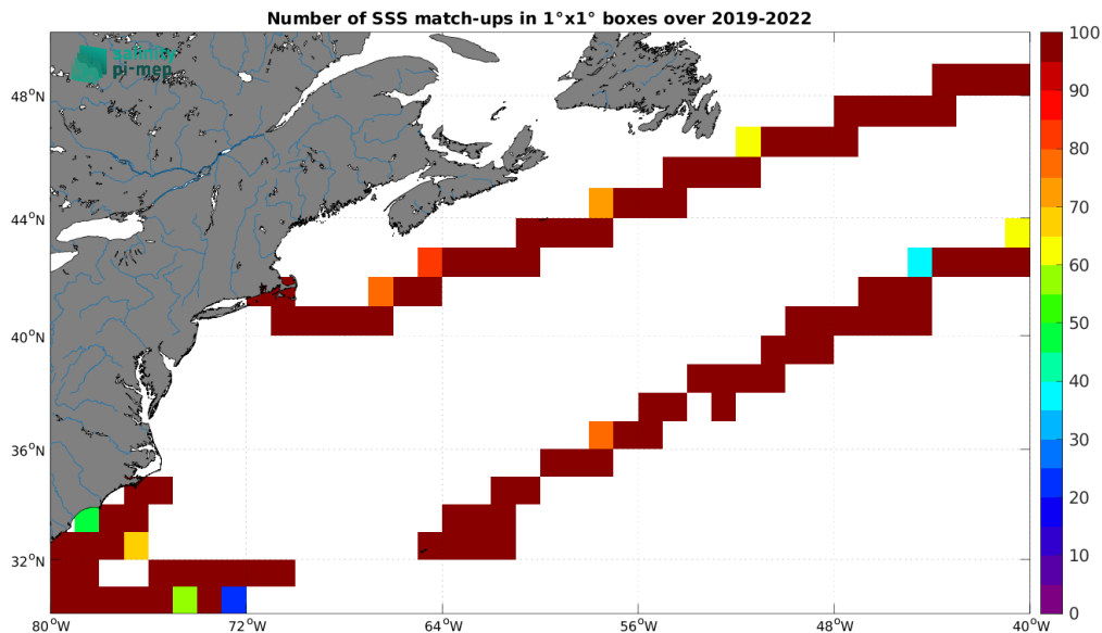
Figure 5: Number of SSS match-ups between Saildrone SSS and the SMAP SSS L4 OI v3 - Daily (ESR) SSS product for the Gulf Stream Pi-MEP region over 1^\circ \times 1^\circ boxes and for the full satellite product period.
