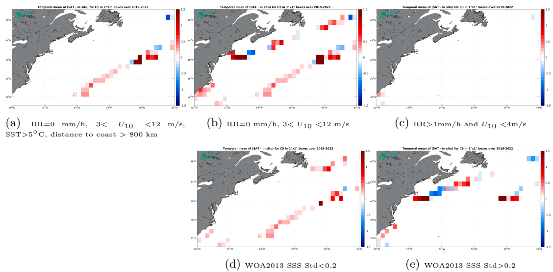
Figure 14: Temporal mean gridded over spatial boxes of size 1^\circ \times 1^\circ of \Delta SSS (SMAP SSS L4 OI v3 - Daily (ESR) - Saildrone) for 5 different subdatasets corresponding to:RR=0 mm/h, 3 < U_{10} < 12 m/s, SST>5°C, distance to coast > 800 km (a), RR=0 mm/h, 3 < U_{10} < 12 m/s (b), RR>1mm/h and U_{10} < 4 m/s (c), WOA2013 SSS Std<0.2 (d), WOA2013 SSS Std>0.2 (e).
