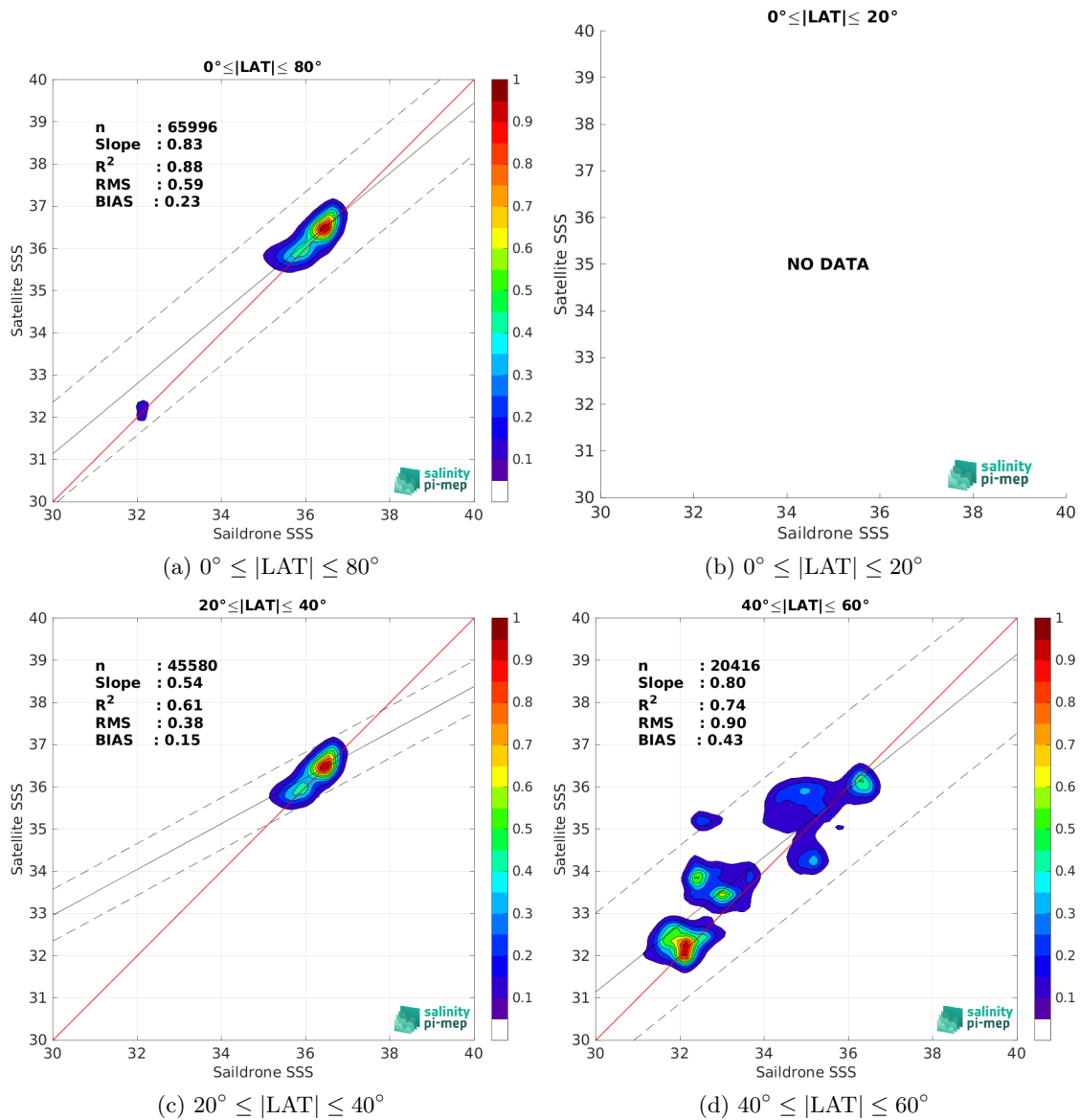
Figure 10: Contour maps of the concentration of SMAP SSS L4 OI v3 - Daily (ESR) SSS (y-axis) versus Saildrone SSS (x-axis) at match-up pairs for different latitude bands. For each plot, the red line shows x=y . The black thin and dashed lines indicate a linear fit through the data cloud and the \pm 95\% confidence levels, respectively. The number match-up pairs n , the slope and R^2 coefficient of the linear fit, the root mean square (RMS) and the mean bias between satellite and in situ data are indicated for each latitude band in each plots.
