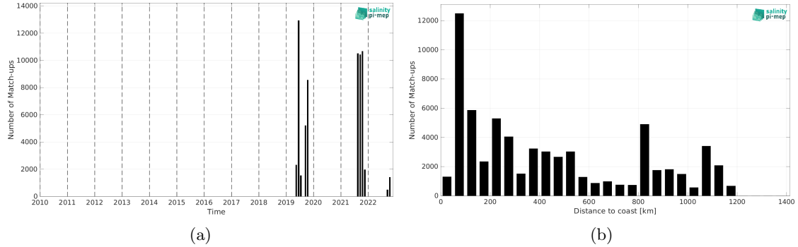
Figure 2: Number of match-ups between Saildrone and SMAP SSS L4 OI v3 - Daily (ESR) SSS as a function of time (a) and as function of the distance to coast (b) over the Gulf Stream Pi-MEP region and for the full satellite product period.
