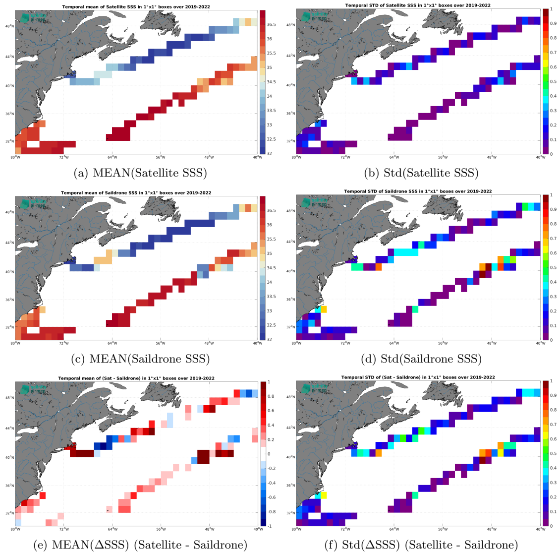
Figure 7: Temporal mean (left) and Std (right) of SSS from SMAP SSS L4 OI v3 - Daily (ESR) (top), Saildrone (middle), and of \Delta SSS (Satellite - Saildrone). Only match-up pairs are used to generate these maps.
