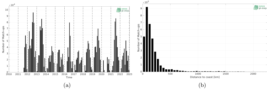
Figure 1: Number of match-ups between TSG (SAMOS) and SMAP SSS L4 OI v2 - 7 Days (ESR) SSS as a function of time (a) and as function of the distance to coast (b) over the Gulf Stream Pi-MEP region and for the full satellite product period.
