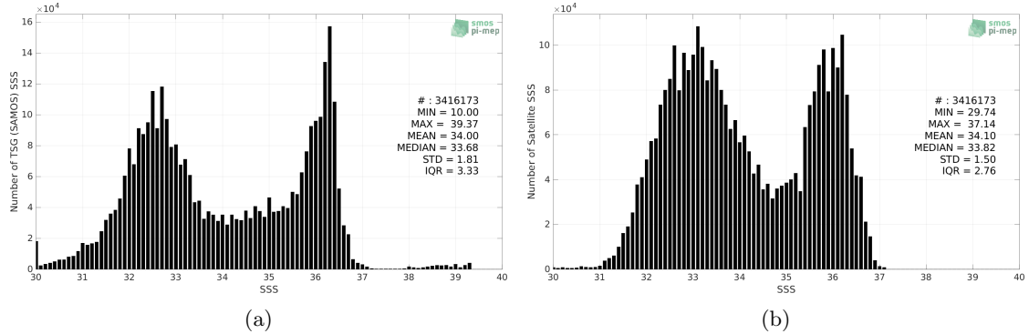
Figure 2: Histograms of SSS from TSG (SAMOS) (a) and SMAP SSS L4 OI v2 - 7 Days (ESR) (b) considering all match-up pairs per bins of 0.1 over the Gulf Stream Pi-MEP region and for the full satellite product period.
