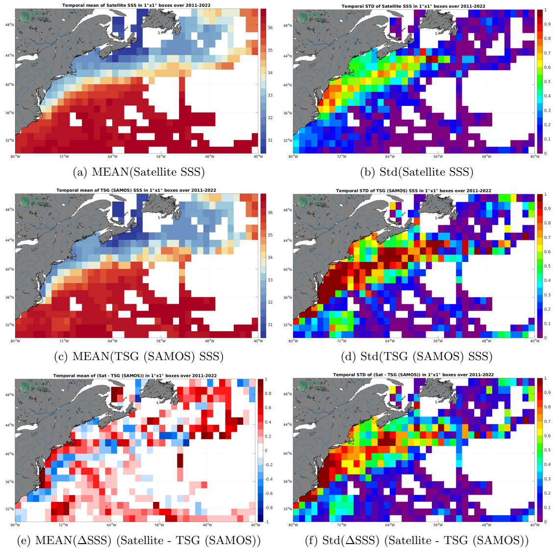
Figure 6: Temporal mean (left) and Std (right) of SSS from SMAP SSS L4 OI v2 - 7 Days (ESR) (top), TSG (SAMOS) (middle), and of \Delta SSS (Satellite - TSG (SAMOS)). Only match-up pairs are used to generate these maps.
