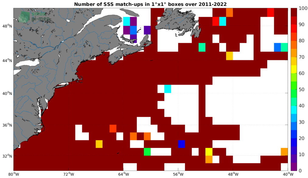
Figure 4: Number of SSS match-ups between TSG (SAMOS) SSS and the SMAP SSS L4 OI v2 - 7 Days (ESR) SSS product for the Gulf Stream Pi-MEP region over 1^\circ \times 1^\circ boxes and for the full satellite product period.
