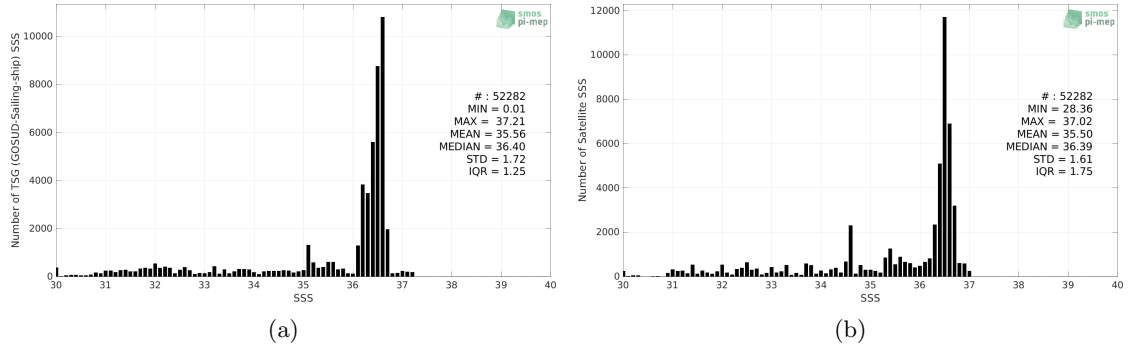
Figure 2: Histograms of SSS from TSG (GOSUD-Sailing-ship) (a) and SMAP SSS L4 OI v2 - 7 Days (ESR) (b) considering all match-up pairs per bins of 0.1 over the Gulf Stream Pi-MEP region and for the full satellite product period.
