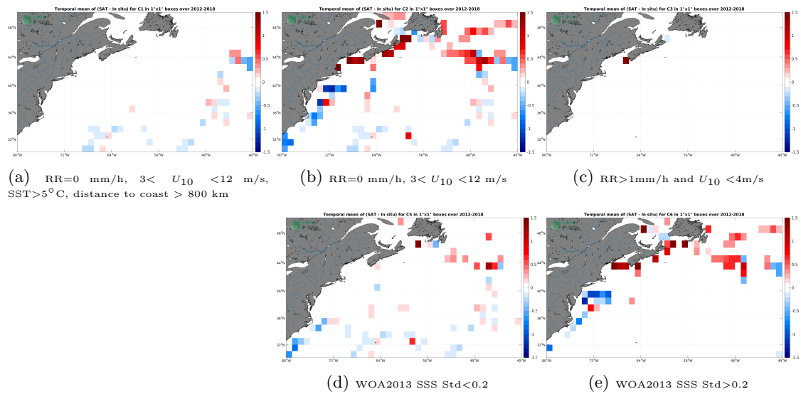
Figure 12: Temporal mean gridded over spatial boxes of size 1^\circ \times 1^\circ of \Delta SSS (SMAP SSS L4 OI v2 - 7 Days (ESR) - TSG (GOSUD-Sailing-ship)) for 5 different subdatasets corresponding to:RR=0 mm/h, 3 < U_{10} < 12 m/s, SST >5^\circ C, distance to coast > 800 km (a), RR=0 mm/h, 3 < U_{10} < 12 m/s (b), RR >1 mm/h and U_{10} < 4 m/s (c), WOA2013 SSS Std <0.2 (d), WOA2013 SSS Std >0.2 (e).
