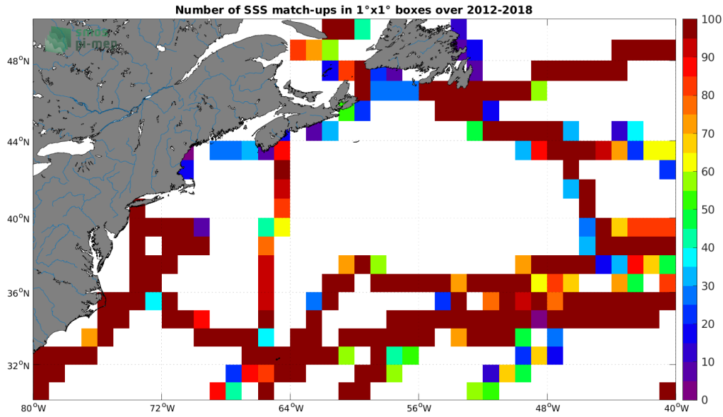
Figure 4: Number of SSS match-ups between TSG (GOSUD-Sailing-ship) SSS and the SMAP SSS L4 OI v2 - 7 Days (ESR) SSS product for the Gulf Stream Pi-MEP region over 1^\circ \times 1^\circ boxes and for the full satellite product period.
