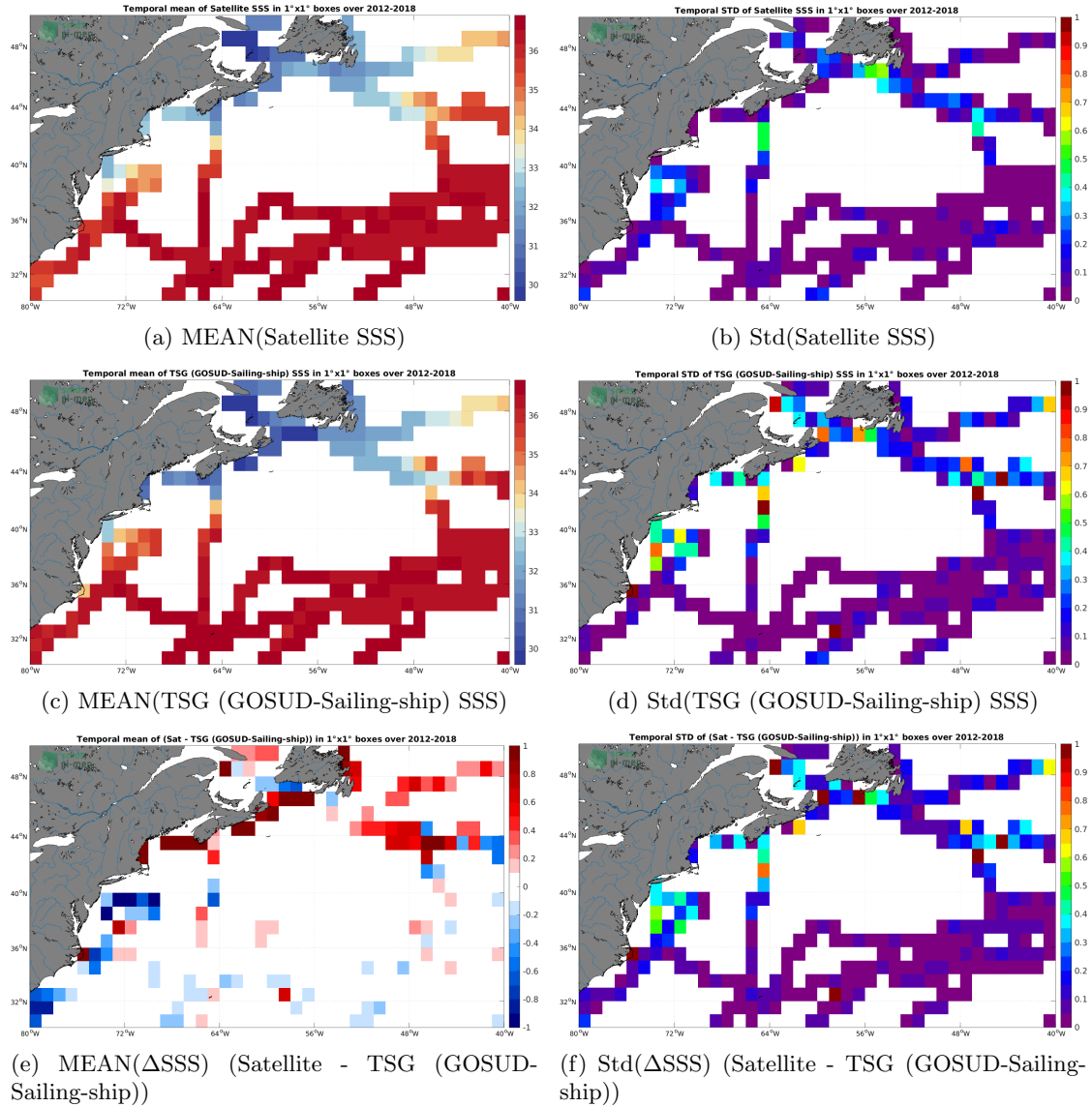
Figure 6: Temporal mean (left) and Std (right) of SSS from SMAP SSS L4 OI v2 - 7 Days (ESR) (top), TSG (GOSUD-Sailing-ship) (middle), and of \Delta SSS (Satellite - TSG (GOSUD-Sailing-ship)). Only match-up pairs are used to generate these maps.
