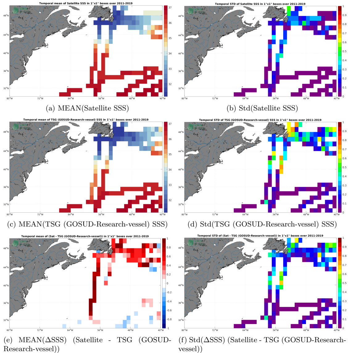
Figure 6: Temporal mean (left) and Std (right) of SSS from SMAP SSS L4 OI v2 - 7 Days (ESR) (top), TSG (GOSUD-Research-vessel) (middle), and of \Delta SSS (Satellite - TSG (GOSUD-Research-vessel)). Only match-up pairs are used to generate these maps.
