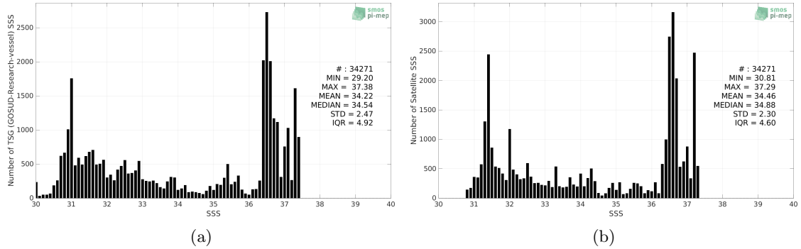
Figure 2: Histograms of SSS from TSG (GOSUD-Research-vessel) (a) and SMAP SSS L4 OI v2 - 7 Days (ESR) (b) considering all match-up pairs per bins of 0.1 over the Gulf Stream Pi-MEP region and for the full satellite product period.
