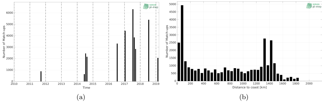
Figure 1: Number of match-ups between TSG (GOSUD-Research-vessel) and SMAP SSS L4 OI v2 - 7 Days (ESR) SSS as a function of time (a) and as function of the distance to coast (b) over the Gulf Stream Pi-MEP region and for the full satellite product period.
