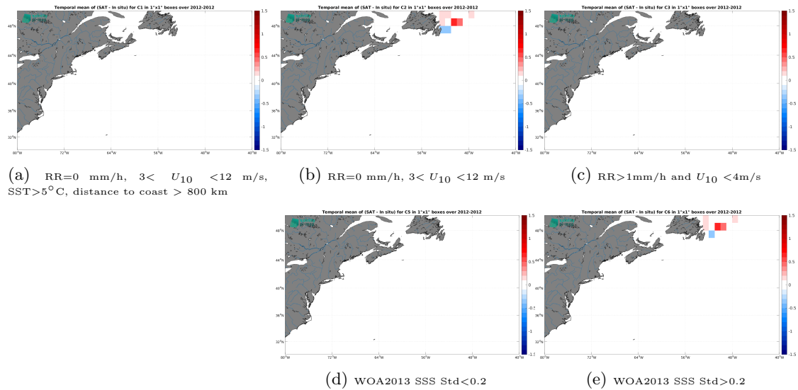
Figure 12: Temporal mean gridded over spatial boxes of size 1^{\circ}\times 1^{\circ} of \Delta\text{SSS} (SMAP SSS L4 OI v2 - 7 Days (ESR) - TSG (CSIC-UTM)) for 5 different subdatasets corresponding to:RR=0 mm/h, 3 < U_{10} < 12 m/s, SST >5^{\circ}\text{C} , distance to coast > 800 km (a), RR=0 mm/h, 3 < U_{10} < 12 m/s (b), RR >1 mm/h and U_{10} < 4 m/s (c), WOA2013 SSS Std <0.2 (d), WOA2013 SSS Std >0.2 (e).
