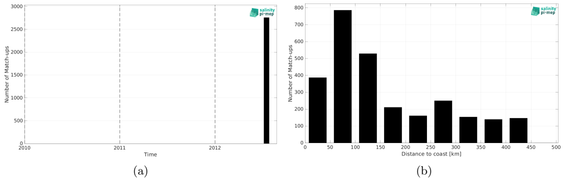
Figure 1: Number of match-ups between TSG (CSIC-UTM) and SMAP SSS L4 OI v2 - 7 Days (ESR) SSS as a function of time (a) and as function of the distance to coast (b) over the Gulf Stream Pi-MEP region and for the full satellite product period.
