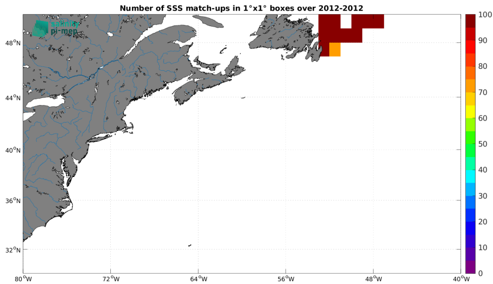
Figure 4: Number of SSS match-ups between TSG (CSIC-UTM) SSS and the SMAP SSS L4 OI v2 - 7 Days (ESR) SSS product for the Gulf Stream Pi-MEP region over 1^\circ \times 1^\circ boxes and for the full satellite product period.
