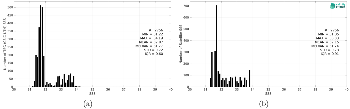
Figure 2: Histograms of SSS from TSG (CSIC-UTM) (a) and SMAP SSS L4 OI v2 - 7 Days (ESR) (b) considering all match-up pairs per bins of 0.1 over the Gulf Stream Pi-MEP region and for the full satellite product period.
