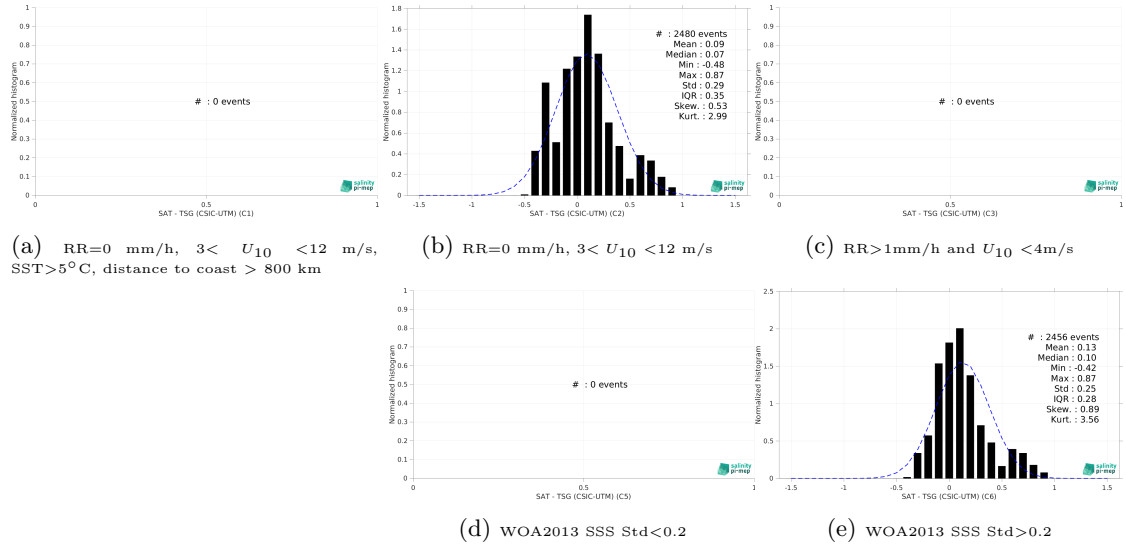
Figure 13: Normalized histogram of \Delta SSS (SMAP SSS L4 OI v2 - 7 Days (ESR) - TSG (CSIC-UTM)) for 5 different subdatasets corresponding to: RR=0 mm/h, 3 < U_{10} < 12 m/s, SST > 5°C, distance to coast > 800 km (a), RR=0 mm/h, 3 < U_{10} < 12 m/s (b), RR > 1mm/h and U_{10} < 4 m/s (c), WOA2013 SSS Std < 0.2 (d), WOA2013 SSS Std > 0.2 (e).
