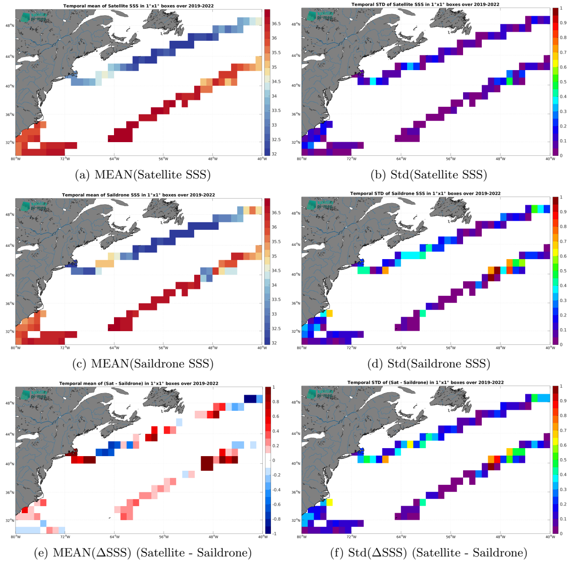
Figure 6: Temporal mean (left) and Std (right) of SSS from SMAP SSS L4 OI v2 - 7 Days (ESR) (top), Saildrone (middle), and of \Delta SSS (Satellite - Saildrone). Only match-up pairs are used to generate these maps.
