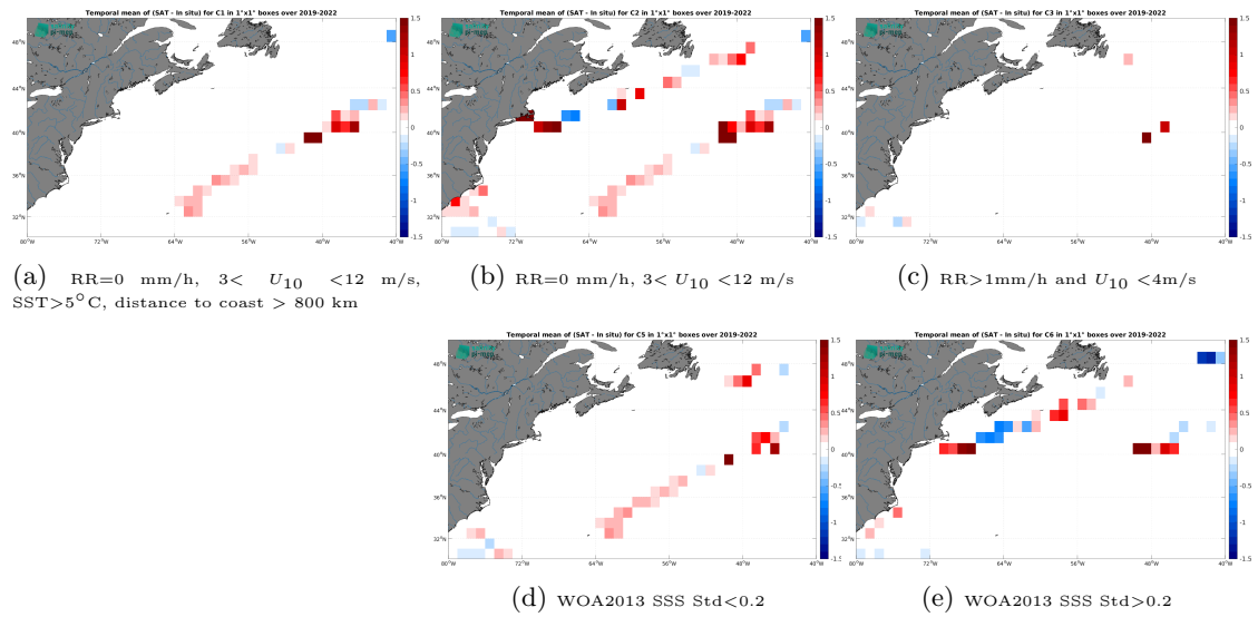
Figure 12: Temporal mean gridded over spatial boxes of size 1^\circ \times 1^\circ of \Delta SSS (SMAP SSS L4 OI v2 - 7 Days (ESR) - Sairdrone) for 5 different subdatasets corresponding to:RR=0 mm/h, 3 < U_{10} < 12 m/s, SST >5^\circ C, distance to coast > 800 km (a), RR=0 mm/h, 3 < U_{10} < 12 m/s (b), RR >1 mm/h and U_{10} < 4 m/s (c), WOA2013 SSS Std <0.2 (d), WOA2013 SSS Std >0.2 (e).
