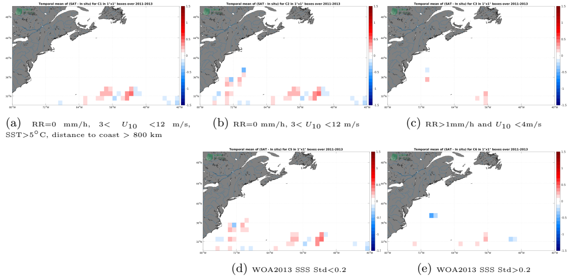
Figure 11: Temporal mean gridded over spatial boxes of size 1^{\circ}\times 1^{\circ} of \Delta\text{SSS} (SMAP SSS L4 OI v2 - 7 Days (ESR) - Surface drifters) for 5 different subdatasets corresponding to:RR=0 mm/h, 3 < U_{10} < 12 m/s, SST > 5^{\circ}\text{C} , distance to coast > 800 km (a), RR=0 mm/h, 3 < U_{10} < 12 m/s (b), RR > 1 mm/h and U_{10} < 4 m/s (c), WOA2013 SSS Std < 0.2 (d), WOA2013 SSS Std > 0.2 (e).
