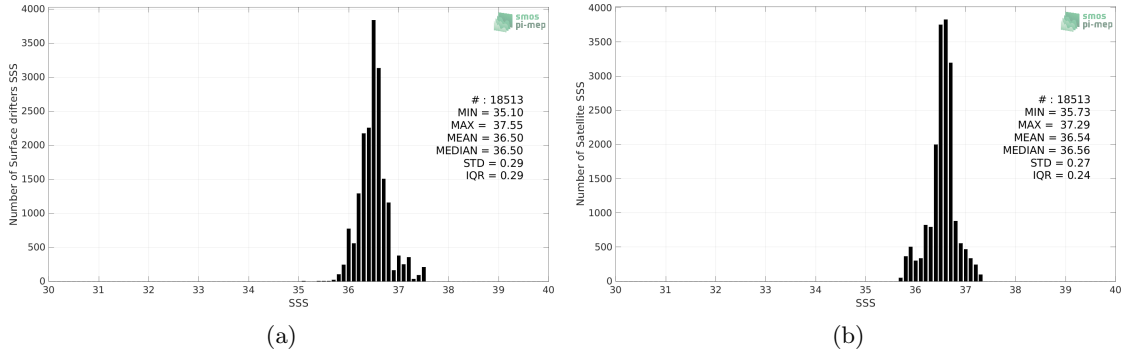
Figure 2: Histograms of SSS from Surface drifters (a) and SMAP SSS L4 OI v2 - 7 Days (ESR) (b) considering all match-up pairs per bins of 0.1 over the Gulf Stream Pi-MEP region and for the full satellite product period.
