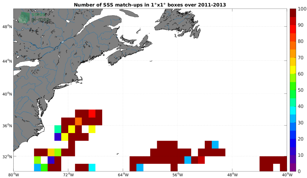
Figure 3: Number of SSS match-ups between Surface drifters SSS and the SMAP SSS L4 OI v2 - 7 Days (ESR) SSS product for the Gulf Stream Pi-MEP region over 1^\circ \times 1^\circ boxes and for the full satellite product period.
