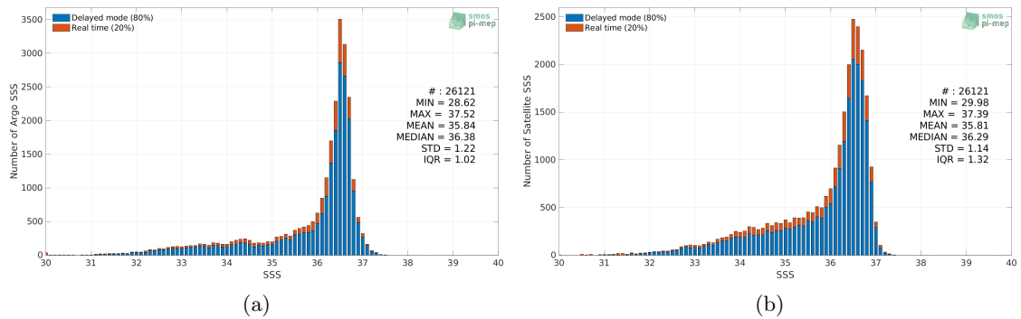
Figure 2: Histograms of SSS from Argo (a) and SMAP SSS L4 OI v2 - 7 Days (ESR) (b) considering all match-up pairs per bins of 0.1 over the Gulf Stream Pi-MEP region and for the full satellite product period.
