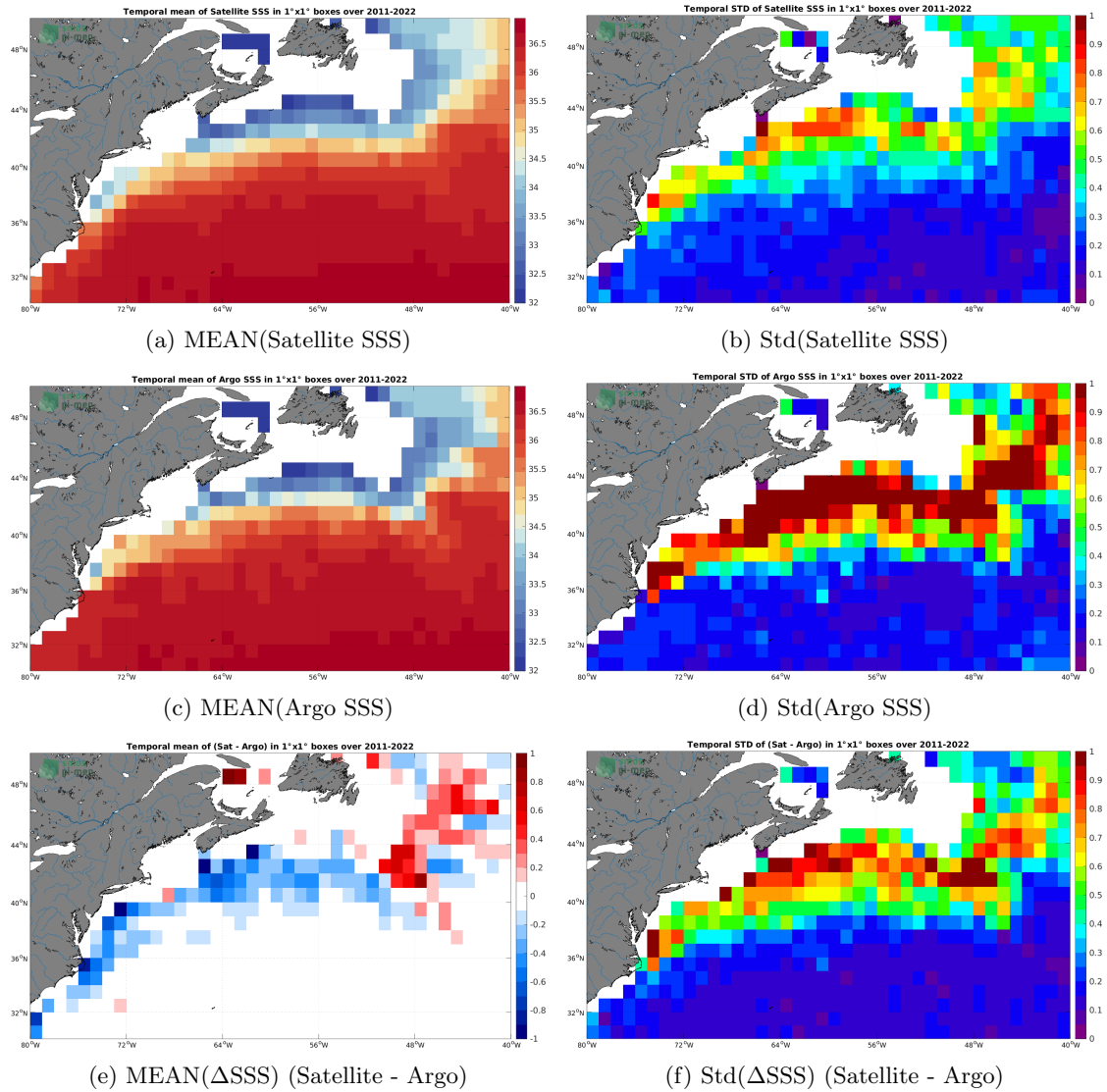
Figure 6: Temporal mean (left) and Std (right) of SSS from SMAP SSS L4 OI v2 - 7 Days (ESR) (top), Argo (middle), and of \Delta SSS (Satellite - Argo). Only match-up pairs are used to generate these maps.
