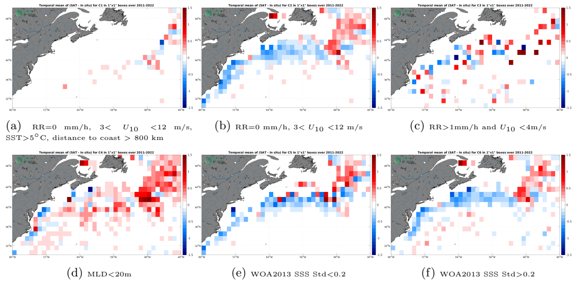
Figure 12: Temporal mean gridded over spatial boxes of size 1^\circ \times 1^\circ of \Delta SSS (SMAP SSS L4 OI v2 - 7 Days (ESR) - Argo) for 6 different subdatasets corresponding to:RR=0 mm/h, 3 < U_{10} < 12 m/s, SST >5^\circ C, distance to coast > 800 km (a), RR=0 mm/h, 3 < U_{10} < 12 m/s (b), RR >1 mm/h and U_{10} < 4 m/s (c),MLD <20 m (d),WOA2013 SSS Std <0.2 (e),WOA2013 SSS Std >0.2 (f).
