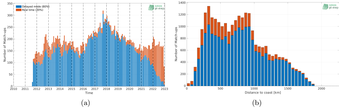
Figure 1: Number of match-ups between Argo and SMAP SSS L4 OI v2 - 7 Days (ESR) SSS as a function of time (a) and as function of the distance to coast (b) over the Gulf Stream Pi-MEP region and for the full satellite product period.
