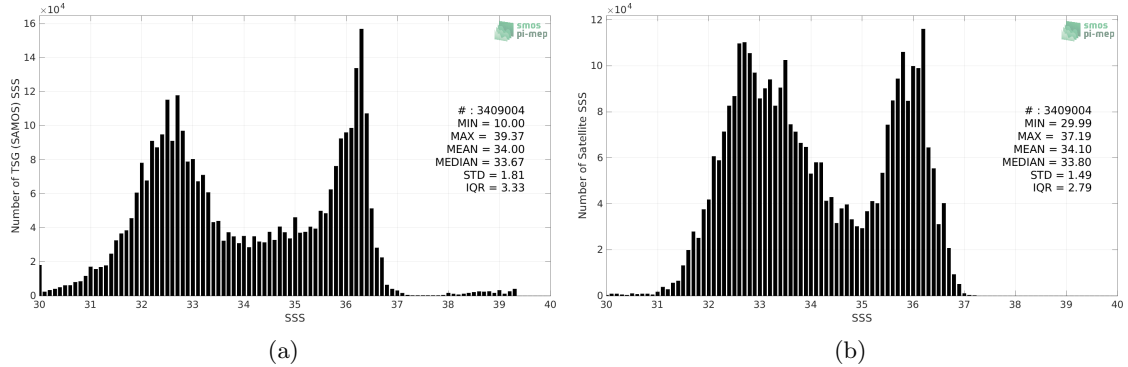
Figure 2: Histograms of SSS from TSG (SAMOS) (a) and SMAP SSS L4 OI v2 - Monthly (IPRC) (b) considering all match-up pairs per bins of 0.1 over the Gulf Stream Pi-MEP region and for the full satellite product period.
