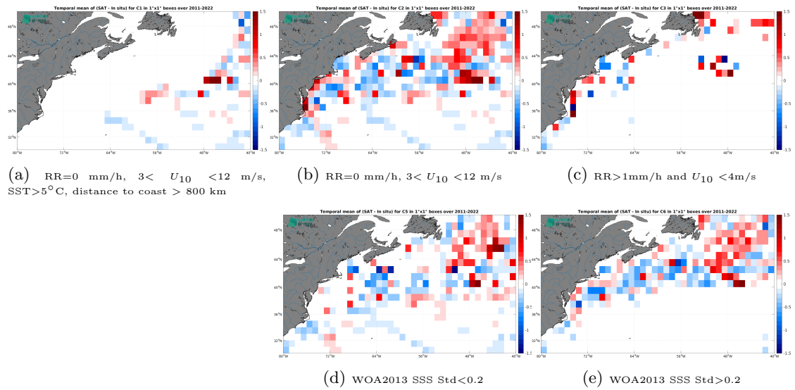
Figure 12: Temporal mean gridded over spatial boxes of size 1^\circ \times 1^\circ of \Delta SSS (SMAP SSS L4 OI v2 - Monthly (IPRC) - TSG (LEGOS-DM)) for 5 different subdatasets corresponding to:RR=0 mm/h, 3 < U_{10} < 12 m/s, SST >5^\circ C, distance to coast > 800 km (a), RR=0 mm/h, 3 < U_{10} < 12 m/s (b), RR >1 mm/h and U_{10} < 4 m/s (c), WOA2013 SSS Std <0.2 (d), WOA2013 SSS Std >0.2 (e).
