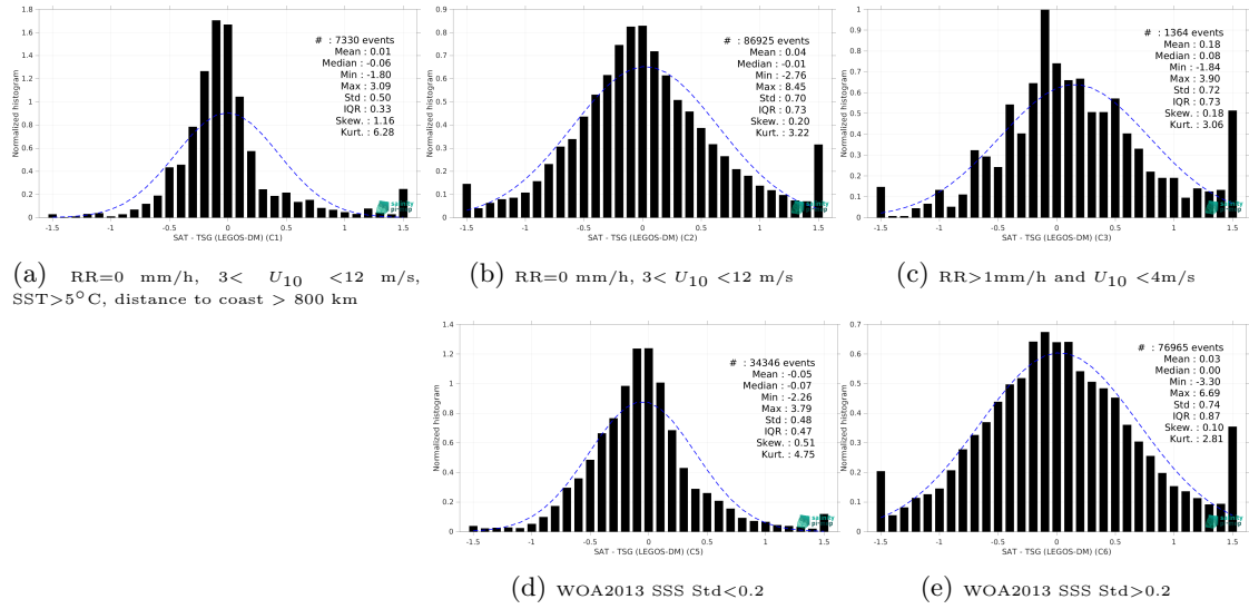
Figure 13: Normalized histogram of \Delta SSS (SMAP SSS L4 OI v2 - Monthly (IPRC) - TSG (LEGOS-DM)) for 5 different subdatasets corresponding to: RR=0 mm/h, 3 < U_{10} < 12 m/s, SST > 5°C, distance to coast > 800 km (a), RR=0 mm/h, 3 < U_{10} < 12 m/s (b), RR > 1mm/h and U_{10} < 4 m/s (c), WOA2013 SSS Std < 0.2 (d), WOA2013 SSS Std > 0.2 (e).
