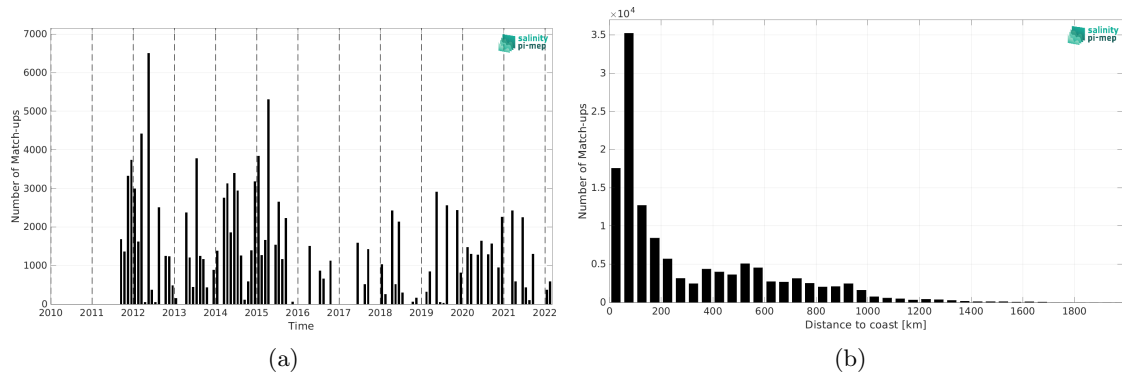
Figure 1: Number of match-ups between TSG (LEGOS-DM) and SMAP SSS L4 OI v2 - Monthly (IPRC) SSS as a function of time (a) and as function of the distance to coast (b) over the Gulf Stream Pi-MEP region and for the full satellite product period.
