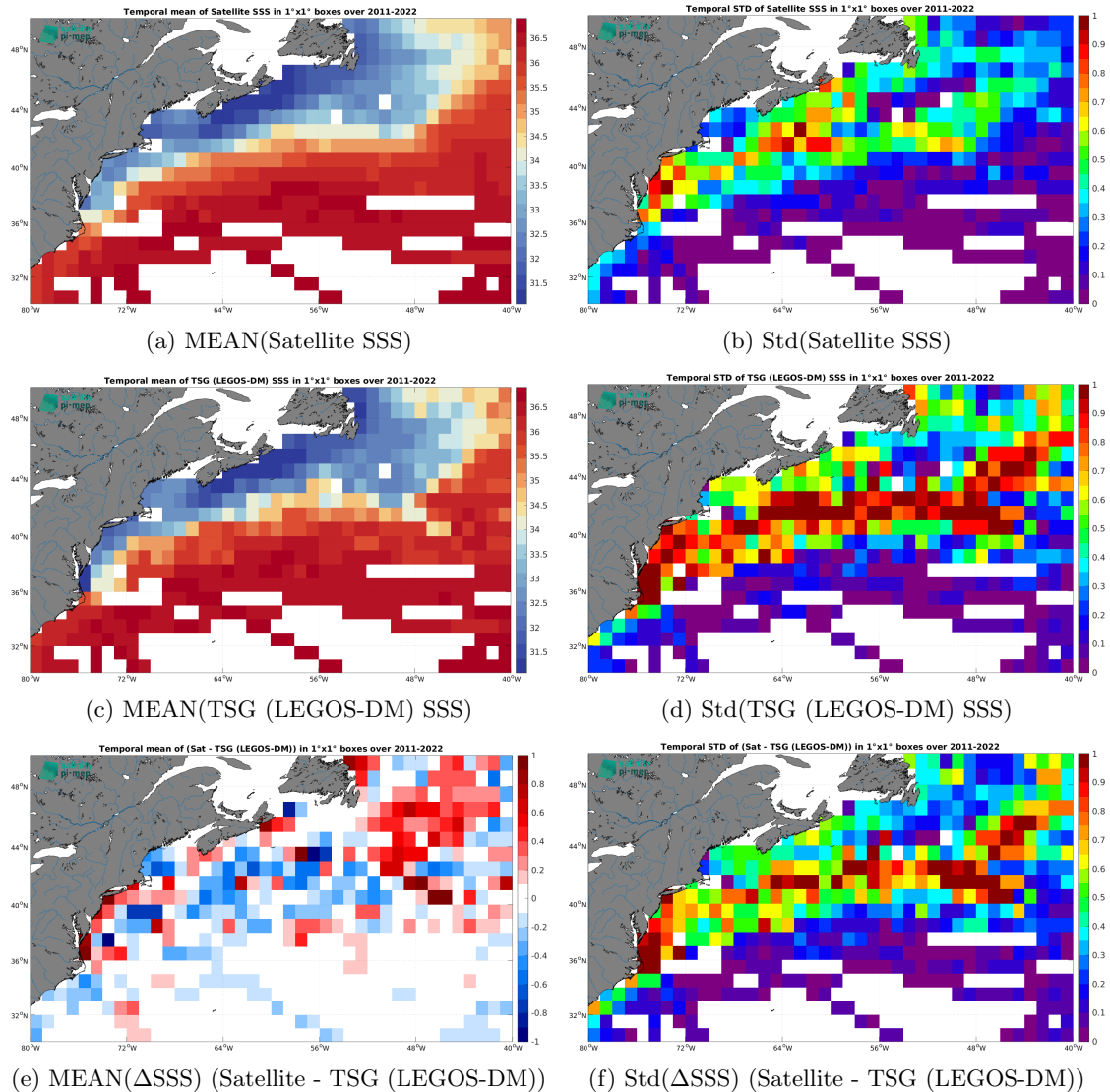
Figure 6: Temporal mean (left) and Std (right) of SSS from SMAP SSS L4 OI v2 - Monthly (IPRC) (top), TSG (LEGOS-DM) (middle), and of \Delta SSS (Satellite - TSG (LEGOS-DM)). Only match-up pairs are used to generate these maps.
