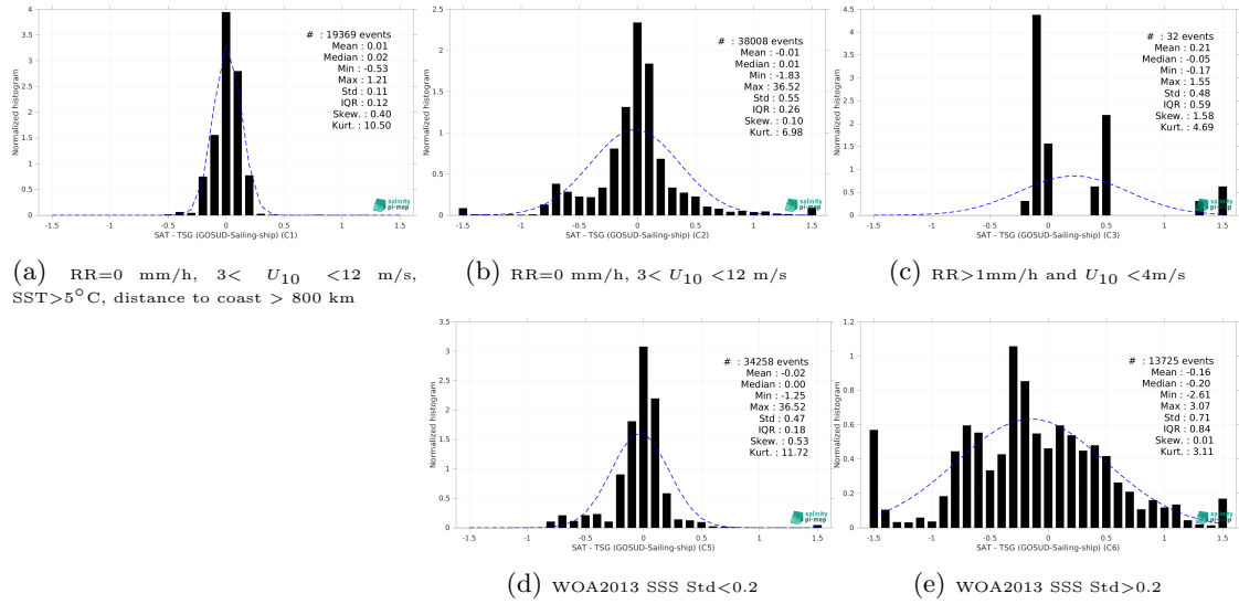
Figure 13: Normalized histogram of \Delta SSS (SMAP SSS L4 OI v2 - Monthly (IPRC) - TSG (GOSUD-Sailing-ship)) for 5 different subdatasets corresponding to: RR=0 mm/h, 3 < U_{10} < 12 m/s, SST>5°C, distance to coast > 800 km (a), RR=0 mm/h, 3 < U_{10} < 12 m/s (b), RR>1mm/h and U_{10} < 4 m/s (c), WOA2013 SSS Std<0.2 (d), WOA2013 SSS Std>0.2 (e).
