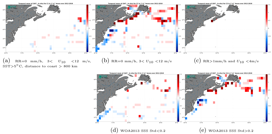
Figure 12: Temporal mean gridded over spatial boxes of size 1^\circ \times 1^\circ of \Delta SSS (SMAP SSS L4 OI v2 - Monthly (IPRC) - TSG (GOSUD-Sailing-ship)) for 5 different subdatasets corresponding to: RR=0 mm/h, 3 < U_{10} < 12 m/s, SST > 5°C, distance to coast > 800 km (a), RR=0 mm/h, 3 < U_{10} < 12 m/s (b), RR > 1mm/h and U_{10} < 4 m/s (c), WOA2013 SSS Std < 0.2 (d), WOA2013 SSS Std > 0.2 (e).
