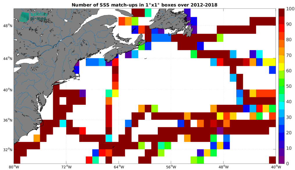
Figure 4: Number of SSS match-ups between TSG (GOSUD-Sailing-ship) SSS and the SMAP SSS L4 OI v2 - Monthly (IPRC) SSS product for the Gulf Stream Pi-MEP region over 1^\circ \times 1^\circ boxes and for the full satellite product period.
