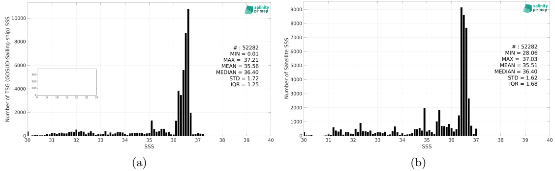
Figure 2: Histograms of SSS from TSG (GOSUD-Sailing-ship) (a) and SMAP SSS L4 OI v2 - Monthly (IPRC) (b) considering all match-up pairs per bins of 0.1 over the Gulf Stream Pi-MEP region and for the full satellite product period.
