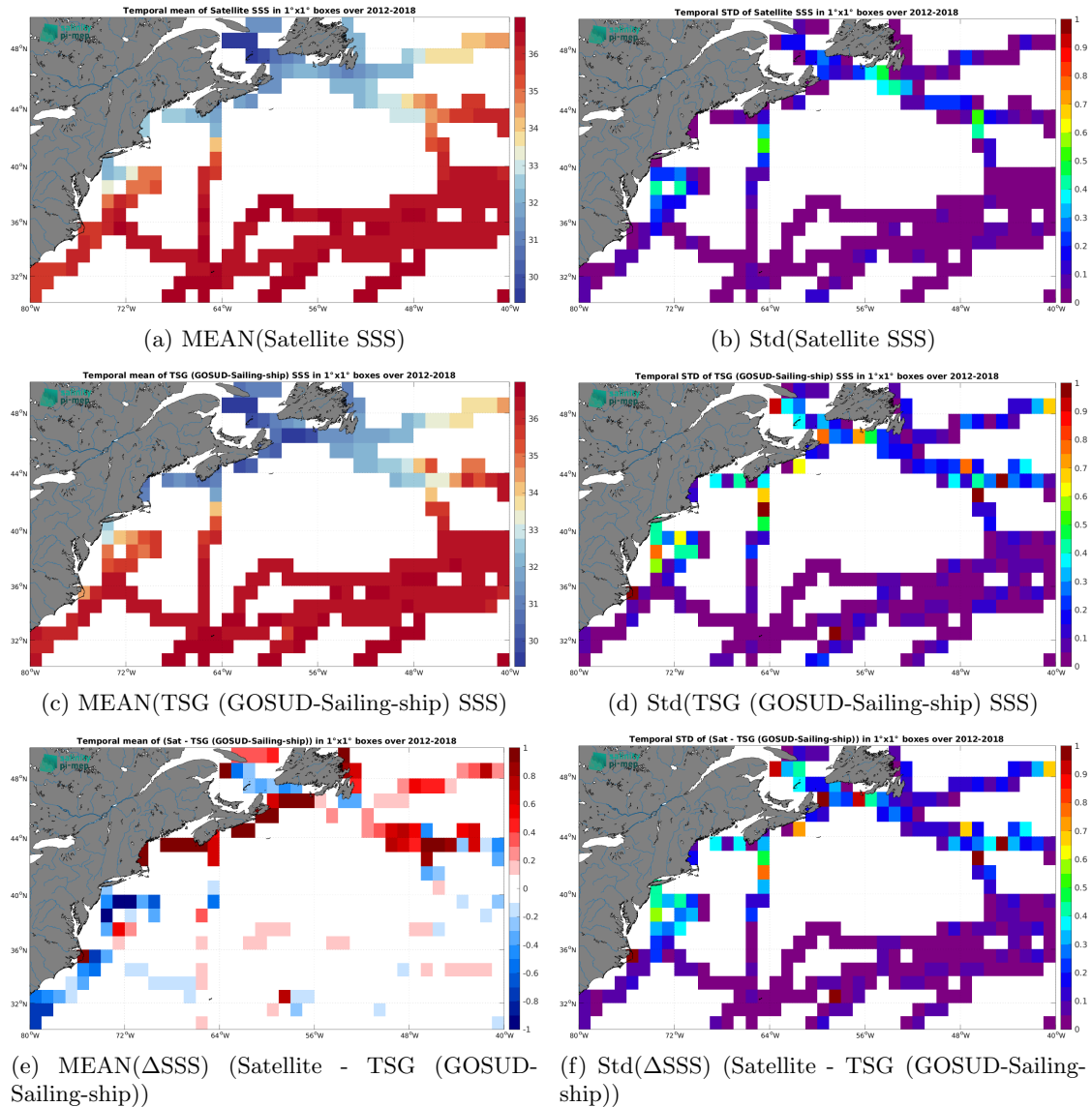
Figure 6: Temporal mean (left) and Std (right) of SSS from SMAP SSS L4 OI v2 - Monthly (IPRC) (top), TSG (GOSUD-Sailing-ship) (middle), and of \Delta SSS (Satellite - TSG (GOSUD-Sailing-ship)). Only match-up pairs are used to generate these maps.
