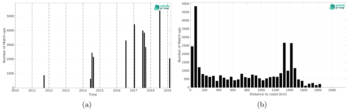
Figure 1: Number of match-ups between TSG (GOSUD-Research-vessel) and SMAP SSS L4 OI v2 - Monthly (IPRC) SSS as a function of time (a) and as function of the distance to coast (b) over the Gulf Stream Pi-MEP region and for the full satellite product period.
