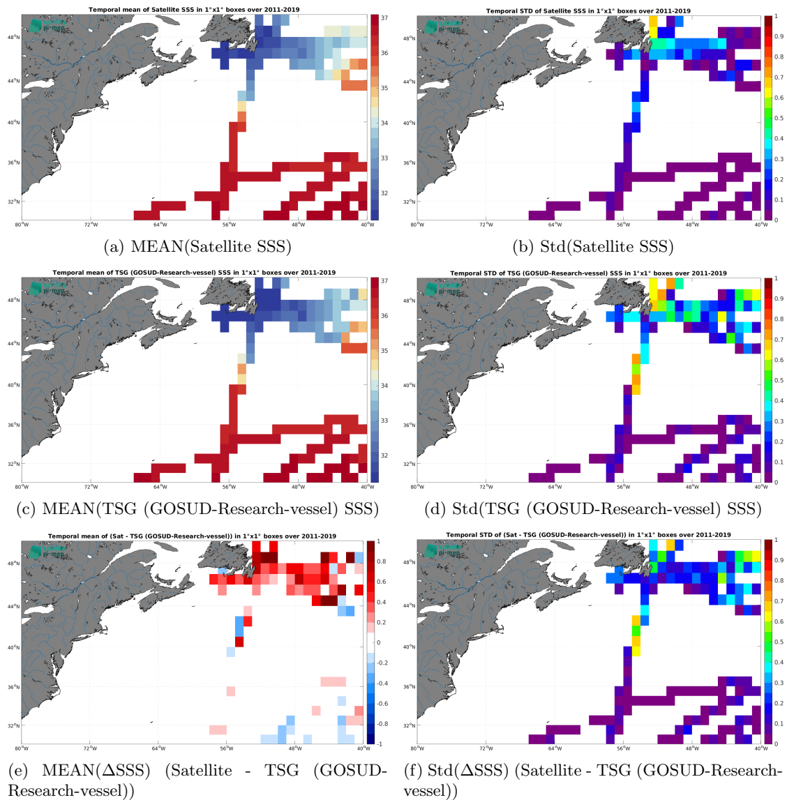
Figure 6: Temporal mean (left) and Std (right) of SSS from SMAP SSS L4 OI v2 - Monthly (IPRC) (top), TSG (GOSUD-Research-vessel) (middle), and of \Delta SSS (Satellite - TSG (GOSUD-Research-vessel)). Only match-up pairs are used to generate these maps.
