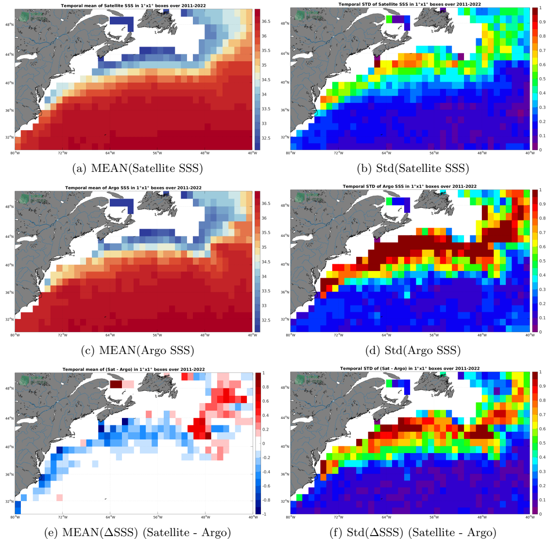
Figure 6: Temporal mean (left) and Std (right) of SSS from SMAP SSS L4 OI v2 - Monthly (IPRC) (top), Argo (middle), and of \Delta SSS (Satellite - Argo). Only match-up pairs are used to generate these maps.
