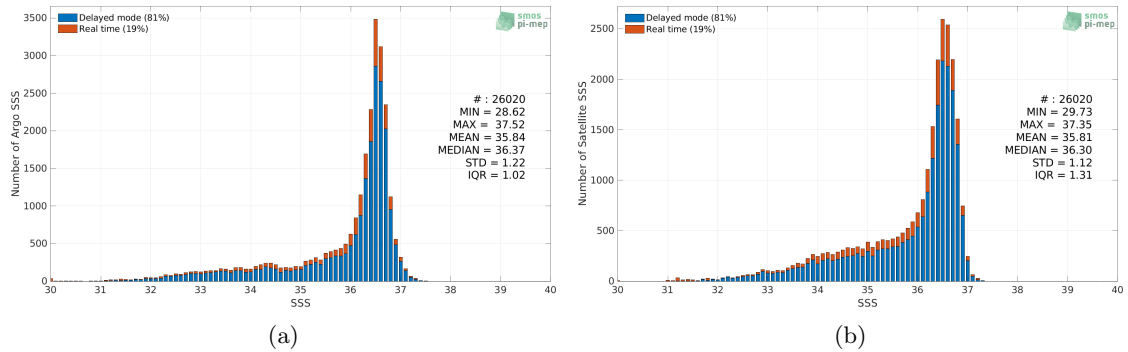
Figure 2: Histograms of SSS from Argo (a) and SMAP SSS L4 OI v2 - Monthly (IPRC) (b) considering all match-up pairs per bins of 0.1 over the Gulf Stream Pi-MEP region and for the full satellite product period.
