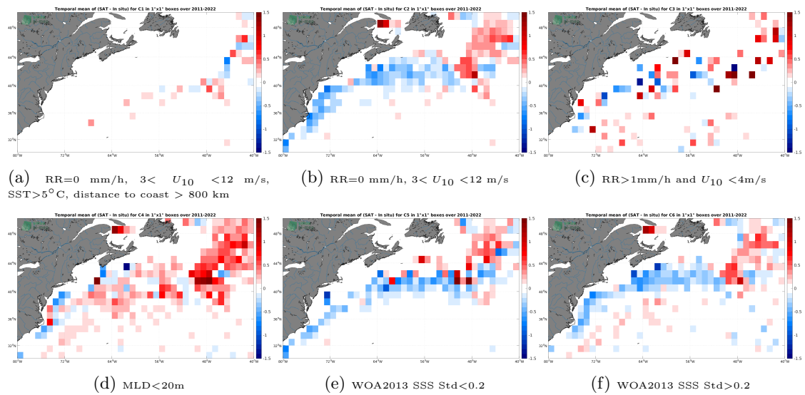
Figure 12: Temporal mean gridded over spatial boxes of size 1^\circ \times 1^\circ of \Delta SSS (SMAP SSS L4 OI v2 - Monthly (IPRC) - Argo) for 6 different subdatasets corresponding to:RR=0 mm/h, 3 < U_{10} < 12 m/s, SST > 5^\circ\text{C} , distance to coast > 800 km (a), RR=0 mm/h, 3 < U_{10} < 12 m/s (b), RR > 1 mm/h and U_{10} < 4 m/s (c),MLD < 20 m (d),WOA2013 SSS Std < 0.2 (e),WOA2013 SSS Std > 0.2 (f).
