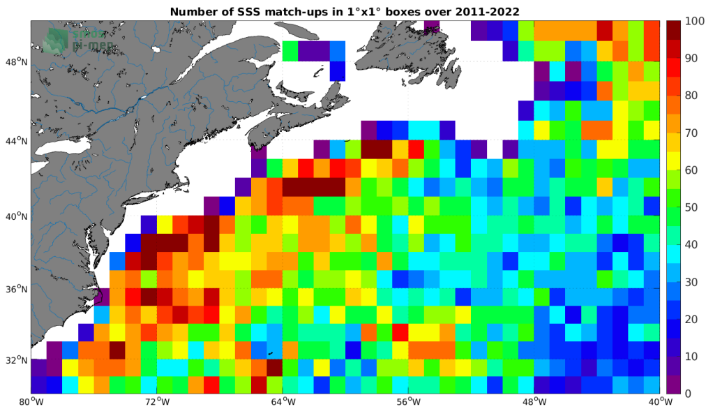
Figure 4: Number of SSS match-ups between Argo SSS and the SMAP SSS L4 OI v2 - Monthly (IPRC) SSS product for the Gulf Stream Pi-MEP region over 1^\circ \times 1^\circ boxes and for the full satellite product period.
