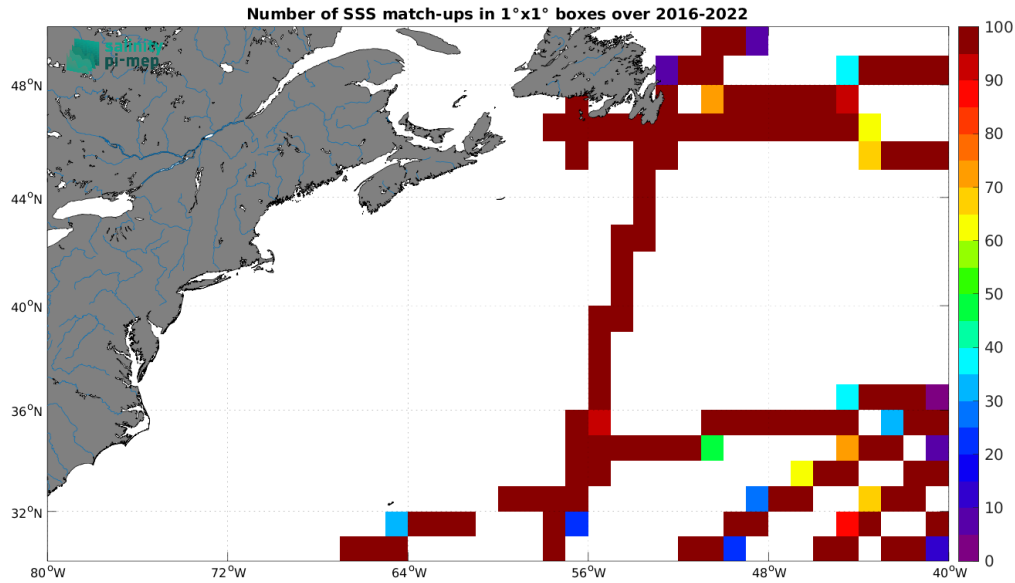
Figure 5: Number of SSS match-ups between TSG (GOSUD-Research-vessel) SSS and the SMAP SSS L3 v6 - 8-Day running (RSS) SSS product for the Gulf Stream Pi-MEP region over 1^\circ \times 1^\circ boxes and for the full satellite product period.
