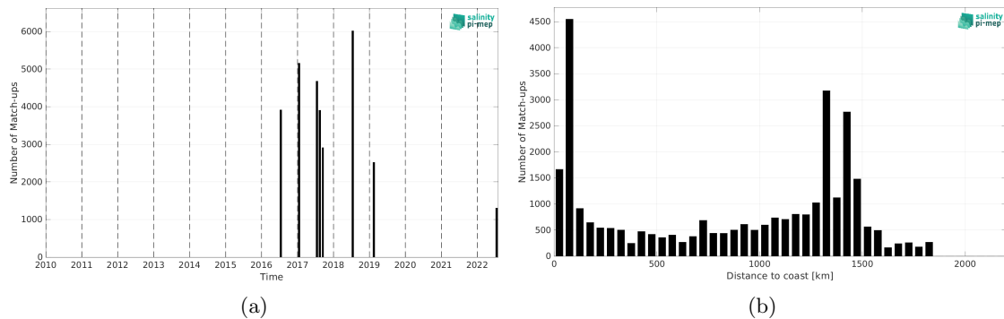
Figure 2: Number of match-ups between TSG (GOSUD-Research-vessel) and SMAP SSS L3 v6 - 8-Day running (RSS) SSS as a function of time (a) and as function of the distance to coast (b) over the Gulf Stream Pi-MEP region and for the full satellite product period.
