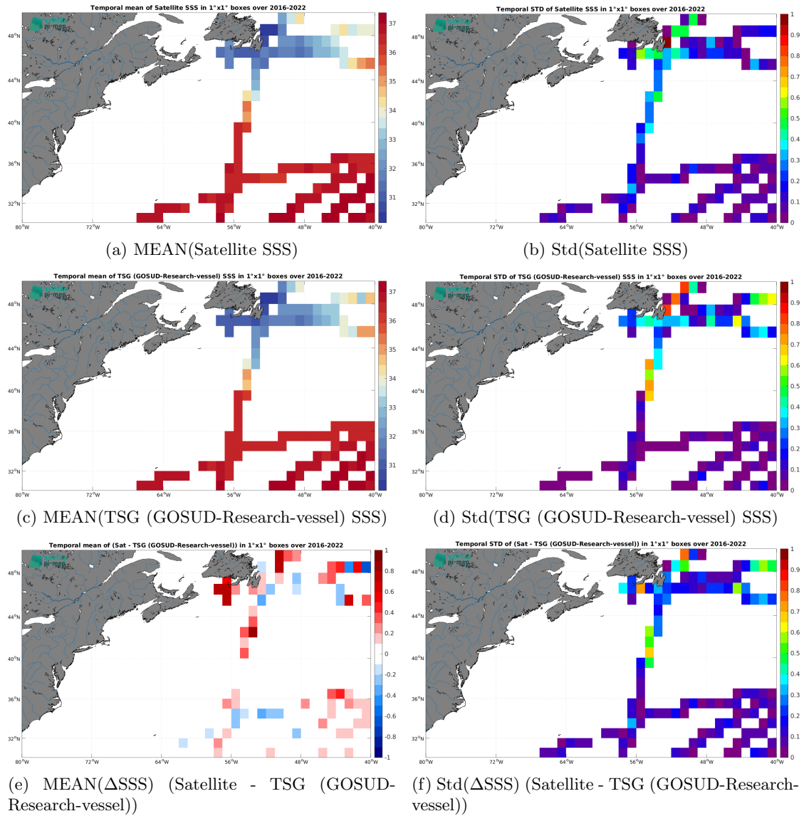
Figure 7: Temporal mean (left) and Std (right) of SSS from SMAP SSS L3 v6 - 8-Day running (RSS) (top), TSG (GOSUD-Research-vessel) (middle), and of \Delta SSS (Satellite - TSG (GOSUD-Research-vessel)). Only match-up pairs are used to generate these maps.
