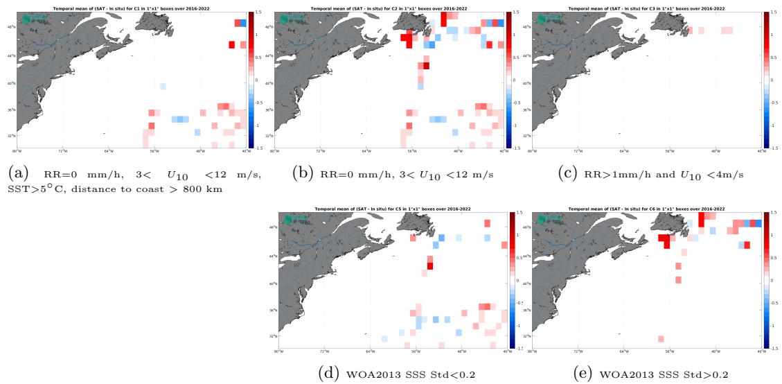
Figure 14: Temporal mean gridded over spatial boxes of size 1^\circ \times 1^\circ of \Delta SSS (SMAP SSS L3 v6 - 8-Day running (RSS) - TSG (GOSUD-Research-vessel)) for 5 different subdatasets corresponding to:RR=0 mm/h, 3 < U_{10} < 12 m/s, SST>5°C, distance to coast > 800 km (a), RR=0 mm/h, 3 < U_{10} < 12 m/s (b), RR>1mm/h and U_{10} < 4 m/s (c), WOA2013 SSS Std<0.2 (d), WOA2013 SSS Std>0.2 (e).
