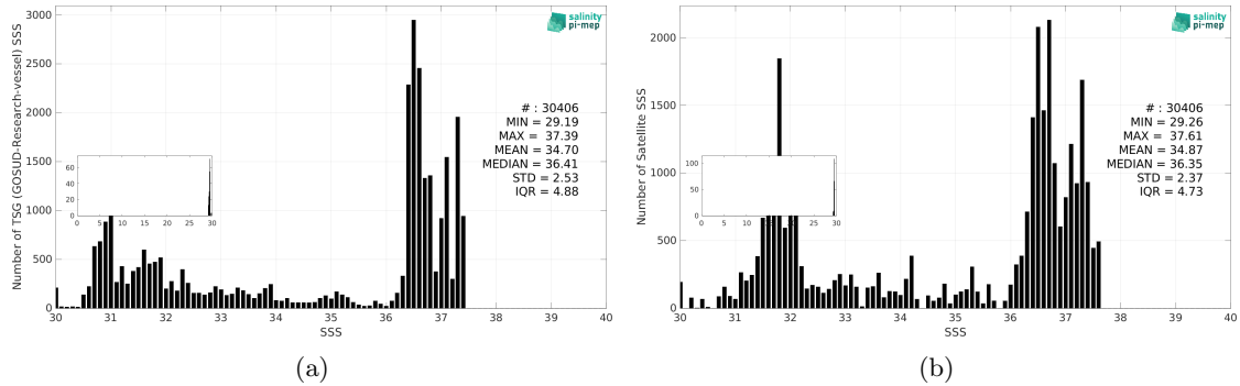
Figure 3: Histograms of SSS from TSG (GOSUD-Research-vessel) (a) and SMAP SSS L3 v6 - 8-Day running (RSS) (b) considering all match-up pairs per bins of 0.1 over the Gulf Stream Pi-MEP region and for the full satellite product period.
