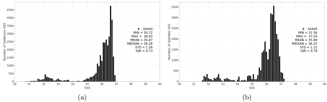
Figure 3: Histograms of SSS from Saildrone (a) and SMAP SSS L3 v6 - 8-Day running (RSS) (b) considering all match-up pairs per bins of 0.1 over the Gulf Stream Pi-MEP region and for the full satellite product period.
