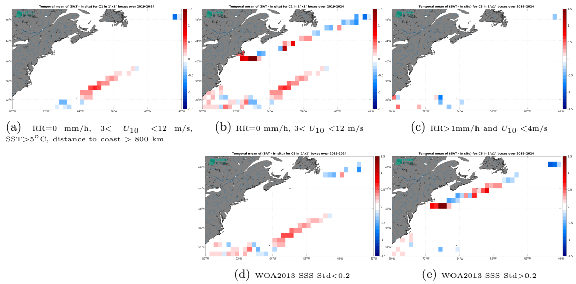
Figure 14: Temporal mean gridded over spatial boxes of size 1^\circ \times 1^\circ of \Delta SSS (SMAP SSS L3 v6 - 8-Day running (RSS) - Sairdrone) for 5 different subdatasets corresponding to: RR=0 mm/h, 3 < U_{10} < 12 m/s, SST > 5°C, distance to coast > 800 km (a), RR=0 mm/h, 3 < U_{10} < 12 m/s (b), RR > 1mm/h and U_{10} < 4 m/s (c), WOA2013 SSS Std < 0.2 (d), WOA2013 SSS Std > 0.2 (e).
