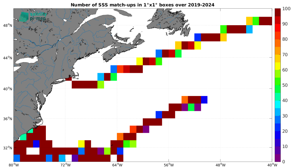
Figure 5: Number of SSS match-ups between Saildrone SSS and the SMAP SSS L3 v6 - 8-Day running (RSS) SSS product for the Gulf Stream Pi-MEP region over 1^\circ \times 1^\circ boxes and for the full satellite product period.
