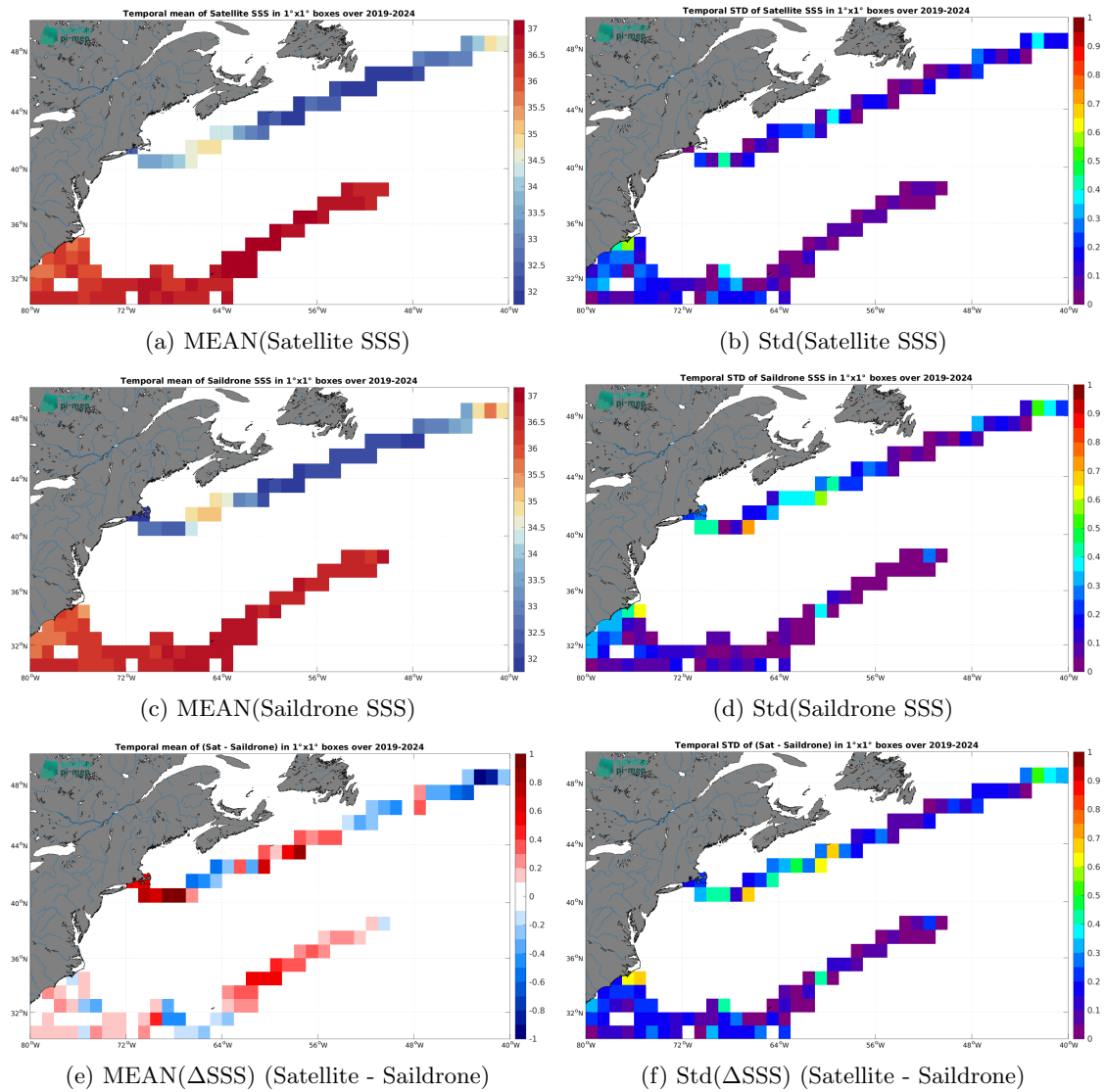
Figure 7: Temporal mean (left) and Std (right) of SSS from SMAP SSS L3 v6 - 8-Day running (RSS) (top), Saildrone (middle), and of \Delta SSS (Satellite - Saildrone). Only match-up pairs are used to generate these maps.
