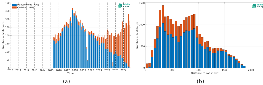
Figure 2: Number of match-ups between Argo and SMAP SSS L3 v6 - 8-Day running (RSS) SSS as a function of time (a) and as function of the distance to coast (b) over the Gulf Stream Pi-MEP region and for the full satellite product period.
