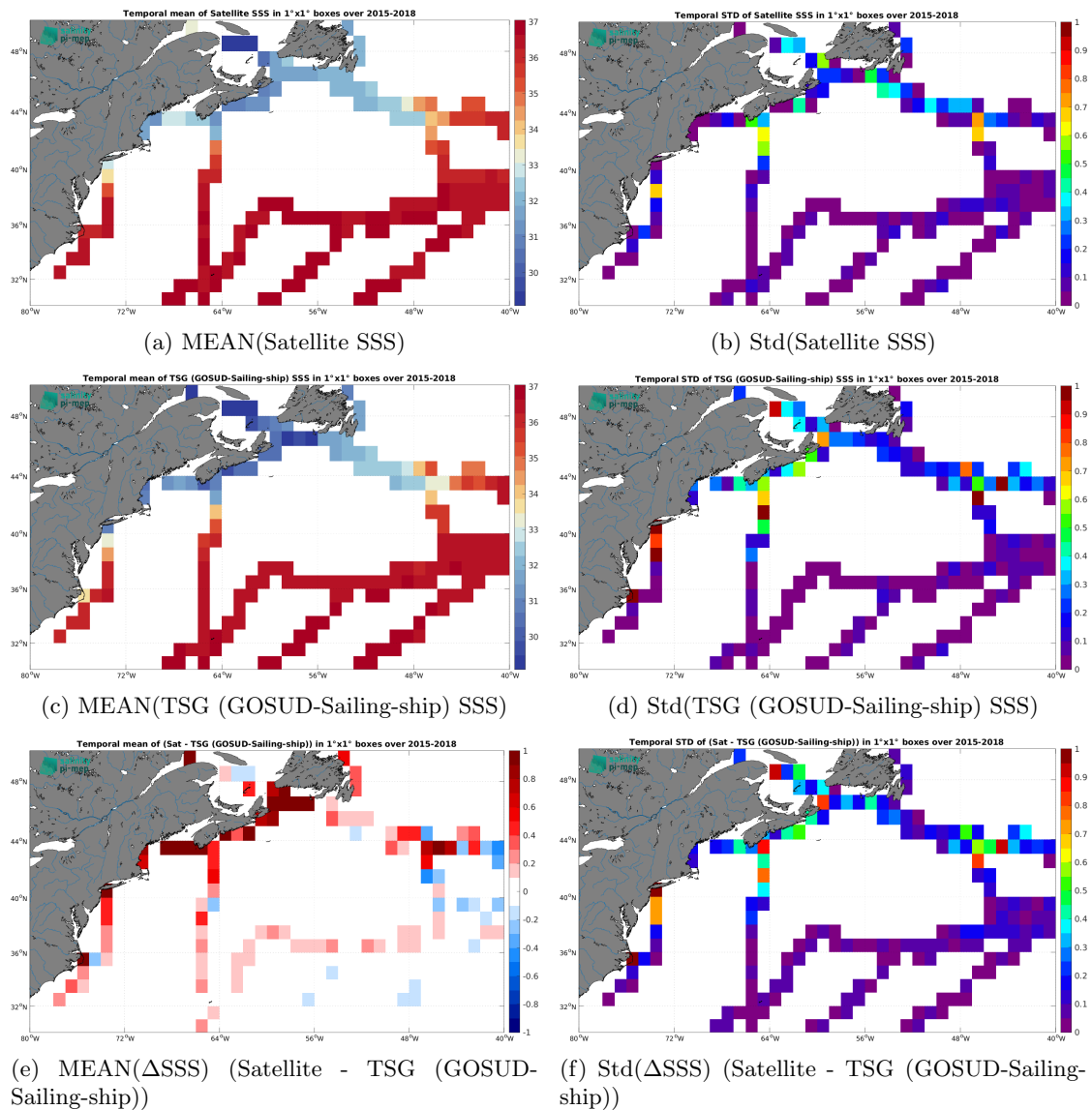
Figure 7: Temporal mean (left) and Std (right) of SSS from SMAP SSS L3 v6 - Monthly (RSS) (top), TSG (GOSUD-Sailing-ship) (middle), and of \Delta SSS (Satellite - TSG (GOSUD-Sailing-ship)). Only match-up pairs are used to generate these maps.
