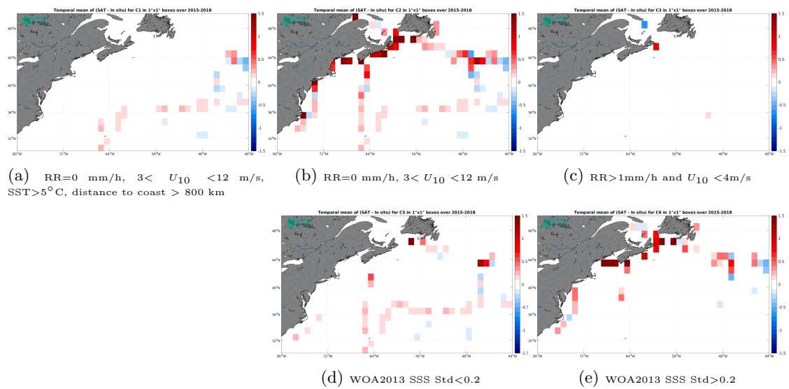
Figure 14: Temporal mean gridded over spatial boxes of size 1^\circ \times 1^\circ of \Delta SSS (SMAP SSS L3 v6 - Monthly (RSS) - TSG (GOSUD-Sailing-ship)) for 5 different subdatasets corresponding to:RR=0 mm/h, 3 < U_{10} < 12 m/s, SST >5^\circ C, distance to coast > 800 km (a), RR=0 mm/h, 3 < U_{10} < 12 m/s (b), RR >1 mm/h and U_{10} < 4 m/s (c), WOA2013 SSS Std <0.2 (d), WOA2013 SSS Std >0.2 (e).
