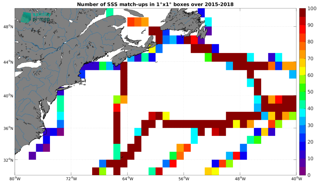
Figure 5: Number of SSS match-ups between TSG (GOSUD-Sailing-ship) SSS and the SMAP SSS L3 v6 - Monthly (RSS) SSS product for the Gulf Stream Pi-MEP region over 1^\circ \times 1^\circ boxes and for the full satellite product period.
