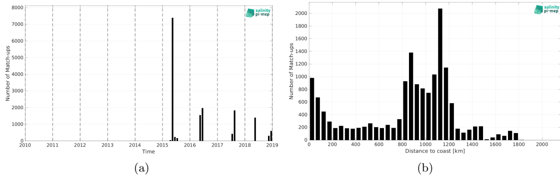
Figure 2: Number of match-ups between TSG (GOSUD-Sailing-ship) and SMAP SSS L3 v6 - Monthly (RSS) SSS as a function of time (a) and as function of the distance to coast (b) over the Gulf Stream Pi-MEP region and for the full satellite product period.
