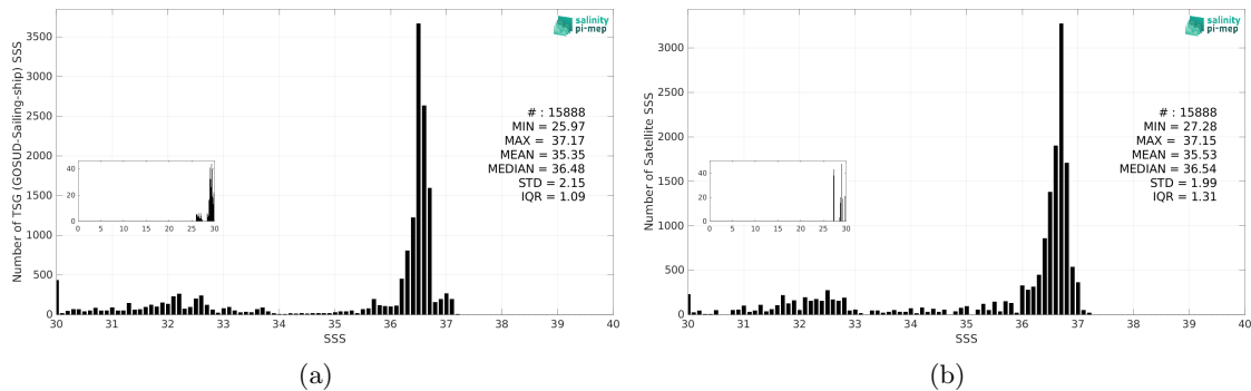
Figure 3: Histograms of SSS from TSG (GOSUD-Sailing-ship) (a) and SMAP SSS L3 v6 - Monthly (RSS) (b) considering all match-up pairs per bins of 0.1 over the Gulf Stream Pi-MEP region and for the full satellite product period.
