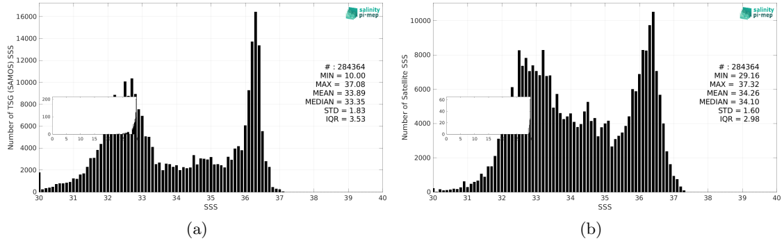
Figure 3: Histograms of SSS from TSG (SAMOS) (a) and SMAP SSS L3 v5.3 - 8-Day running (RSS) (b) considering all match-up pairs per bins of 0.1 over the Gulf Stream Pi-MEP region and for the full satellite product period.
