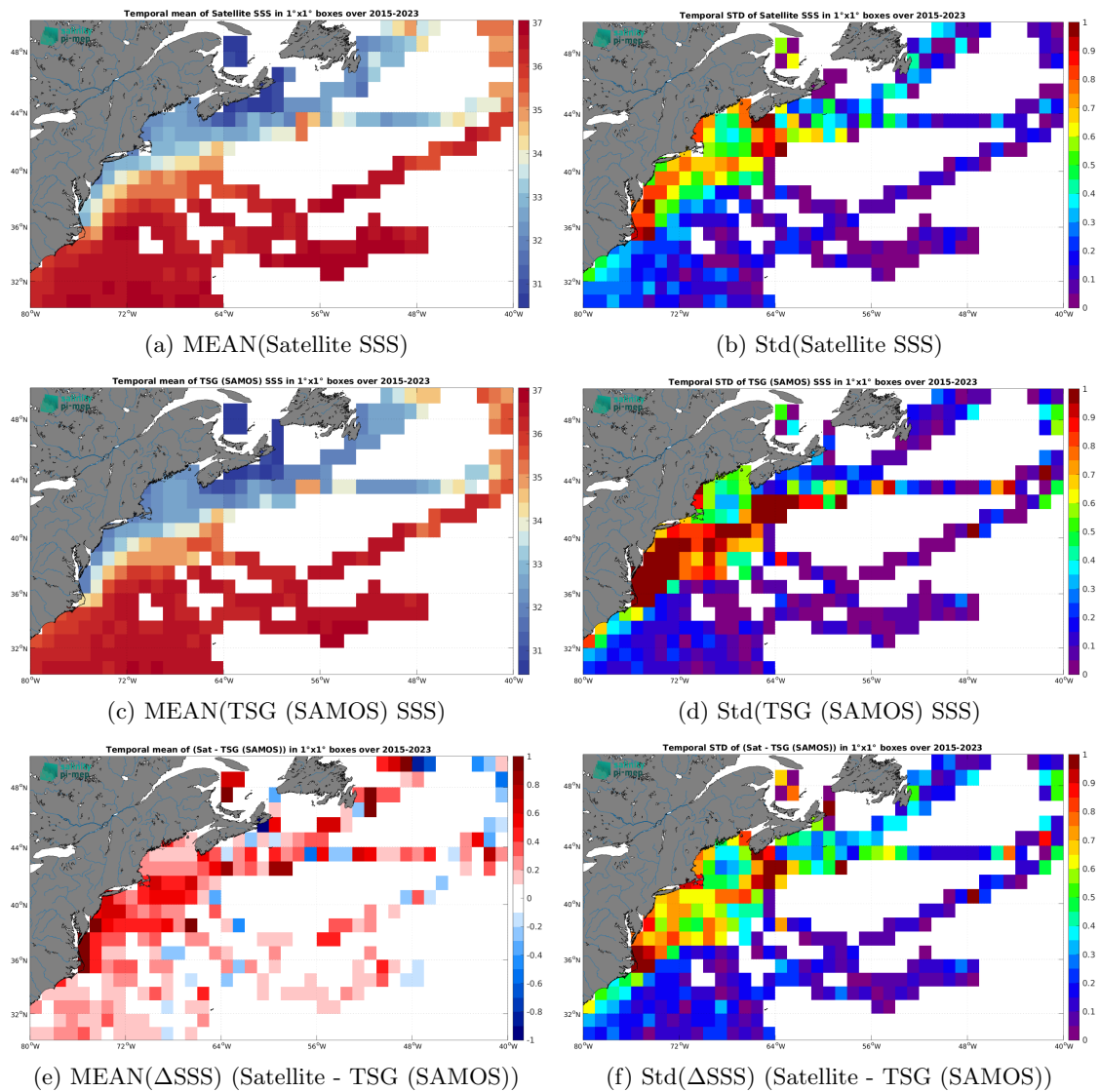
Figure 7: Temporal mean (left) and Std (right) of SSS from SMAP SSS L3 v5.3 - 8-Day running (RSS) (top), TSG (SAMOS) (middle), and of \Delta SSS (Satellite - TSG (SAMOS)). Only match-up pairs are used to generate these maps.
