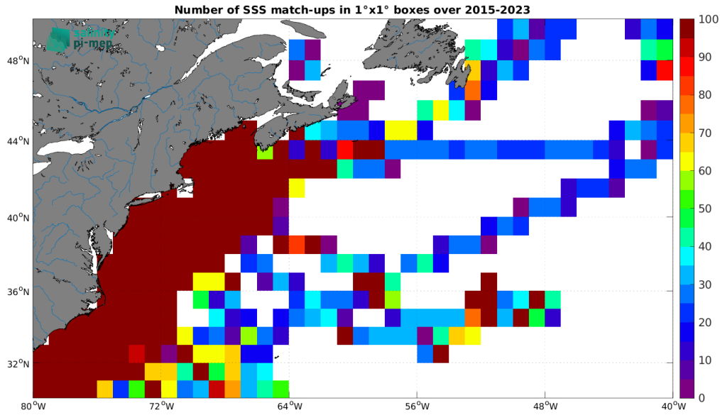
Figure 5: Number of SSS match-ups between TSG (SAMOS) SSS and the SMAP SSS L3 v5.3 - 8-Day running (RSS) SSS product for the Gulf Stream Pi-MEP region over 1^\circ \times 1^\circ boxes and for the full satellite product period.
