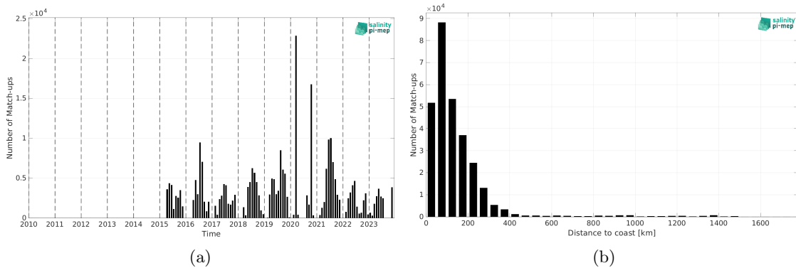
Figure 2: Number of match-ups between TSG (SAMOS) and SMAP SSS L3 v5.3 - 8-Day running (RSS) SSS as a function of time (a) and as function of the distance to coast (b) over the Gulf Stream Pi-MEP region and for the full satellite product period.
