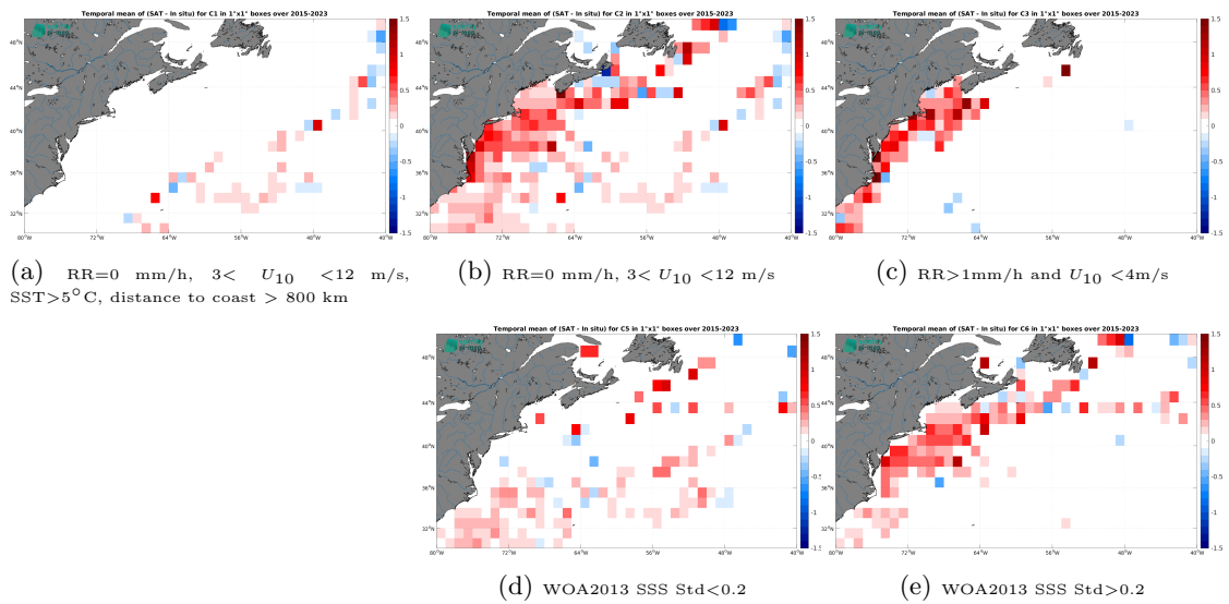
Figure 14: Temporal mean gridded over spatial boxes of size 1^\circ \times 1^\circ of \Delta SSS (SMAP SSS L3 v5.3 - 8-Day running (RSS) - TSG (SAMOS)) for 5 different subdatasets corresponding to:RR=0 mm/h, 3 < U_{10} < 12 m/s, SST > 5^\circ C , distance to coast > 800 km (a), RR=0 mm/h, 3 < U_{10} < 12 m/s (b), RR>1mm/h and U_{10} < 4 m/s (c), WOA2013 SSS Std<0.2 (d), WOA2013 SSS Std>0.2 (e).
