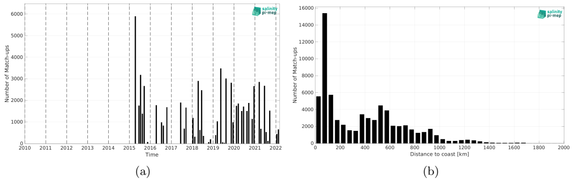
Figure 2: Number of match-ups between TSG (LEGOS-DM) and SMAP SSS L3 v5.3 - 8-Day running (RSS) SSS as a function of time (a) and as function of the distance to coast (b) over the Gulf Stream Pi-MEP region and for the full satellite product period.
