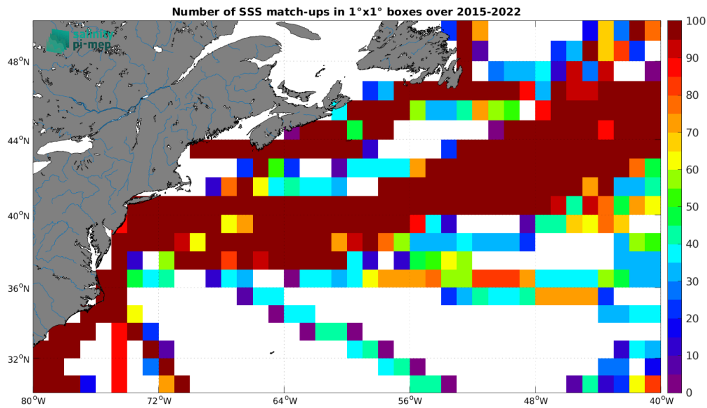
Figure 5: Number of SSS match-ups between TSG (LEGOS-DM) SSS and the SMAP SSS L3 v5.3 - 8-Day running (RSS) SSS product for the Gulf Stream Pi-MEP region over 1^\circ \times 1^\circ boxes and for the full satellite product period.
