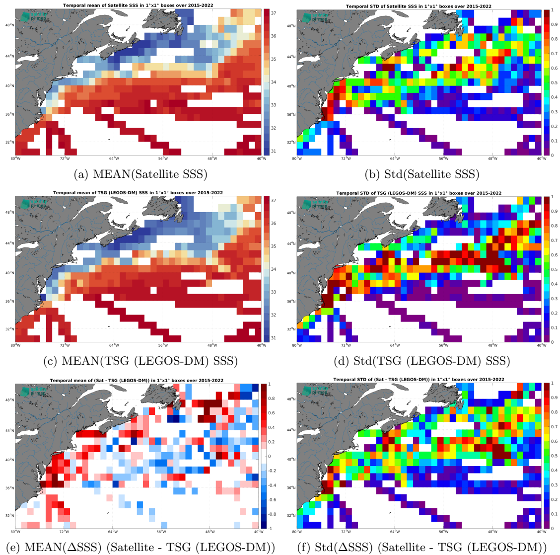
Figure 7: Temporal mean (left) and Std (right) of SSS from SMAP SSS L3 v5.3 - 8-Day running (RSS) (top), TSG (LEGOS-DM) (middle), and of \Delta SSS (Satellite - TSG (LEGOS-DM)). Only match-up pairs are used to generate these maps.
