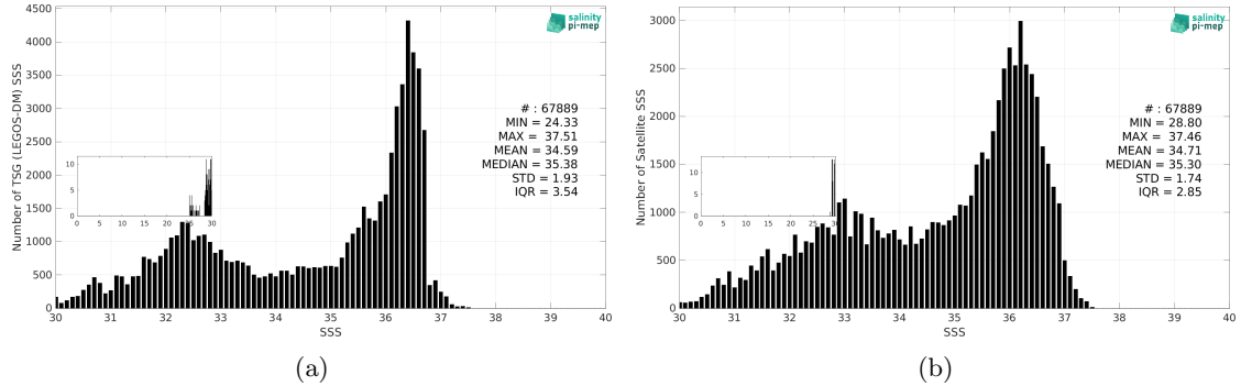
Figure 3: Histograms of SSS from TSG (LEGOS-DM) (a) and SMAP SSS L3 v5.3 - 8-Day running (RSS) (b) considering all match-up pairs per bins of 0.1 over the Gulf Stream Pi-MEP region and for the full satellite product period.
