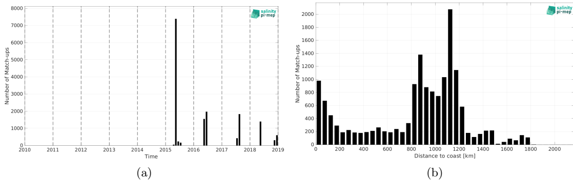
Figure 2: Number of match-ups between TSG (GOSUD-Sailing-ship) and SMAP SSS L3 v5.3 - 8-Day running (RSS) SSS as a function of time (a) and as function of the distance to coast (b) over the Gulf Stream Pi-MEP region and for the full satellite product period.
