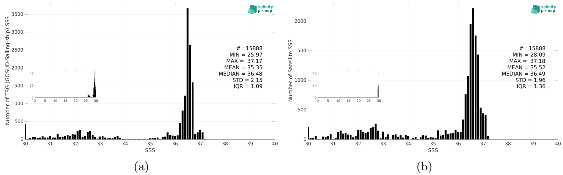
Figure 3: Histograms of SSS from TSG (GOSUD-Sailing-ship) (a) and SMAP SSS L3 v5.3 - 8-Day running (RSS) (b) considering all match-up pairs per bins of 0.1 over the Gulf Stream Pi-MEP region and for the full satellite product period.
