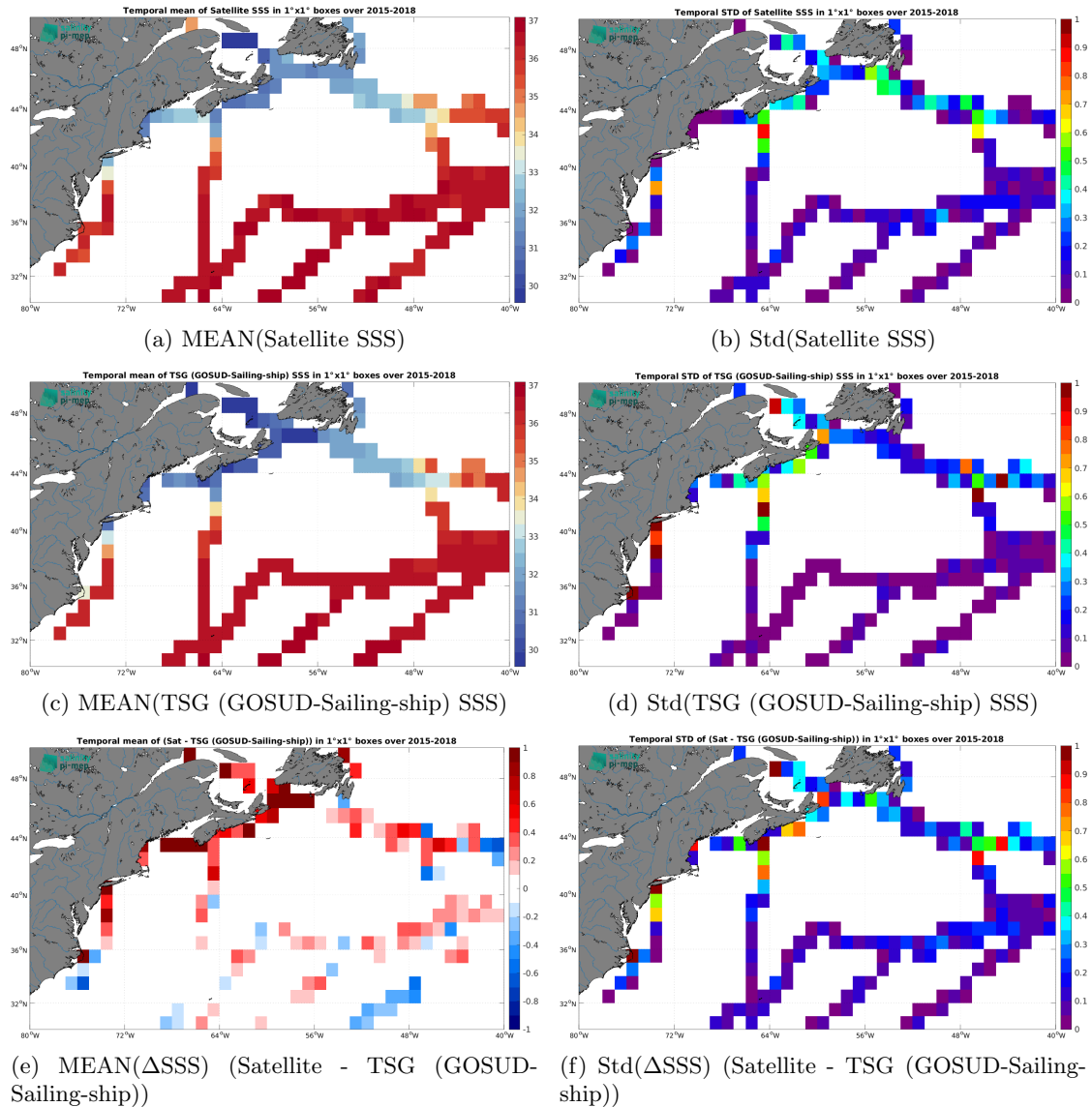
Figure 7: Temporal mean (left) and Std (right) of SSS from SMAP SSS L3 v5.3 - 8-Day running (RSS) (top), TSG (GOSUD-Sailing-ship) (middle), and of \Delta SSS (Satellite - TSG (GOSUD-Sailing-ship)). Only match-up pairs are used to generate these maps.
